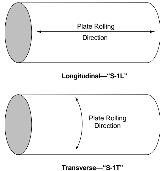
Figure A-1—Plate Rolling Direction Orientation
