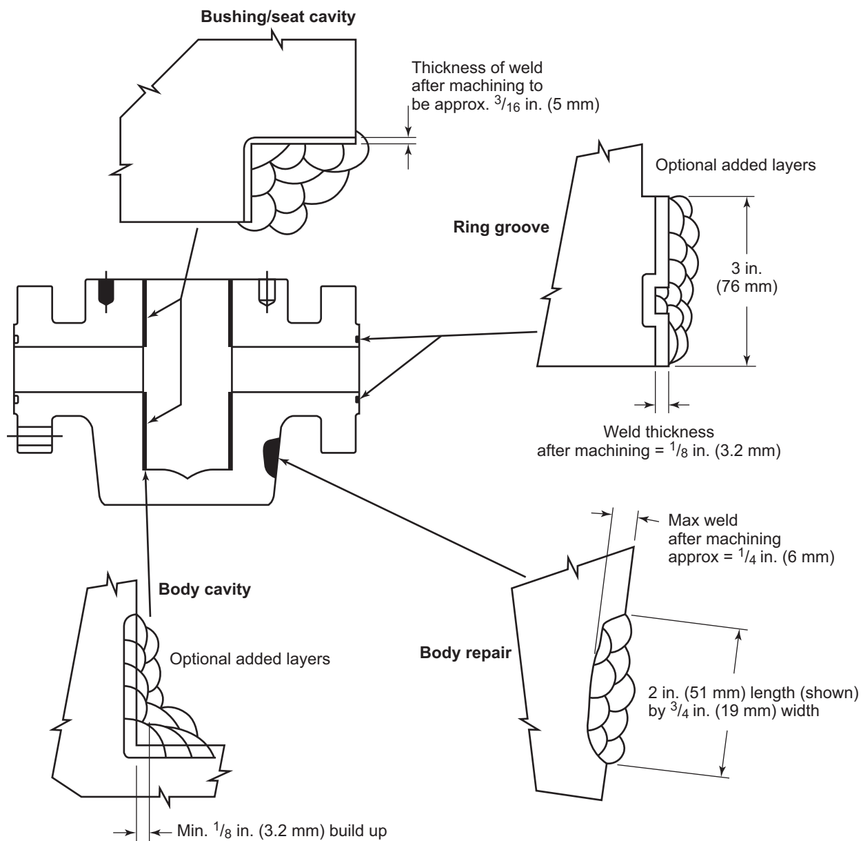
Figure C.7—Bushing/Seat Cavity
