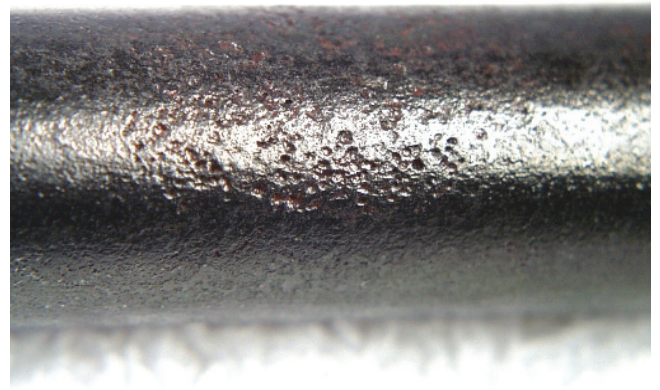
Pitting
