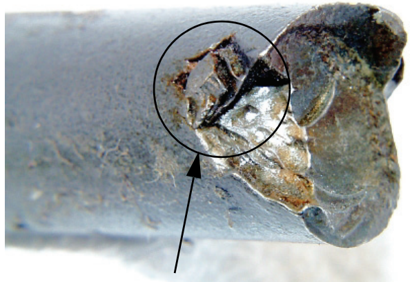
Rolled-in Scale
