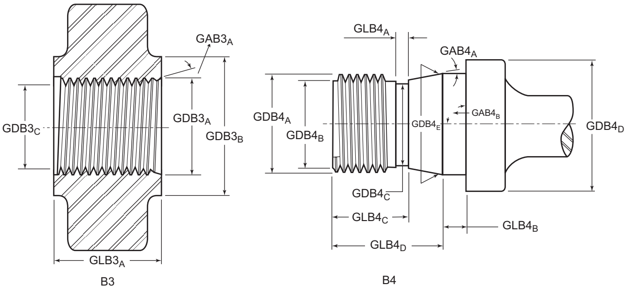
Figure I.4—Box-cone Gauges (For Gauging Box Connections)
