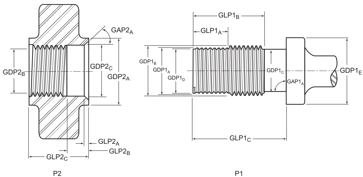
Figure I.6—Go Pin-thread Gauges (For Gauging Polished Rod Pin Connections)
