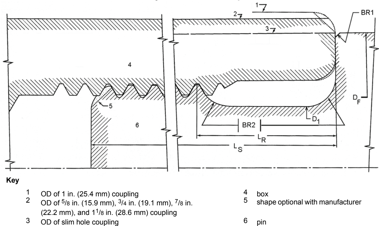
Figure A.3—Sucker Rod Connection
