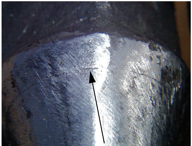
Forging Overfill
