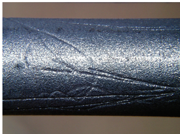
Surface Shearing From Foreign Objects Impressed During Hot Rolling Operation
