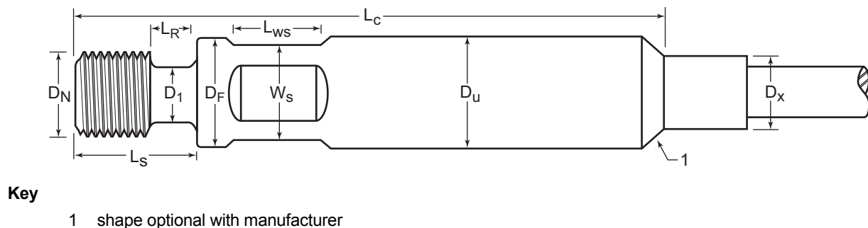
Figure D.1—General Dimensions for FRP Sucker Rod Pin Ends
