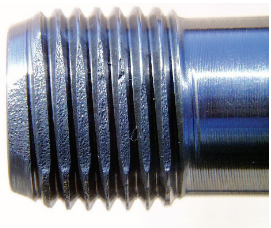
Thread Underfill
