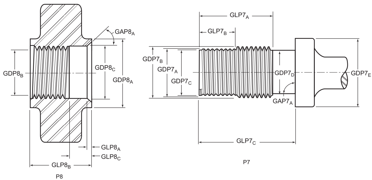
Figure I.1—Go Pin-thread Gauges (For Gauging Sucker Rod Pin Connections)
