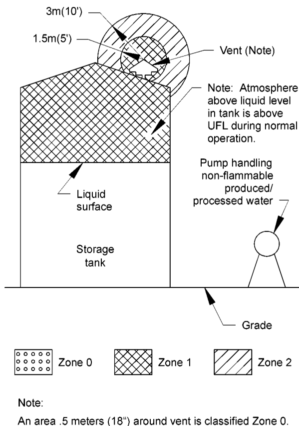
Figure 50—Flammable Gas-Blanketed and Produced Water-Handling Equipment in a Nonenclosed Adequately Ventilated Area (See Sections 10.8 and 10.12.4)
