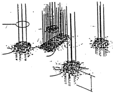
Figure 15—Components of an Independent Template Foundation System
