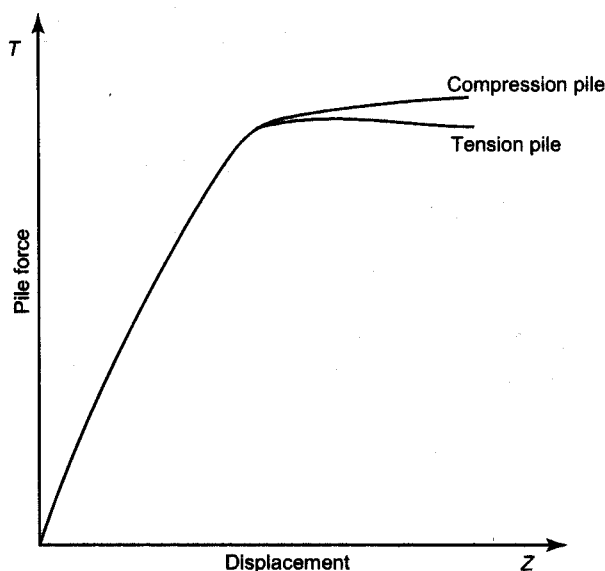
Figure D.1—Relative Residual Strength After Pile Overload
