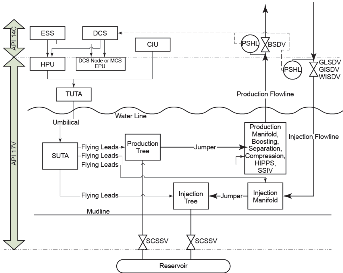
Figure 1—API RP 17V Scope
