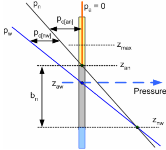
Figure 2.14—Capillary pressure distribution in the presence of LNAPL
