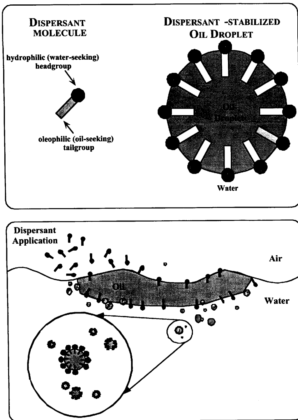
Figure 14. The mechanism of chemical dispersion.
