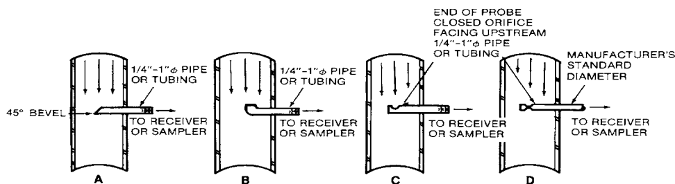
FIG. 17 Probe Designs
