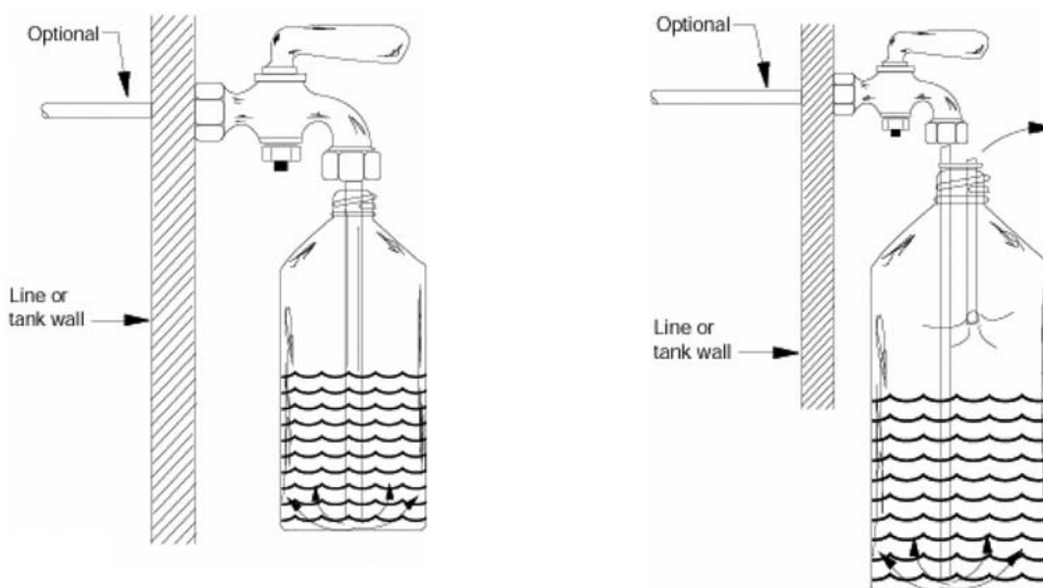
FIG. 16 Tank Sample Taps
