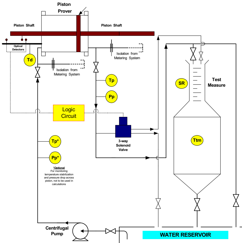
Figure 3C—Schematic Drawing of a Typical Layout for a Waterdraw Calibration of a Displacement Prover with Equal Size Diameter Shafts on Both Sides of a Captive Displacer and External Detectors using Top-filling Test Measures
