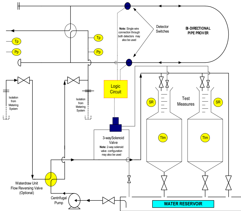
Figure 2B—Schematic Drawing of a Typical Layout for a Waterdraw Calibration of a Displacement Type Bi-directional Prover with a Free Sphere Displacer using Top-filling Test Measures
