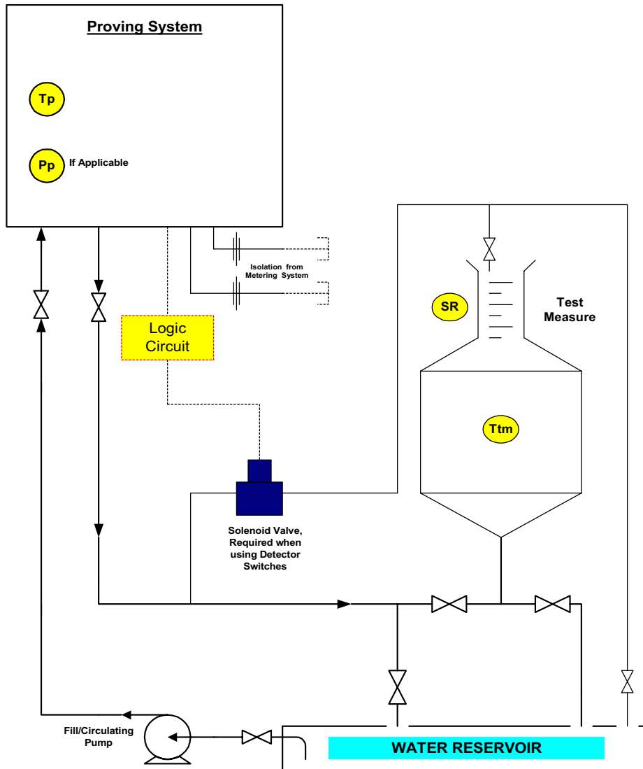
Figure 5—Alternate Method—Schematic Drawing of a Typical Layout for a Waterdraw Calibration of a Proving System using Bottom-filling Test Measures
