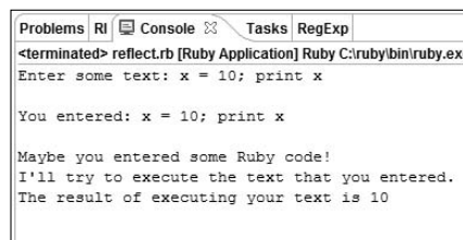
Figure 1-1: A run of the code in Listing 1-1.
