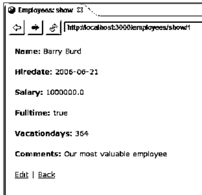
Figure 3-24: The Show page for one employee.
