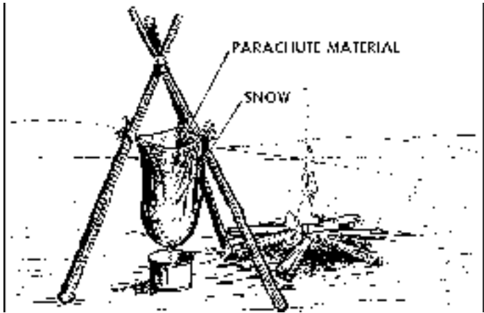
Figure VII-3. Water Generator
