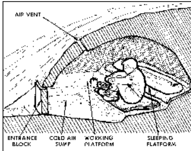
Figure VI-7. Snow Cave
