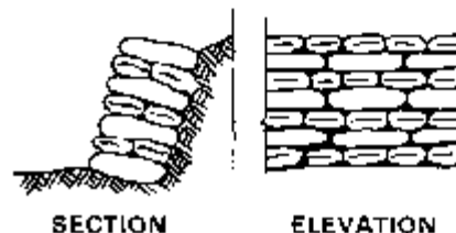
Stretchers and headers
