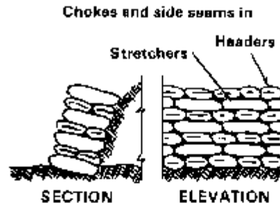
Retaining wall revetment
