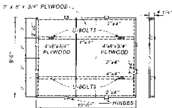
FLOOR DETAIL 1 NEEDED
