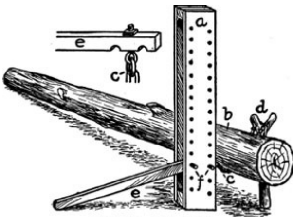
FIGURE 4—LOG JACK
