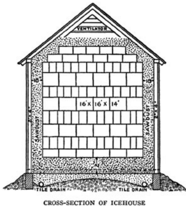
CROSS-SECTION OF ICEHOUSE
