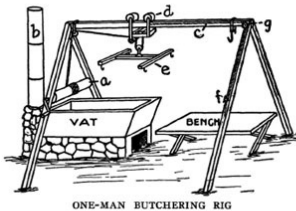
ONE-MAN BUTCHERING RIG
