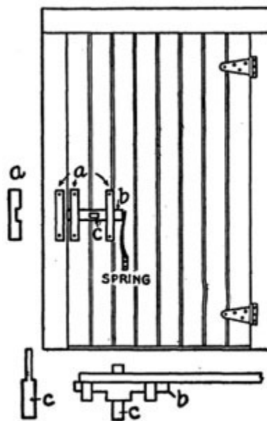
FIGURE 2—SPRING FASTENER
