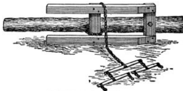
FIGURE I—LOGGING BOB
