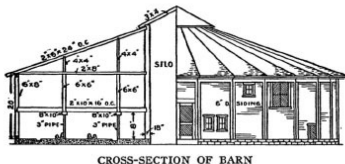
CROSS-SECTION OF BARN
