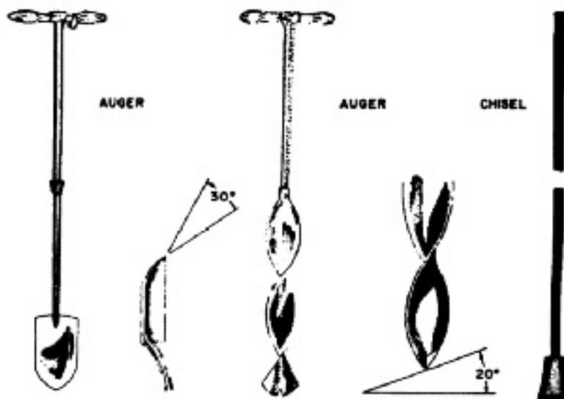
Figure 8-35. Types of ice augers and ice chisel.
