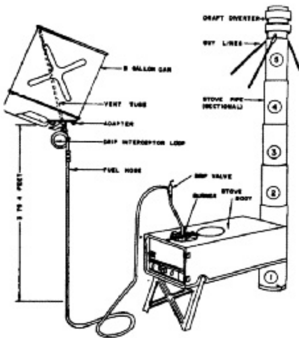
2 Installation setup
