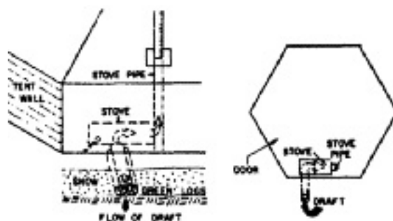
Figure 3-7. Draft channel for stove.
