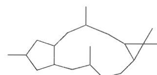
Fig. 6.60. Lathyrane
