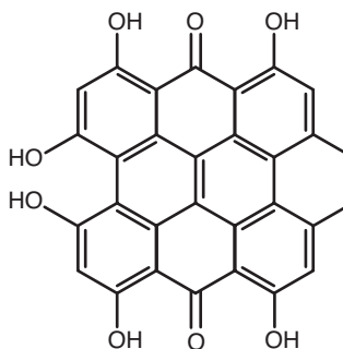
Figure 6.1 Chemical structure of hypericin (Wikipedia)
