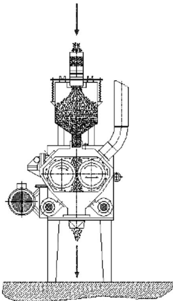
FIGURE 4.56 Rubber-roll sheller. (From Rubber-roll sheller S10 PR. Reinbek, Germany: FH Schule Muehlenbau GmbH.)
