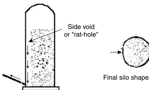
FIGURE 4.51 Rat-holing leads to unbalanced sidewall forces. (From Ministry of Agriculture, Food and Rural Affairs, Government of Ontario, Canada, http://www.omafr.gov.on.ca/english/engineer/facts/88-070.htm .)
