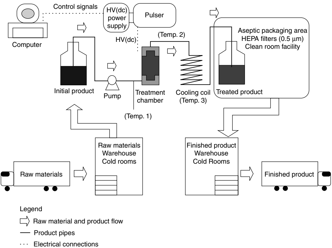
FIGURE 33.9 PEF unit operations layout.
