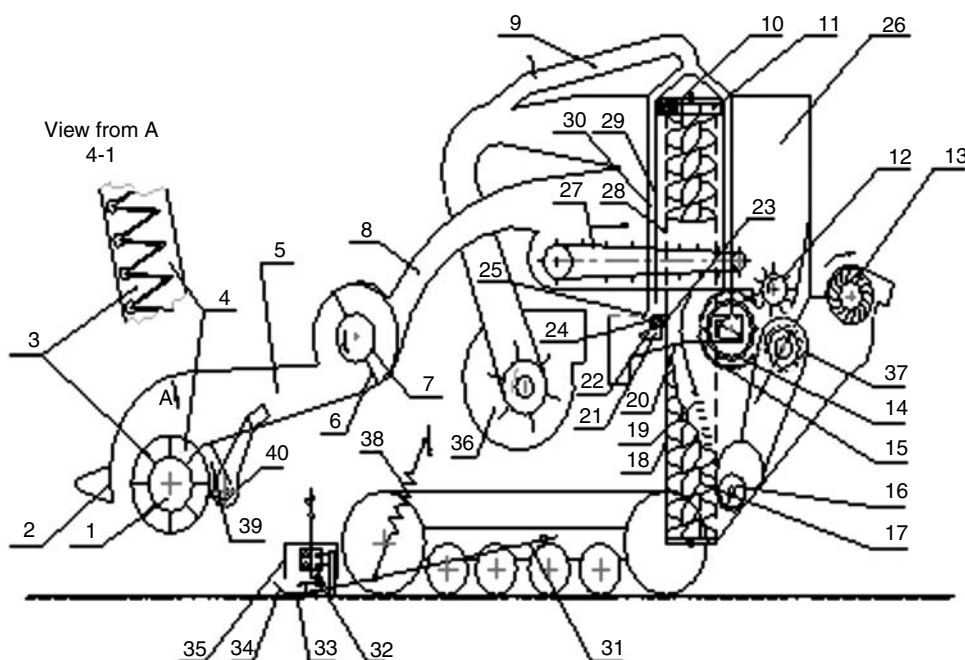
FIGURE 4.23 Schematic arrangement of combine stripper harvester for rice and wheat: 1. stripping rotor; 2. hood; 3. teeth on rotor; 4. stagger-positioned teeth on conduit bottom; 5. conduit; 6, 7. tines and drum of raking booster; 8, 9. conduit; 10. exit for recycling; 11. blade; 12. discharge rotor; 13. cross-flow fan; 14. major re thresher; 15. concave; 16. horizontal auger; 17. vertical auger; 18. auger case; 19. shutter; 20. container; 21. discharge blade; 22. sheave; 23. ball bearing; 24. blade on ring distributor; 25. conic reflector; 26. depositing chamber; 27. belt conveyor; 28. cylindrical sieve; 29. intermediate cylinder; 30. outer cylinder; 31. pushing rod; 32. crank shaft roller; 33. knife; 34. guard with upward point; 35. rod of revolving rake; 36. fan; 37. detachable axial-flow re thresher; 38. suspension spring; 39. recovery chamber; 40. impeller-blower. (From Y. Jiang et al. In: G.R. Quick, Ed. Proceedings of the International Conference on Crop Harvesting and Processing , Louisville, KY, 2003.)
