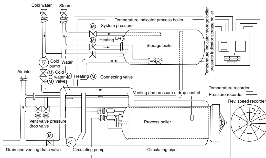
FIGURE 24.4 Horizontal circulating water retort. (From Perkins, W.E., Introductions to the Fundamentals of Thermal Processing , Sleeth, R.B., ed., IFT, Chicago, November 15, 1979, p. 82.)
