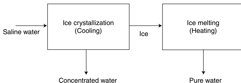
FIGURE 27.1 Freezing–melting process.
