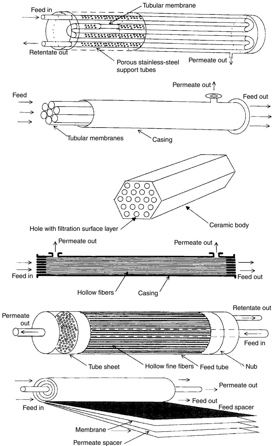
FIGURE 16.2 Membrane modules. (Adapted from Mannapperuma, J. D., In Handbook of Food Engineering Practice , CRC Press, Boca Raton, FL, 1997.)
