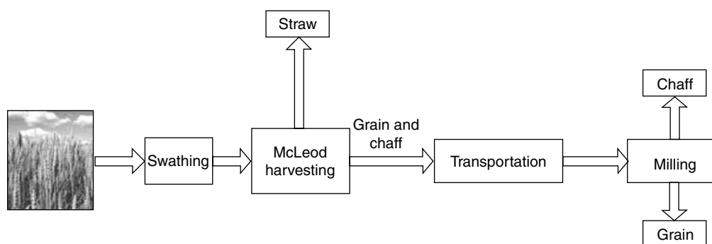
FIGURE 4.16 Sequential operation of McLeod harvesting system. (From S. Sokhansanj et al. Dynamic simulation of McLeod harvesting system for wheat, barley, and canola crops. Paper No. 048010. St. Joseph, MI: American Society of Agricultural Engineers, 2004.)
