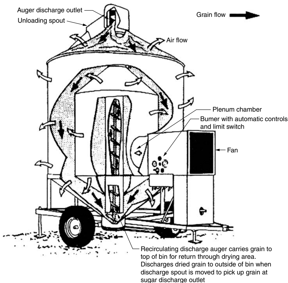
FIGURE 4.28 Recirculating batch dryer. (From K.J. Hellevang, W.F. Wilcke. Maintaining corn quality for wet milling. AE-1119, Extension Service, North Dakota State University, Fargo, ND, 1996.)
