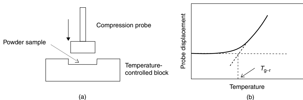
FIGURE 17.9 (a) Principles of measurement of stickiness of powder by thermal mechanical compression test (TMCT) method; (b) T_{g-r} indicates glass–rubbery transition when the powder is scanned through temperature.
