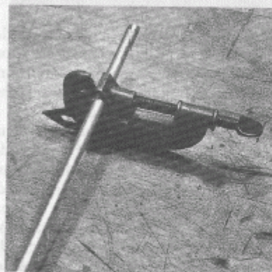
Using a small tube cutter, cut sections of tubing into 2 1/2-inch segments.
