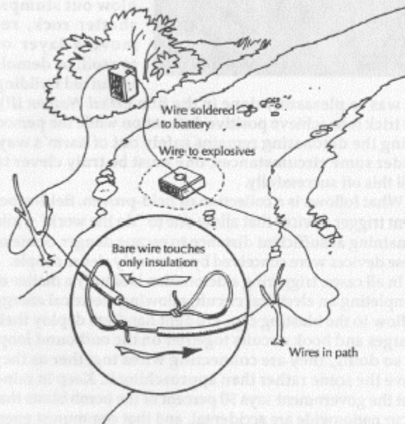
FIGURE 1: TRIP TRIGGER
