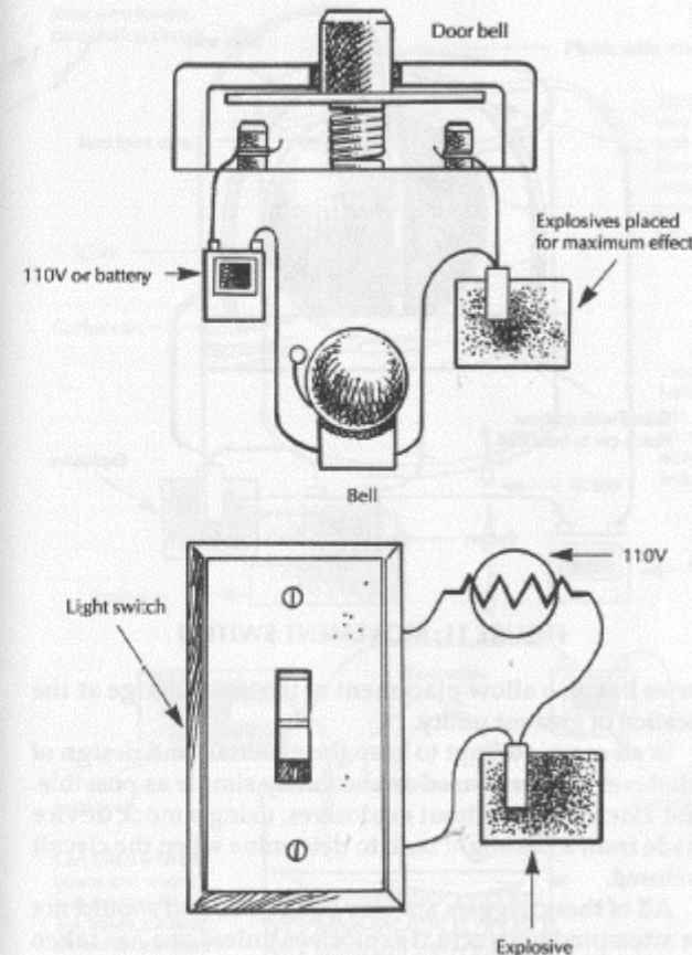
FIGURE 10: COMMON SWITCHES MADE INTO TRIGGERS
