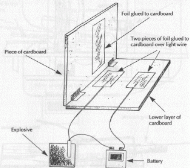
FIGURE 8: FOIL AND WIRE TRIGGER
