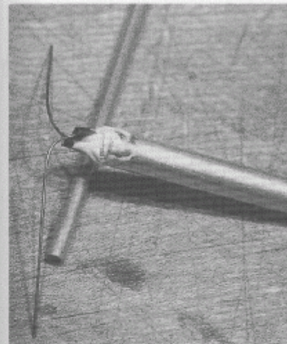
Bend bridge wires down, but keep them separated. Cut to about 1 inch in length.
