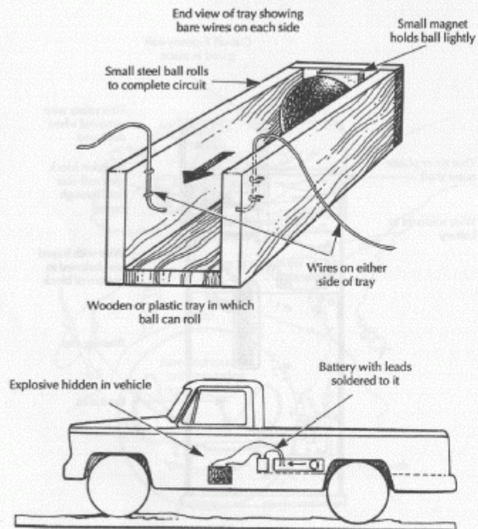
FIGURE 3: INERTIA TRIGGER
