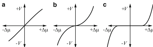
Fig. 8.13 Symmetrical with respect to the value of the chemical potential difference curves for the rates of growth and dissolution of crystals for the different growth mechanisms discussed above. +v : rate of growth; -v : rate of dissolution; (a) normal growth, (b) spiral growth, (c) two-dimensional nucleation. As far as the process of direct incorporation and dissolution of particles proceeds on the same sites for normal growth the same linear dependence is to be expected for growth and dissolution. Spiral growth or dissolution starts with relatively low absolute values of \Delta\mu , while for growth mediated by two-dimensional nucleation a threshold has to be reached, before perceptible growth takes place. Such symmetric curves are found experimentally only for small supersaturations
