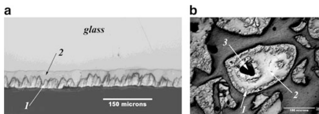
Fig. 14.23 Illustration of the possible effects of elastic stresses in the crystallization of semolina glass samples (see text and [179–182])
