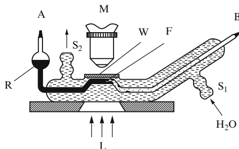
Fig. 8.19 Crystallization cell with glass capillary in which the mode of growth mediated by two-dimensional nucleation was demonstrated for \text{Na}_2\text{S}_2\text{O}_3 \cdot 5\text{H}_2\text{O} : A, B – sealed glass capillary; W – optical window; S_1 , S_2 – input and output for thermostat water; F – advancing crystal front. A seed crystal was initially introduced at R (According to Gutzow, Razpopov, and Kaischew (1970) [324])
