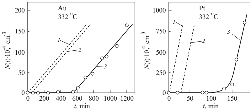
Fig. 7.14 Kinetics of nucleation in \text{NaPO}_3 -melts induced by gold and platinum crystallization cores. Curve (1): Expected N(t) -curve when no transient effects are involved; curve (2): Possible shift of the N(t) -curves accounting for the growth of the crystalline clusters to visible dimensions; curve (3): Experimentally observed N(t) -curves
