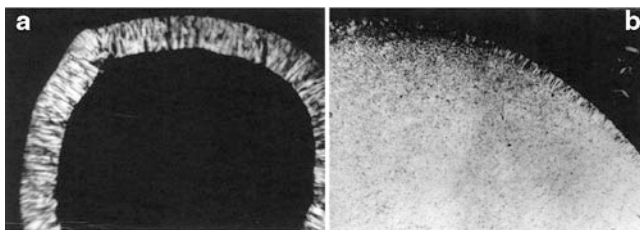
Fig. 7.20 Surface and bulk devitrification of \text{NaPO}_3 -glass rods heat treated for 150 min at 320^\circ\text{C} . ( left side ) Crystalline layer at the surface of a \text{NaPO}_3 -sample. ( right side ) Crystallization of a sample in which bulk devitrification is initiated by the addition of 5 \cdot 10^{-3} wt % platinum forming a population of platinum crystallization cores. Despite the addition of the bulk initiator of crystallization, surface nucleation is clearly visible (micrograph of thin slides at 50 magnification, crossed nicols)
