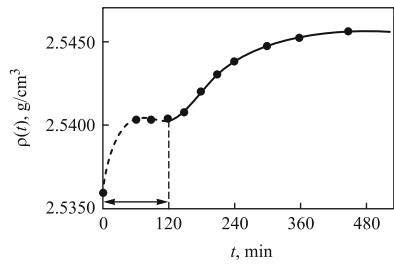
Fig. 10.6 Pycnometric determination of surface crystallization of a Na-silicate glass at 520^{\circ}\text{C} (glass semolina sample with \bar{d} = 0.75 - 1.0 mm). Note the initial stabilization process ( broken line ) preceding crystallization
