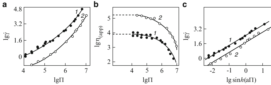
Fig. 12.4 Stress-induced flow of poly(methyl metacrylate) melts as an example of a pseudo-plastic Non-Newtonian liquid. Experimental data are reported by Gul and Kulesnev (1966) [282]: (a) \log(d\gamma/dt) vs \log(\Pi) data for two temperatures interpolated by applying the de Waele-Ostwald equation. (b) Stress dependence of the apparent viscosity. (c) Experimental (d\gamma/dt) vs \Pi data in coordinates according to the Prandtl-Eyring model; (black dots): data for 523 K; (circles) data for 473 K
