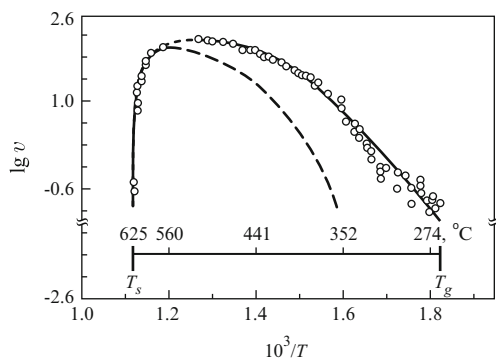
Fig. 8.21 Temperature dependence of the rate of linear growth of \alpha — \text{NaPO}_3 from its own melt in coordinates \lg v vs. 1/T . The growth rate determined experimentally is given by a full line . The theoretical prediction obtained according to the dislocational growth mechanism when viscosity data are used for the determination of the impingement rate Z is shown by a dashed curve
