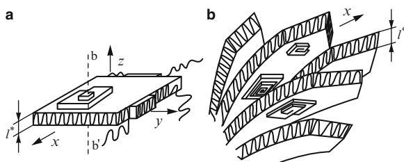
Fig. 8.9 Illustration of possible modes of polymer crystal growth. (a) A plate-like polymer crystal of thickness, l^* , growing in the x - y -plane via the formation of two-dimensional regular reentry nuclei. With (bb') the position of the Burgers vector of a screw dislocation is indicated around which a growth front could have been developed. Screw dislocation growth fronts can be formed only on flat non-growing surfaces of the lamellae. (b) Polymeric lamellae growing from a common spherulitic center
