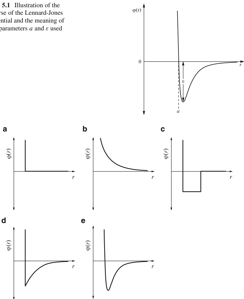
Fig. 5.2 Schematic representation of other often used pair-interaction potentials: (a) Hard spheres; (b) point center of repulsion; (c) rectangular potential well; (d) Sutherland potential; (e) Lennard-Jones or Mie-potential
