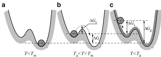
Fig. 2.32 Mechanical analogy for an interpretation of the differences between the stable at T < T_m crystalline state (a), the metastable melt (b) and the glass below T_g (After Simon and Jones (1949) [409]). In this mechanical analogy the crystalline state corresponds to an absolute minimum of the potential well, the under-cooled melt to a higher local minimum. In order to be transferred from the metastable to the stable crystalline state the system has to overcome a potential barrier \Delta G_c . \Delta G is the thermodynamic driving force of crystallization. The glass is represented in this analogy by a ball glued to the wall of the potential well above the minimum (c). Crystallization is commonly preceded by stabilization processes, the thermodynamic force of stabilization \Delta G_s is also indicated
