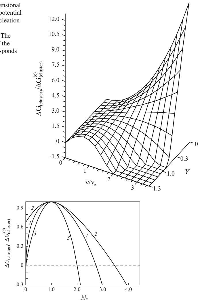
Fig. 6.20 The thermodynamic barrier of nucleation and its different analytical descriptions. Curve (1): (\Delta G_{(cluster)}) / \Delta G_{(cluster)}^{(c)} according to Eq. (6.47); curve (2): the classical Taylor-series approximation Eq. (6.108) as applied, e.g., by Becker and Döring; curve (3): inverted parabola approximation for polymer nucleation (Eq. (6.200), Gutzow and Dobрева (1992) [310])
