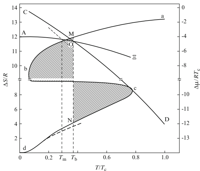
Fig. 5.6 Temperature dependence of the total entropy ( S/R ) (curve (abcd) ) and of the chemical potential ( \Delta\mu/k_B T ) of the liquid ( AB ), the vapor ( CD ) and of the crystal ( EF ). T_c and p_c are the critical values of pressure and temperature of the system. The dashed curve in the figure represents the entropy of the substance in the state of a perfect crystal using Einstein's approximation in the calculation of the partition function. By T_b the boiling point is indicated. With T_m the melting point is denoted, again, i.e., the temperature, where the \Delta\mu curves of the liquid and the crystal intersect. In order to illustrate the position of the melting point more clearly the slope of the \Delta\mu -curve of the crystal has been increased by a factor five (For further details see Milchev and Gutzow (1981) [560])
