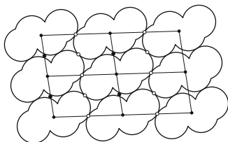
Fig. 4.13 Close packing of molecules with complex shape according to Kitaigorodski (1955) [457]. Note the small fraction of free volume as compared with close packing of equally sized spheres
