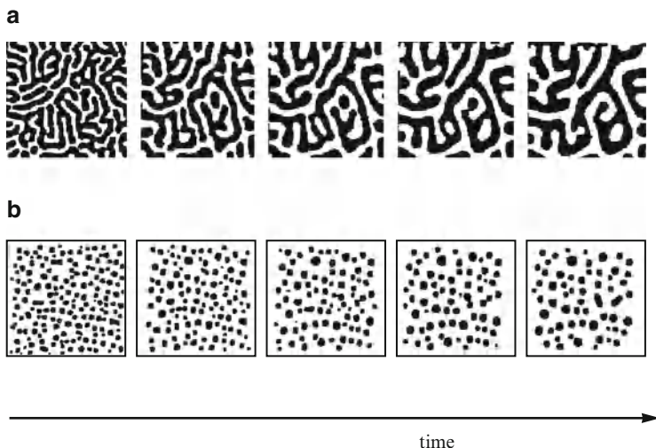
Fig. 11.3 Different stages of a phase transformation as obtained, as a rule, by (a) spinodal decomposition and (b) nucleation and growth
