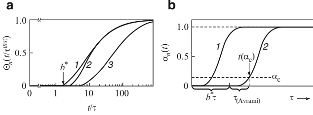
Fig. 10.4 Influence of non-steady state effects in nucleation on the kinetics of overall crystallization. (a) Possible \Theta(t/\tau^{(ns)}) -dependencies (for n = 3 ): (1) The exact Gutzow-Kashchiev solution accounting only for transient nucleation effects; (2) the approximative solution (Eq. (10.18)) obtained with the step function approach (Eq. (6.173)); (3) the Shneidman-Weinberg correction accounting for both steady-state effects and size-dependent growth rates (for \Delta G_{(cluster)}/k_B T = 20 ). (b) \alpha_n(t) -dependencies: (1) the steady-state solution; (2) the Gutzow-Kashchiev result with a shift of the curves along the time-axis according to Eqs. (10.17) and (10.18). With \alpha_c a just detectable degree of crystallization is indicated, which in the case of transient nucleation is reached after a time interval t(\alpha_c) = b^* \tau^{(ns)} + \tau_{(Avrami)}
