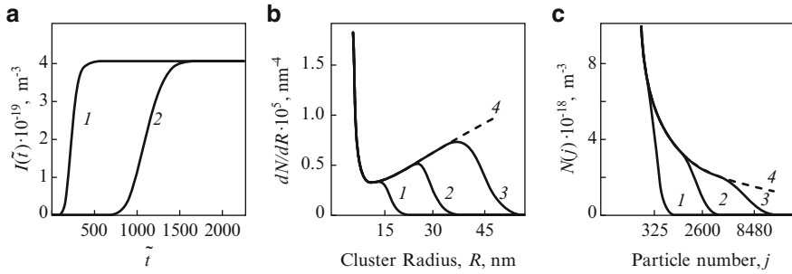
Fig. 6.10 (a) Change of the nucleation rate as a function of reduced time, \tilde{t} , for clusters of different sizes ( R = 1.08 nm (curve (1)) and R = 2.76 nm (curve (2)) obtained by the numerical solution of the set of kinetic equations, Eqs. (6.94)–(6.95). In the calculations the supersaturation in the system is kept constant. (b) and (c) Evolution of the cluster size distribution in nucleation taking place at constant supersaturation expressed through the cluster radius ( dN/dR ), (b) and the number of particles, j , contained in it (c) for different moments of reduced time \tilde{t} : \tilde{t} = 460 (1); \tilde{t} = 1,160 (2) and \tilde{t} = 2,310 (3)
