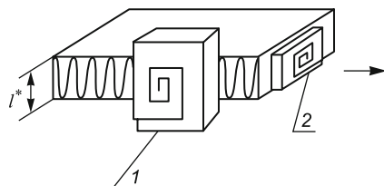
Fig. 8.10 Illustration of the conclusion that dislocational spirals cannot develop on the growth front of a polymer chain-folding crystal. The number (1) indicates a growth spiral having the necessary inter-coil distance allowing a further growth. The number (2) shows a growth spiral with a size adjusted to the growing crystal front, it has inter-coil distances lower than required for a stable growth
