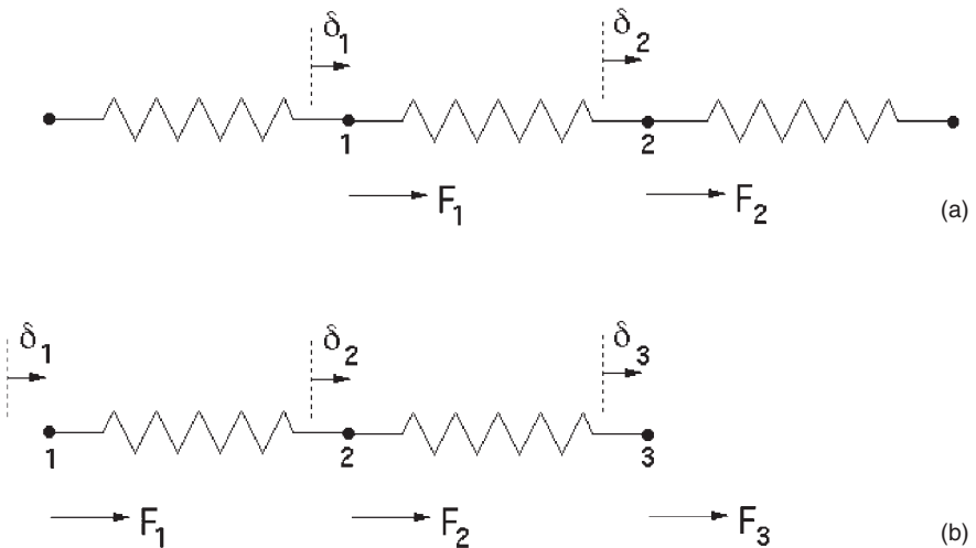
Fig. 14.15 Forces on springs.
