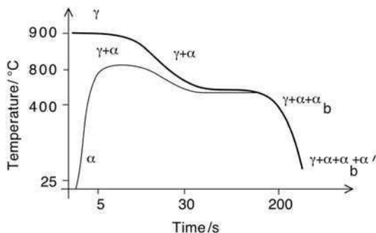
Fig. 10.12 The two kinds of heat treatment used to generate the microstructures of TRIP-assisted steels. The terms \gamma , \alpha , \alpha_b and \alpha' represent austenite, allotriomorphic ferrite, bainite and martensite, respectively.
