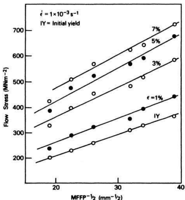
Fig. 2.10 Dependence of the flow stress at several strains on the MFFP in a pearlitic steel (Takahashi and Nagumo, Transactions of the Japan Institute of Metals 11, 113, 1970).
