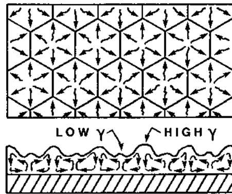
FIG. 6 Diagram of convection flow. (From Ref. 4, used with permission.)
