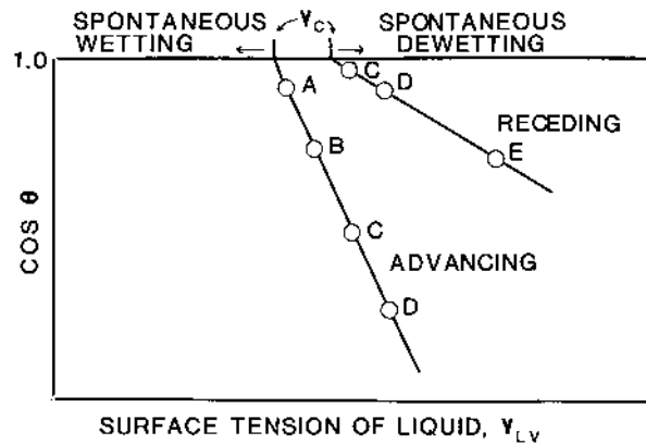
FIG. 17 Critical surface tension (Zisman) plots for advancing and receding contact angles. Liquid A wets the surface very well, B does not wet as well, but will not dewet. Liquids C, D, and E dewet. (From Ref. 5, used with permission.)
