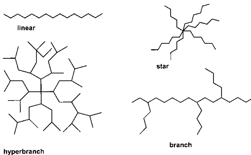
FIG. 9 Polymer architecture.
