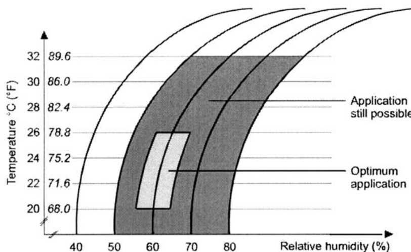
Fig. 8 Processing window for application of waterbased basecoats.
