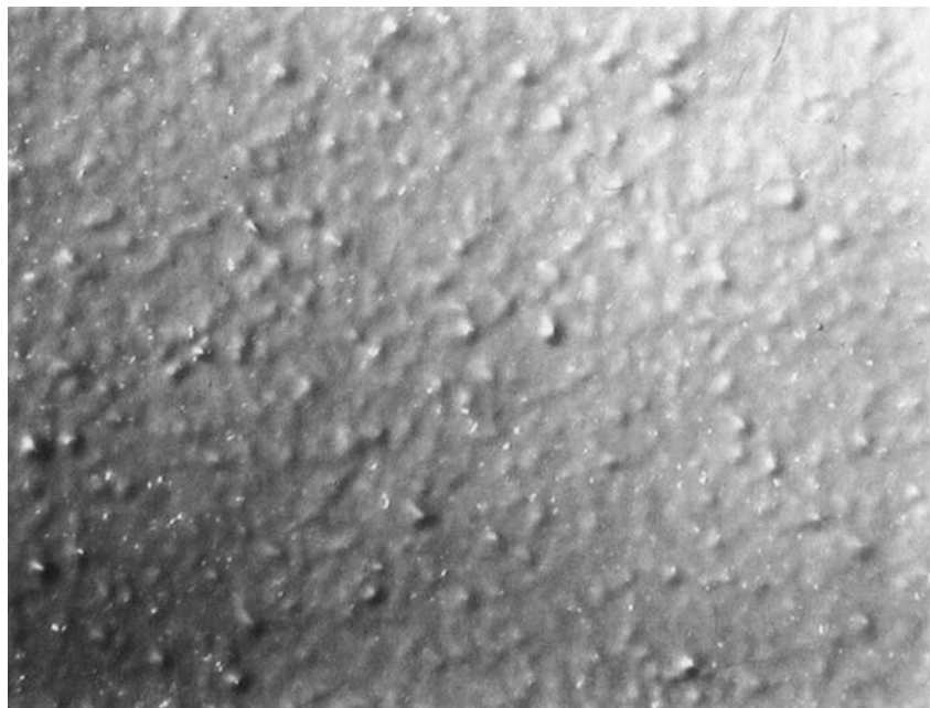
Fig. 12 Example of micropopping. Perhaps, microbumps is a more accurate description in this case. To the eye, the effect is one of fuzziness of reflections.
