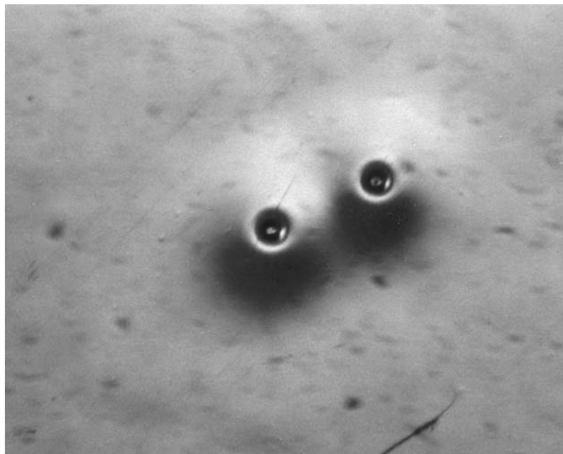
FIG. 9 Solvent popping. (From Ref. 5, used with permission.)
