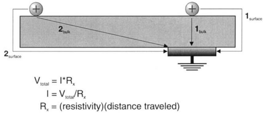
FIG. 28 Charge dissipation currents divide across all available paths using relative power (IR drop) losses just as they would in a parallel electrical circuit.
