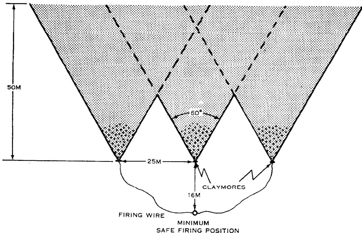
Figure 8. Diagram of lateral separation pattern of (CLAYMORES).
