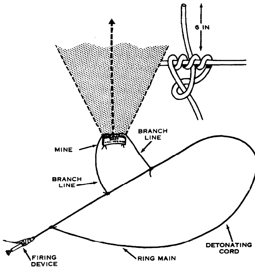
Figure 13. Nonelectric firing system.
