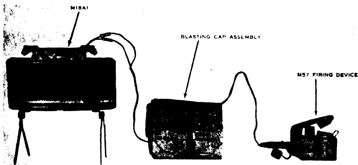
Figure 7. The M18A1 antipersonnel mine with the M57 firing device connected.
