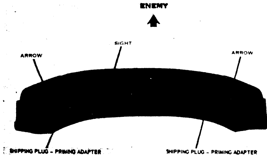
Figure 10. Top view of the M18A1 antipersonnel mine.
