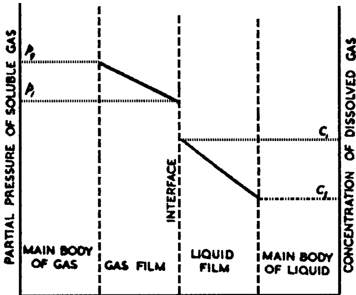
Figure 2. Two-film theory.
