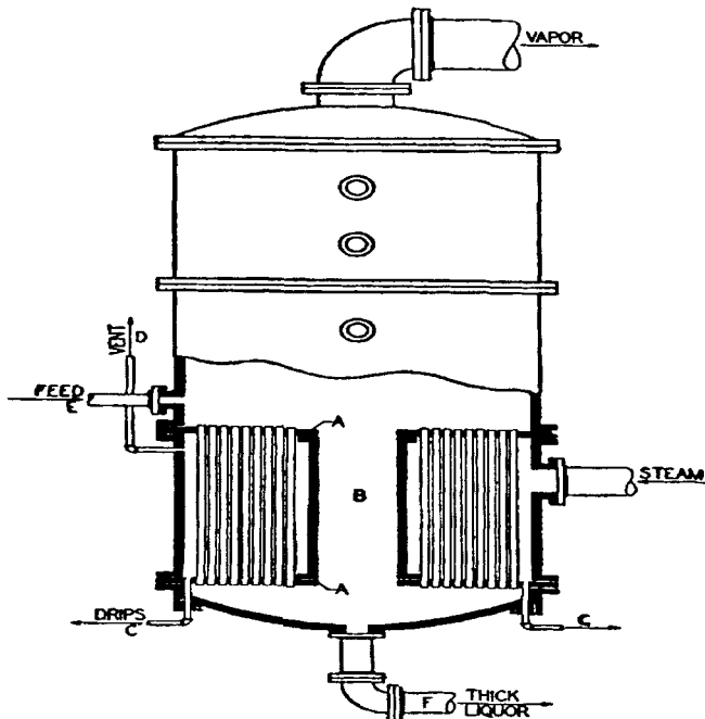
Figure 11. Vertical tube evaporator: (A) Tube sheets; (B) Downtake; (C) Condensate outlet; (D) Non-condensed gas outlet; (E) Liquor inlet; (F) Thick liquor outlet.
