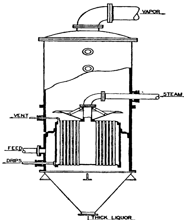
Figure 10. Basket type vertical tube evaporator.
