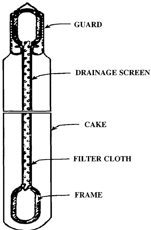
Figure 20. Sectional view.
