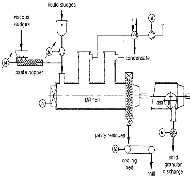
Figure 19. Process flow scheme for continuous contact drying of residues and sludges.
