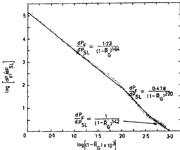
Figure 27. Empirical correlation between pressure drop and hold-up.
