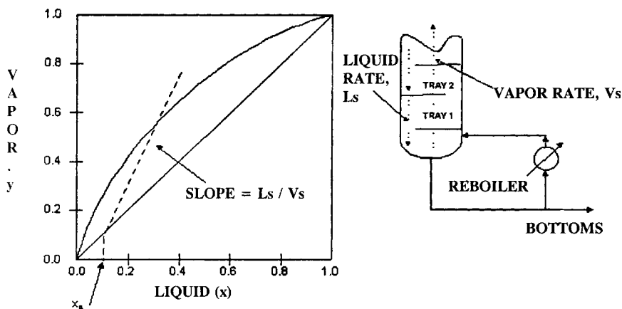
Figure 14. Construction of operating line for stripping section.
