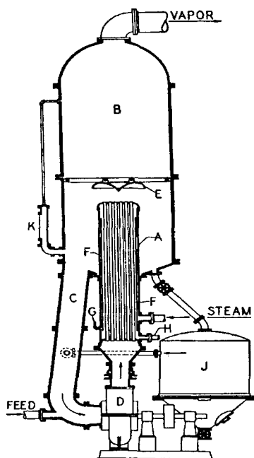
Figure 9. Forced circulation evaporator.
