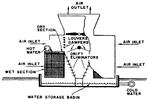
Figure 5. Single structure type wet-dry cooling tower.
