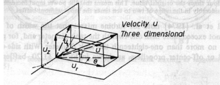
Figure 12. Variation of velocity distribution in a mixing tank on insertion of full side wall baffles.
