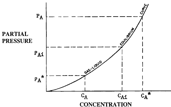
Figure 8. Gas-liquid equilibrium curve.
