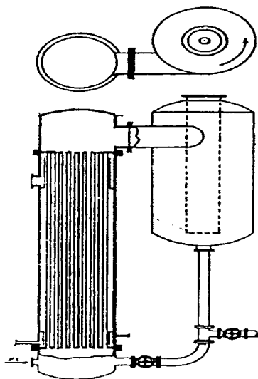
Figure 5. Natural circulation, long tube film evaporator.
