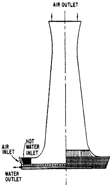
Figure 2. Hyperbolic cooling tower.
