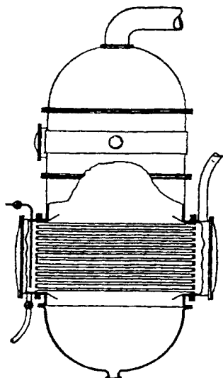
Figure 4. Horizontal design.
