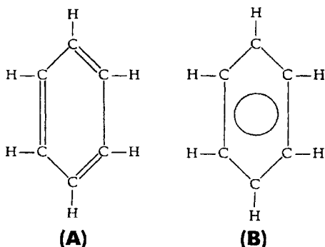
Figure 17. The structure of benzene: (A) conventional illustration of double bonds, (B) illustration implying resonance.
