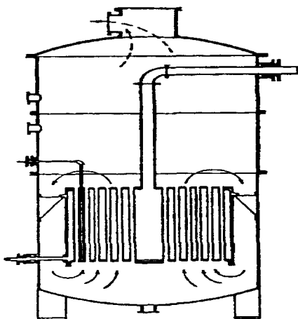
Figure 3. Vertical long-tube evaporator.
