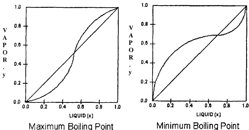
Figure 11. VLE curves for azeotropic systems.
