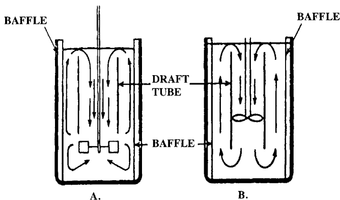
Figure 16. Draft tubes in baffled tanks: (A) turbine; (B) propeller.
