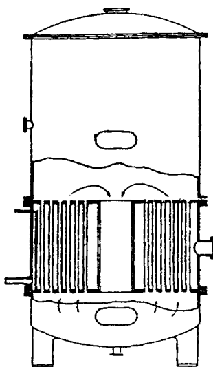
Figure 2. Vertical evaporator.
