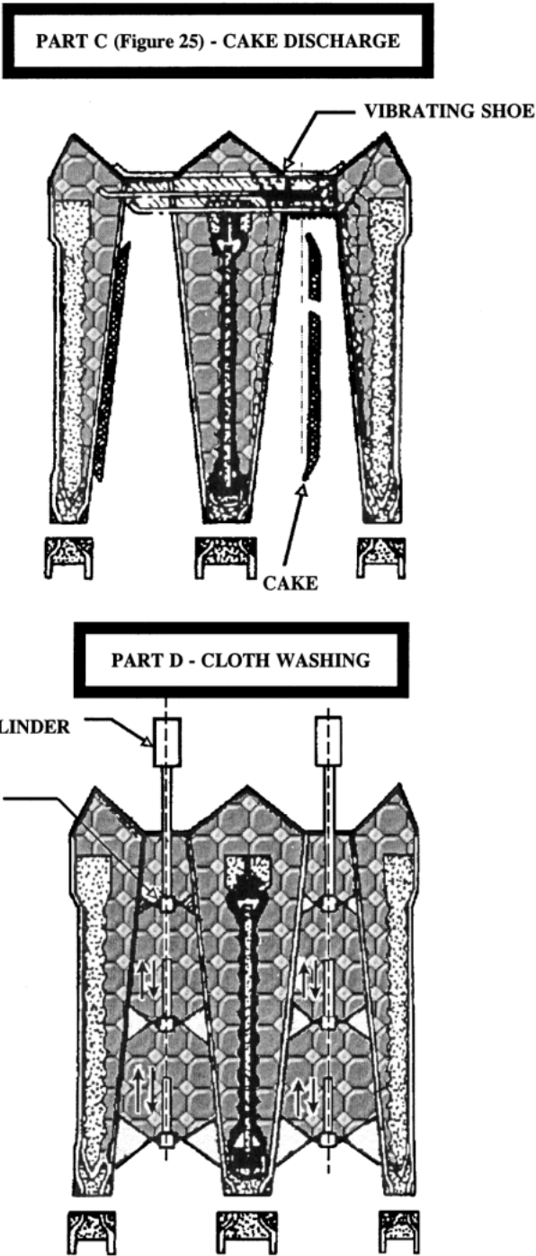
Figure 25. Diaphragm press operating cycles.
