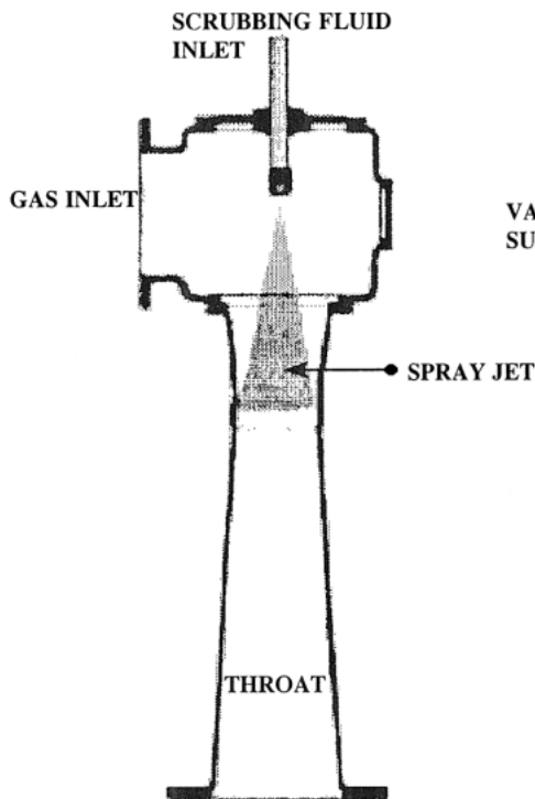
Figure 16. Venturi scrubber.
