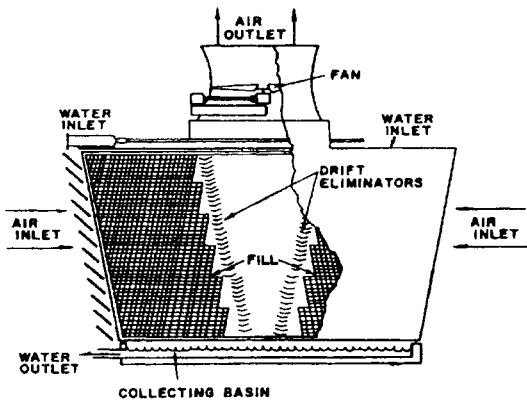
Figure 4. Crossflow cooling tower.
