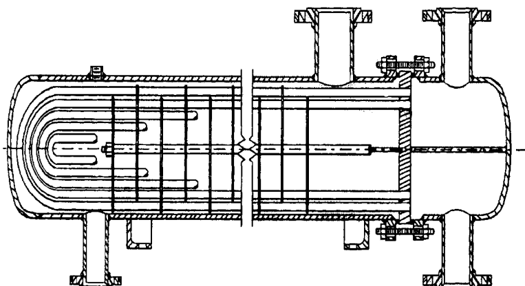
Figure 7. U-tube design.
