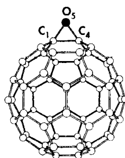
epoxide (6-6 bonded)
