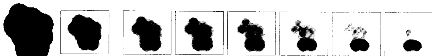
Nitrated nitrobenzene intermediate—meta form
