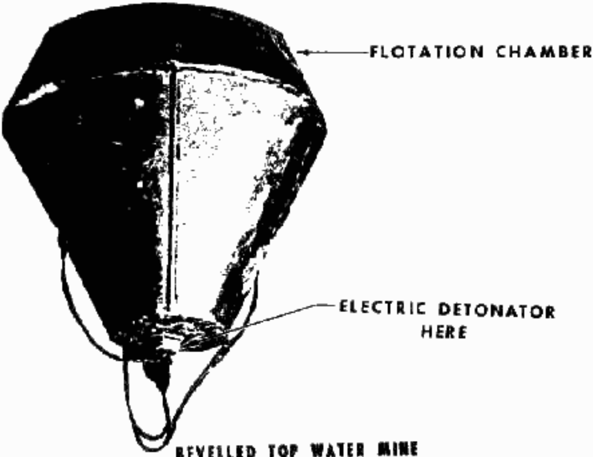
BEVELLED TOP WATER MINE 43 Truncated Cone Water Mine GENERAL DESCRIPTION AND COMMENT
