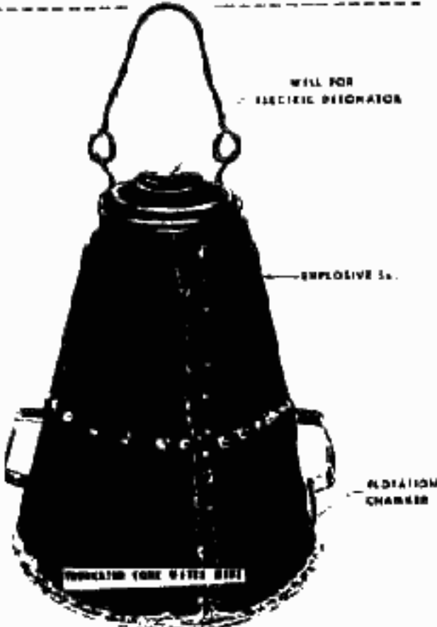
45 Small Truncated Cone-Shaped Charge GENERAL DESCRIPTION AND COMMENT
