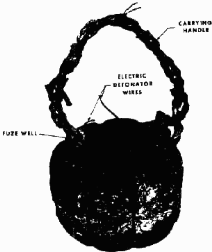
DETOL BOX MINE 29 Turtle Mine
