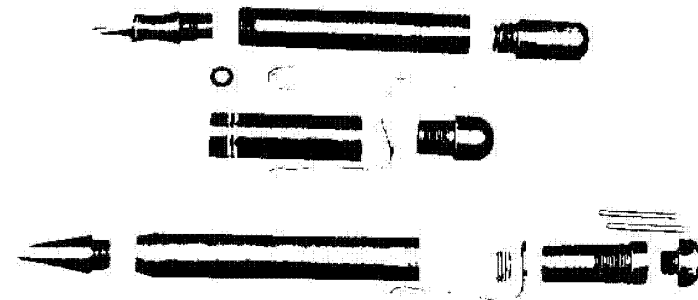
Figure 49 (UNCLASSIFIED). German pen-and-pencil delay fuze (U).
