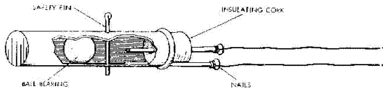
Figure 31 (UNCLASSIFIED). British ball bearing switch (doorknob device) (U).
