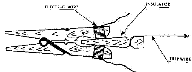
Figure 29 (UNCLASSIFIED). FLN clothespin firing device (pull-operated) (U).
