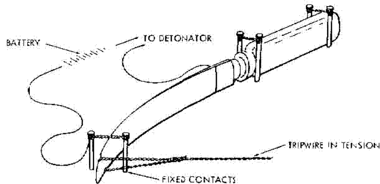
Figure 28 (UNCLASSIFIED). British knife switch (U).
