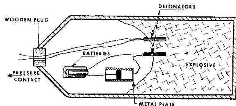
Figure 24 (UNCLASSIFIED). FLN ontilt mine (U).
