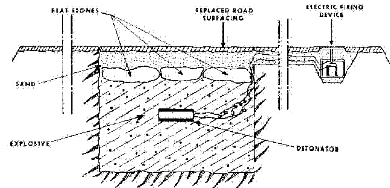
Figure 23 (UNCLASSIFIED). FLN antivehicle mine (U).
