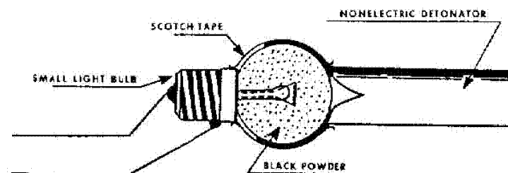
Figure 34 (UNCLASSIFIED). FLN electric detonator (U)
