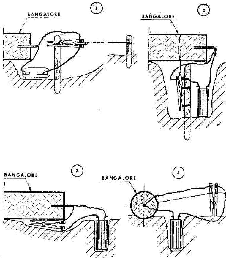
Figure 45 (UNCLASSIFIED). FLN bangalore torpedo boobytraps (U).
