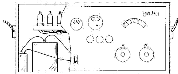
Figure 42 (UNCLASSIFIED). Japanese boobytrapped radio (U).
