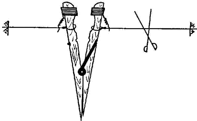
Figure 30 (UNCLASSIFIED). FLN clothespin firing device (tension-release-operated) (U).
