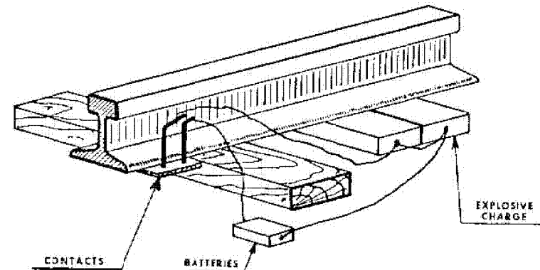
Figure 32 (UNCLASSIFIED). FLN wheel-flange firing device (U).
