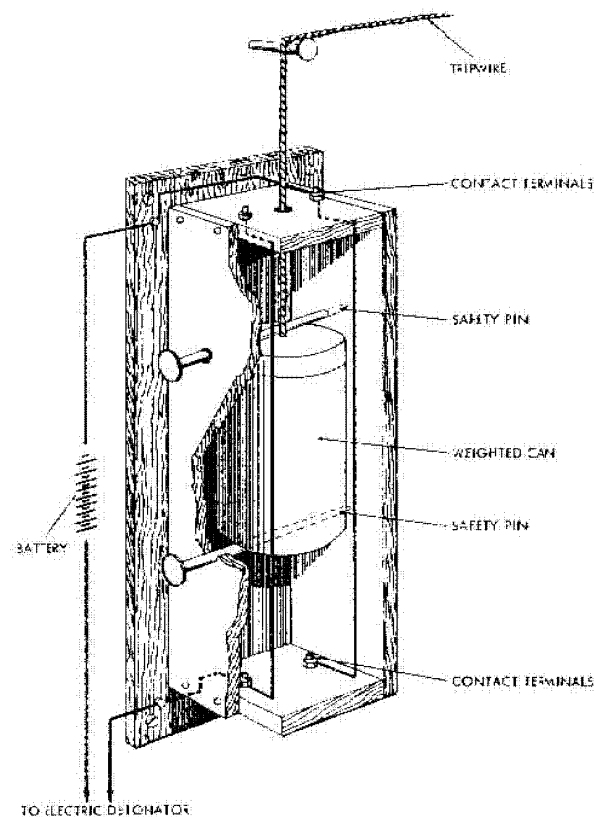
Figure 27 (UNCLASSIFIED). British weighted-can firing device (U).
