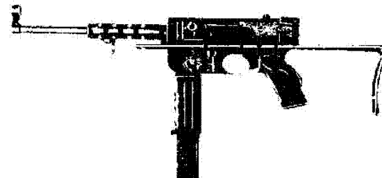
Figure 14 (UNCLASSIFIED). North Vietnamese modified MAT-49 (U).
