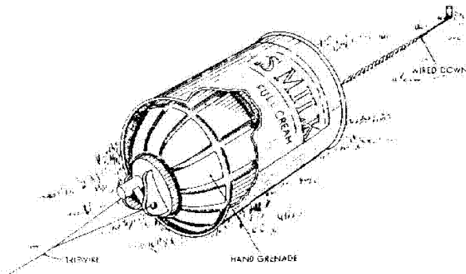
Figure 18 (UNCLASSIFIED). British grenade-in-can mine (U).
