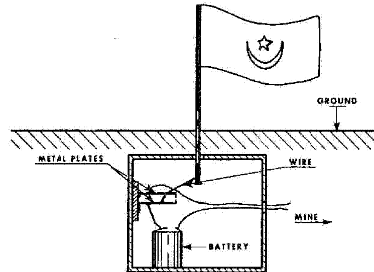
Figure 46 (UNCLASSIFIED). Flag mine (U)
