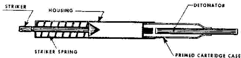
Figure 26 (UNCLASSIFIED). FLN improvised fuze (U).
