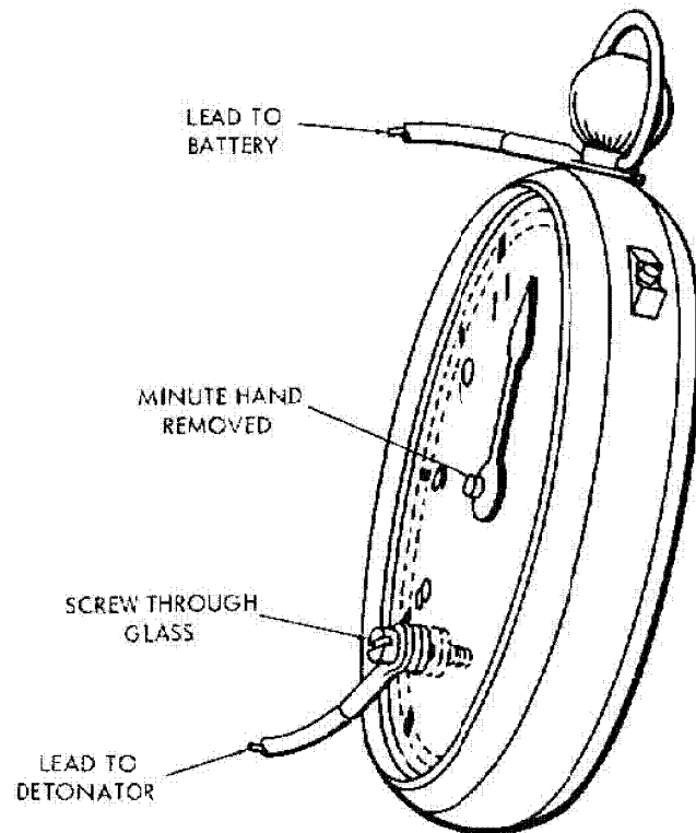
Figure 37 (UNCLASSIFIED). German pocket watch delay. (U).
