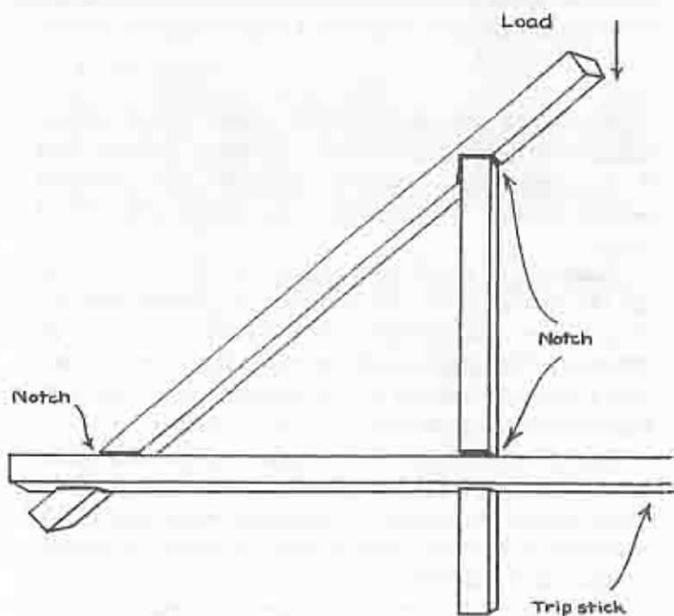
FIGURE 4 TRIGGER
