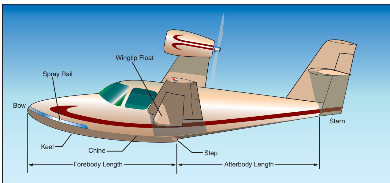
Figure 2-2. Hull components.
