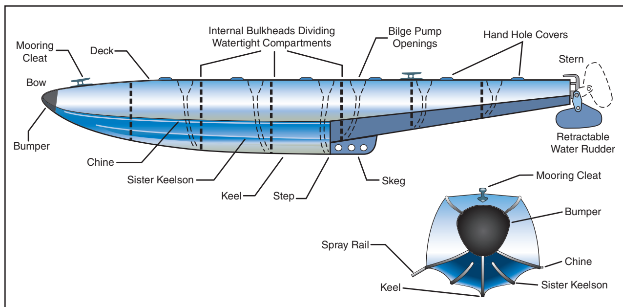
Figure 2-3. Float components.
