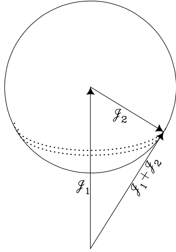
Figure 7.13 Classically the sum vector \mathbf{J}_1 + \mathbf{J}_2 can line anywhere on the sphere of radius |\mathbf{J}_2| around the end of \mathbf{J}_1 .
