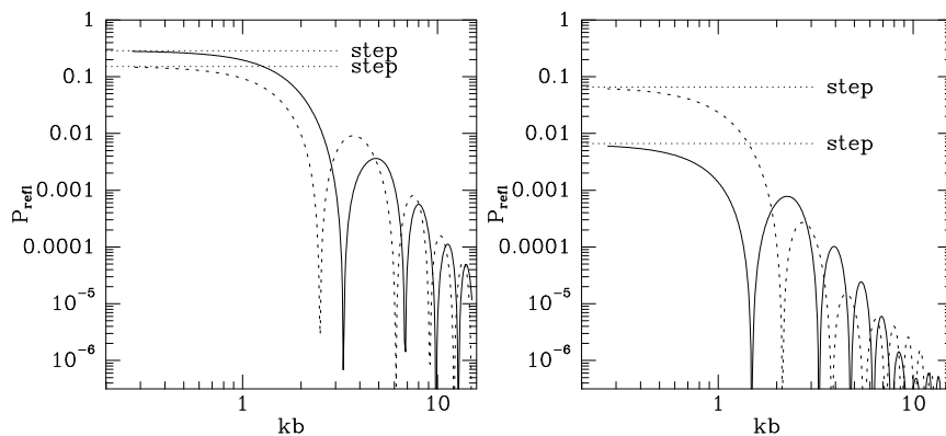
Figure 5.21 Each curve shows the reflection probability when a particle with kinetic energy E encounters a region in which the potential V(x) smoothly changes to V_0 over a distance 2b , and then smoothly returns to zero; the change in V is given by equation (5.69) with x replaced by x + a , and the fall is given by the same equation with x replaced by -(x - a) . The full curves are for ka = 30 and the dashed curves for ka = 15 . The left panel is for barriers of height V_0 = 0.7E , while the right panel is for potential wells ( V_0 = -0.7E ).
