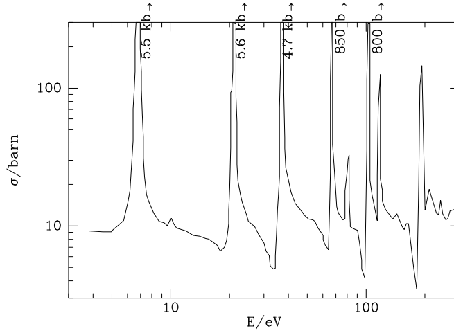
Figure 5.19 The total cross section for the scattering of neutrons by ^{238}\text{U} nuclei. (From data published Bollinger, L.M., et al., Phys.Rev, 105, 661 (1957))
