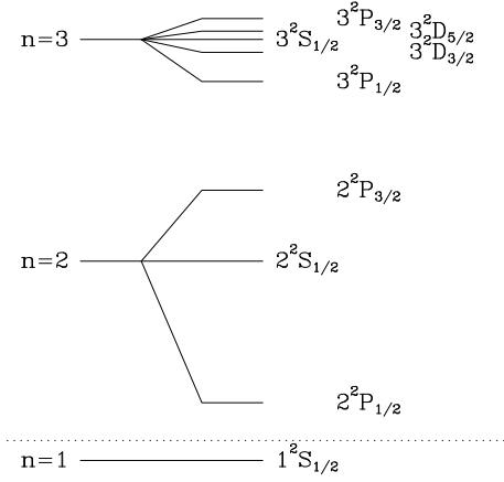
Figure 8.5 The fine structure of a hydrogen-like ion with Z = 200 that is predicted by equation (8.72a). The dotted line denotes a break in the energy scale so that the ground state can be included.
