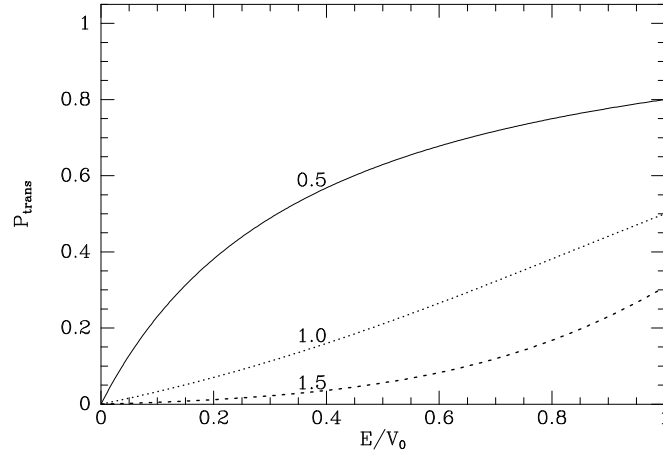
Figure 5.12 The transmission probability for a particle incident on a potential-energy barrier of height V_0 and width 2a as a function of the particle's energy. The curves are labelled by the values of the dimensionless parameter (2mV_0a^2/\hbar^2)^{1/2} .
