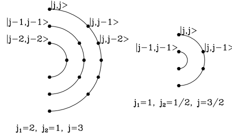
Figure 7.11 The left panel shows states obtained by adding a system of angular momentum j_2 = 1 to one with j_1 = 2 , while the right panel is for j_1 = 1 and j_2 = \frac{1}{2} .
