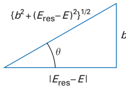
Fig. 14.11 The construction required for the derivation of eqn 14.68.
