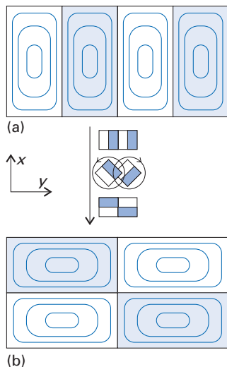
Fig. 2.25 An example of accidental degeneracy: the two functions shown here schematically are degenerate even though one cannot be transformed into the other by a symmetry transformation of the system. Note, however, that a hidden symmetry (the separate rotation of the two halves of the box) does interconvert them.
