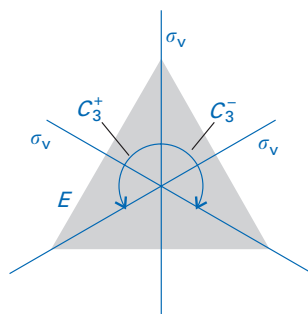
Fig. 5.18 The symmetry elements of the group C_{3v} .
