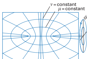
Fig. 8.4 The elliptical coordinates \mu , \nu , and \phi used for the separation of variables in the exact treatment (within the Born–Oppenheimer approximation) of the hydrogen molecule-ion.
