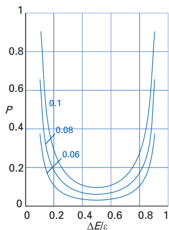
Fig. 11.20 The probability of energy transfer for the model in the previous illustration as a function of the energy separation \Delta E . The numbers labelling the curves are the values of a/\varepsilon . Perturbation theory fails unless P \ll 1 .
