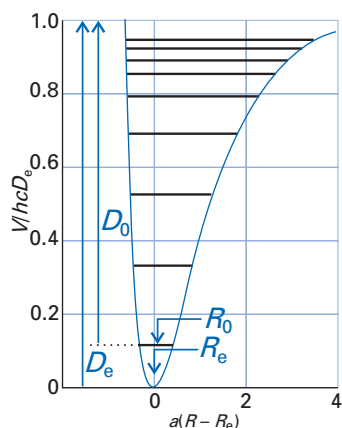
Fig. 10.16 The vibrational energy levels of a molecular oscillator. Note the convergence of levels as the potential becomes less confining. The curve is a plot of the Morse potential.
