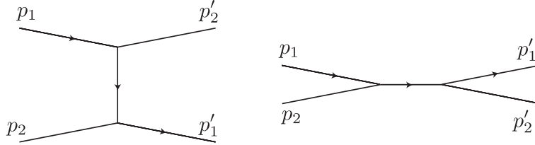
FIG. V.15 Diagrams contributing to N\phi \rightarrow N\phi .
