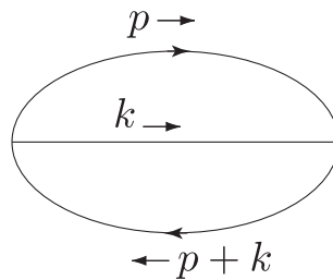
FIG. V.10 Feynman diagram corresponding to matrix element (V.91).
