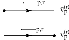
FIG. X.6 Feynman rules for external fermion legs.
