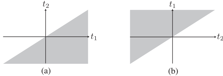
FIG. V.4 The shaded regions correspond to the region of integration in (a) Eq. (V.46) and (b) Eq. (V.47).
