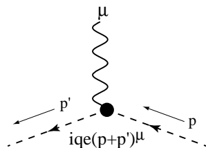
FIG. XI.5 Feynman rule for the derivatively coupled charged scalar.
