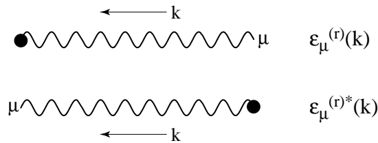
FIG. XI.3 Feynman rules for external vector particles.
