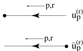
FIG. X.3 Feynman rules for external fermion legs.
