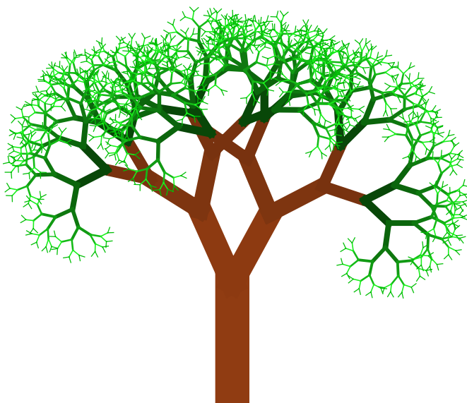
Figure 7.2.3. Fractal tree.
