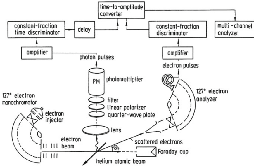
Fig. 2.34 Scheme of a typical electron-photon coincidence apparatus for observing polarized photons perpendicular to the scattering plane, defined by the incoming and scattering electrons; after Standage and Kleinpoppen (1975)
