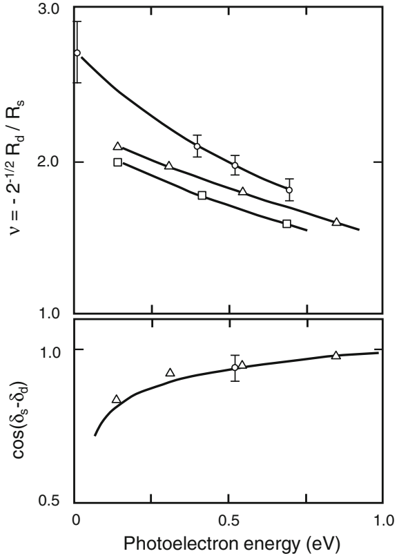
Fig. 4.31 Parameters of photoionization of \text{Ne}^*(2p^5 3p^3 D_3) . Experimental results are shown together with calculations by Chang (1982) ( \triangle ) and Luke (1982) ( \square ). Adapted from Siegel et al. (1983)
