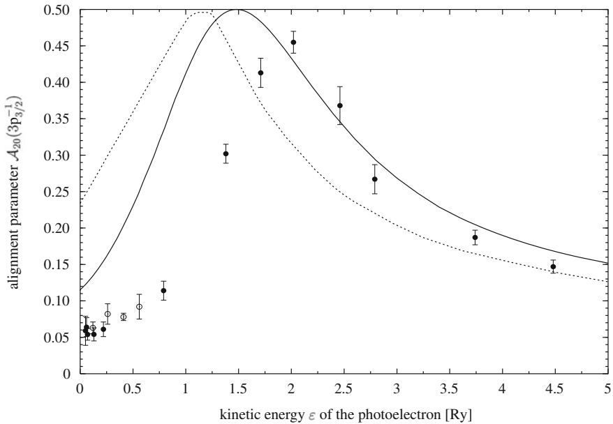
Fig. 3.16 Alignment parameter A_{20} of the photoionized calcium 3p_{3/2} inner shell hole state as a function of the kinetic energy \varepsilon of the photoelectron; numerical results: (—) HFR (Kleiman and Lohmann 2003), (· · · · ·) HS (Berezhko et al. 1978a); experimental data: (●) Kämmerling et al. (1994), (○) Fanis et al. (1999); after Kleiman and Lohmann (2003)
