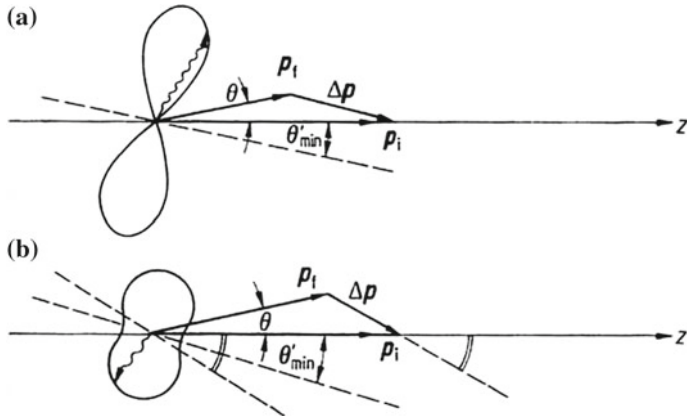
Fig. 2.37 Relation between the electron-photon angular correlation and the momentum transfer \Delta \mathbf{p} for the helium excitation/de-excitation process 1^1S_0 \rightarrow 2^1P_1 \rightarrow 1^1S_0 by electron impact. The electron has initial momentum \mathbf{p}_i and, after the scattering, a momentum \mathbf{p}_f . The length of the wavy arrows is proportional to the coincident photon intensity in the direction of observation: a after Born approximation, \Delta m_\ell = 0 refers to \Delta \mathbf{p} as axis where no change of the orbital angular momentum component m_\ell is possible for the 1^1S_0 \rightarrow 2^1P_1 transition; b according to typical experimental observation
