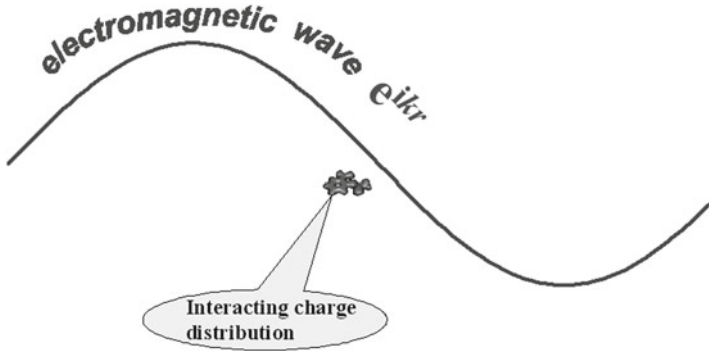
Fig. 4.1 An illustration to the dipole approximation
