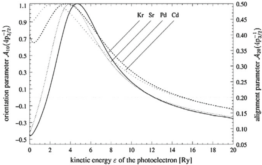
Fig. 3.13 Alignment A_{20} and orientation A_{10} data and their interdependence of the inner shell 4p_{3/2} hole state photoionization of krypton, strontium, palladium, and cadmium as a function of the kinetic energy \varepsilon of the photoelectron; after Kleiman and Lohmann (2003)
