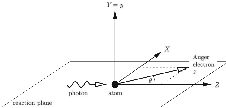
Fig. 3.8 The reaction plane and coordinate frame defined for synchrotron beam excitation (Lohmann et al. 2003b)
