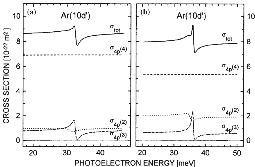
Fig. 4.34 Total and partial J = 2, 3, 4 cross sections for photoionization of \text{Ar}^*(3p^54p\ ^3D_3) atoms in the region of the 10d' resonances: a deduced from experiment; b calculated. After Schohl et al. (1997)
