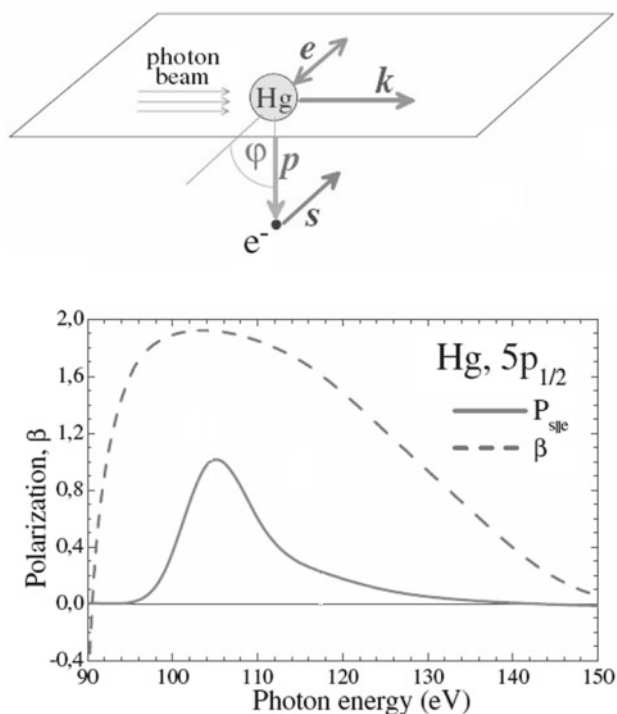
Fig. 4.53 (Bottom) the degree of transverse polarization of the photoelectrons (—) ejected from the 5p_{1/2} subshell of Hg by linearly polarized light for the displayed geometry (top), where \mathbf{k} , \mathbf{e} , \mathbf{p} and \mathbf{s} denote the directions of the photon beam, its linear polarization, photoelectron emission and spin polarization component, respectively. The asymmetry parameter \beta in the angular distribution of the photoelectrons is also shown (---). Adapted from Cherepkov et al. (2003)
