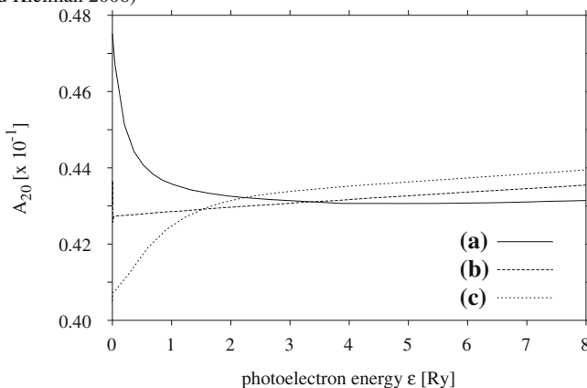
Fig. 3.23 Alignment \mathcal{A}_{20}^{3,3/2} of manganese for the L_3 photoionization of the Mn 2p_{3/2}^{-1}4s^23d_{3/2}^5 ; J = 3 fine structure state using the Mn (a), \text{Mn}^{5+} (b), and Ca (c) configuration potentials; after Lohmann and Kleiman (2006)
