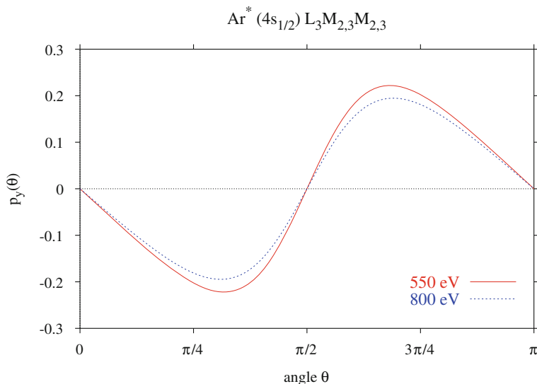
Fig. 3.28 The P_y -component of the spin polarization vector for the resonant \text{Ar}^* (4s_{1/2}) L_3 M_{2,3} M_{2,3} {}^2D_{5/2} final state Auger transition as a function of the Auger emission angle \theta . (—): electron impact energy 550 eV, (· · · · ·): electron impact energy 800 eV; after Lohmann et al. (2002)
