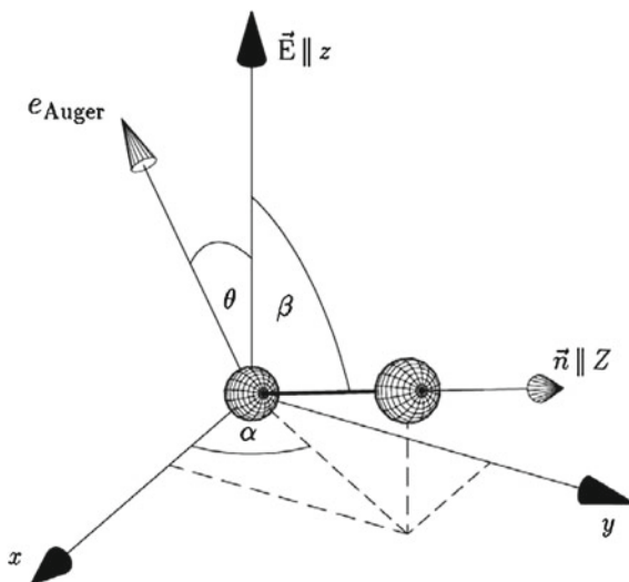
Fig. 3.30 Angles for molecular axes and Auger electrons related to the space-fixed frame xyz ; after Bonhoff et al. (1999)
