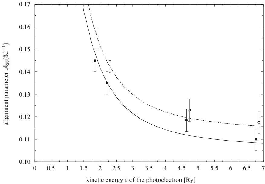
Fig. 3.17 Alignment parameter A_{20} of the photoionized krypton 3d inner shell hole state as a function of the kinetic energy \epsilon of the photoelectron; numerical results: (—) 3d _{3/2} and (---) 3d _{5/2} HFR calculation (Kleiman and Lohmann 2003); experimental data: (●) 3d _{3/2} and (○) 3d _{5/2} (Kämmerling et al. 1989, 1992a); after Kleiman and Lohmann (2003)
