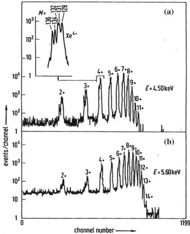
Fig. 2.5 a Time-of-flight charge spectrum of Xe ions with positive charges from \text{Xe}^{2+} to \text{Xe}^{11+} produced by synchrotron radiation of photon energy h\nu = 4.50 keV and a neutral Xe target; the enlarged spectrum above at the top left-hand corner shows the mass numbers of various isotopes for \text{Xe}^{4+} ; b charge spectrum of \text{Xe}^{2+} up to \text{Xe}^{14+} at a photon energy of h\nu = 5.60 keV (after Tonuma et al. 1987)
