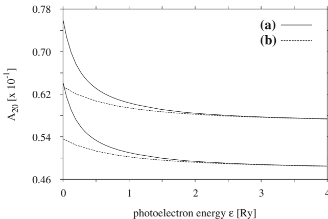
Fig. 3.22 Alignment \mathcal{A}_{20}^{J,1/2} of gold for the photoionized Au 2p_{3/2}^{-1}6s_{1/2} ; J = 1 (bottom) and J = 2 (top) fine structure states using the Au (calc. a) and \text{Au}^+ (calc. b) configuration potentials (after Lohmann and Kleiman 2006)
