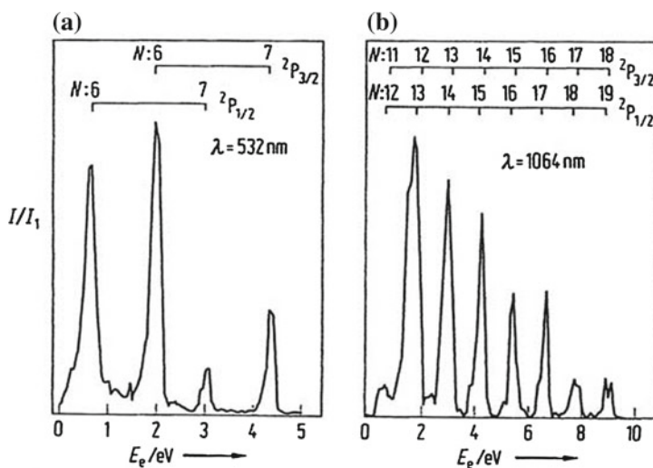
Fig. 2.11 Photoelectron spectra, including ATI peaks in the multiphoton ionization of the Xe atom. a Laser wavelength of the ionizing radiation \lambda = 532 nm; b laser wavelength \lambda = 1064 nm. The numbered rows N give the number of photons absorbed by the atom. E_e is the photoelectron energy, I the signal intensity of the photoelectrons in arbitrary units I_1 (after Humpert et al. 1985)
