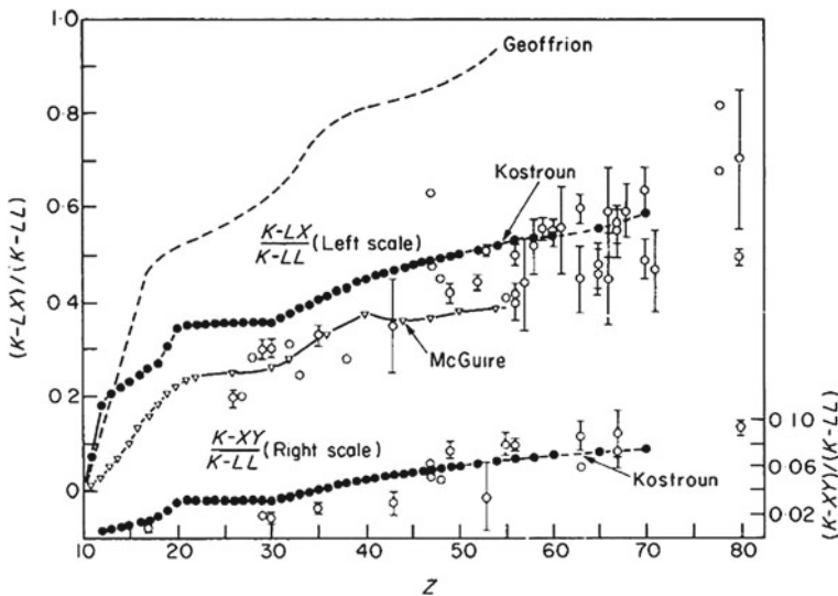
Fig. 3.2 Theoretical and experimental KLX/KLL and KXY/KLL Auger transition probability ratios as a function of the atomic number (after Kostroun et al. 1971). Calculated ratios: Geffrion and Nadeau (1959); Kostroun et al. (1971); McGuire (1970). Measured relative intensities of the K Auger electron groups assembled by Erman et al. (1964); except for the following ratios: Zn (Bellicard et al. 1956), Co (Bellicard et al. 1957), Te (Casey and Albridge 1969), and Ce and Nd after D'yakov and Rogachev (1962)
