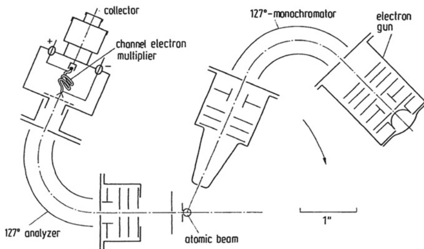
Fig. 2.25 Schematic diagram of a double electrostatic analyzer (after Pavlovic et al. 1972) with two cylindrical 127° electron analyzers (as monochromator for the primary electron beam and as analyzer for the scattered electrons) and electro-optical elements for focussing and extracting the electrons; a channel electron multiplier serves for the detection of the electrons after passing the analyzer. An atomic beam crosses the electron beam of the monochromator perpendicular to the plane of the figure (1" = 2.54 cm)
