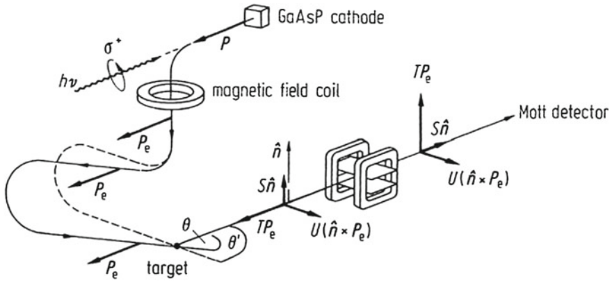
Fig. 2.60 Orientation of the polarization \mathbf{P}_e of electrons from the GaAsP cathode as a source of polarized electrons into a Mott detector in the apparatus of Fig. 2.59
