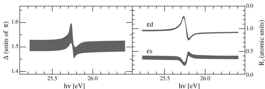
Fig. 4.28 Same as Fig. 4.27 but in the region of the autoionizing O^*(2s2p^4 3^3D) resonance. The error limits are represented by the shadowed zone. Adapted from Plotzke et al. (1996)
