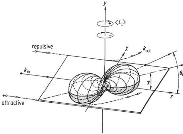
Fig. 2.41 Typical form of the electron cloud for a coherently excited 2^1P_1 state with an orientation angle \gamma = 45^\circ and angular momentum transfer \langle L_\perp \rangle = 0.75 \hbar . The incoming electrons k_{in} are scattered under the angle \theta_e ( k_{out} ) whereby either a repulsive and/or an attractive potential is effective
