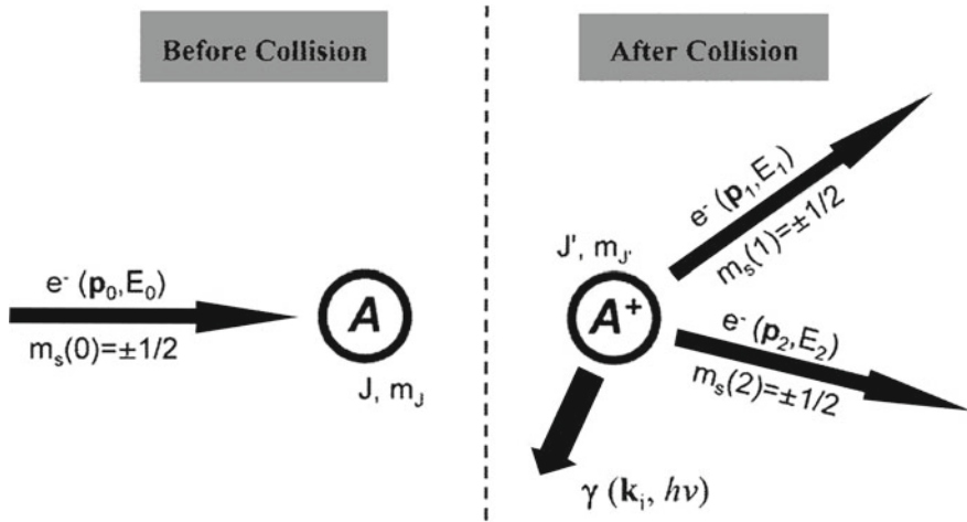
Fig. 2.64 Kinematical and quantum mechanical variables of the (e, 2e) process: momenta of the continuum electrons \mathbf{p}_0 , \mathbf{p}_1 , \mathbf{p}_2 , their spin projections m_s and angular momentum states of the atomic target and the residual ion (after Lower et al. 2004)
