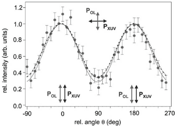
Fig. 4.42 Variation of the upper sideband yield in the low field regime (about 8 \times 10^{10} \text{ W/cm}^2 ) for the two-photon ionization in the 1s shell of He at 13.7 nm as a function of the relative angle between the linear polarization vectors of the free electron laser and the optical (800 nm) laser. (—): fit to the experimental data (●). The results of time-dependent second-order perturbation theory (---), and “soft-photon” approximation (·····) are almost identical. After Meyer et al. (2008)
