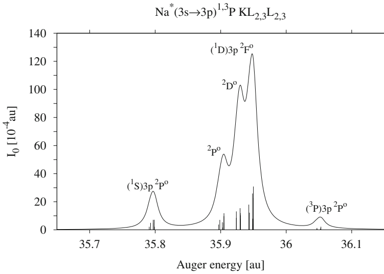
Fig. 3.5 The multiplet splitting of the 3s \rightarrow 3p laser excited Na \text{KL}_{2,3}\text{L}_{2,3} Auger lines (Na D-doublet) following 1s shell ionization. The Auger decay is from the resonantly excited unresolved ^1\text{P}_1 and ^3\text{P}_{0,1,2} fine structure states
