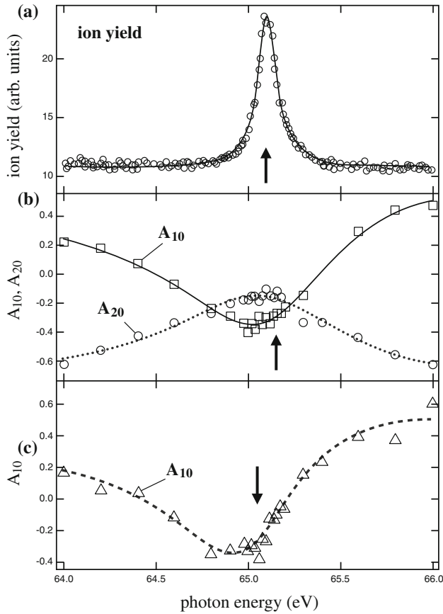
Fig. 4.45 a \text{Xe}^*(4d^{-1}6p)_{J=1} resonance in the total ion yield; b alignment and orientation parameters of the photoion in the (5p^4\ ^3P_2\ 6p[1])_{3/2} state; and c orientation parameter for the (5p^4\ ^1D_2\ 6p[1])_{1/2} state. (States with J = 1/2 cannot be aligned). The energy dependence of the orientation and alignment parameters is fitted by (4.98). Arrows indicate the energy positions of the corresponding Fano profiles. After Grum-Grzhimailo et al. (2005)
