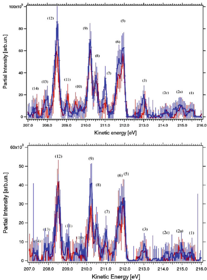
Fig. 3.11 The spin resolved spectrum of the \text{Ar}^*2p_{1/2}^{-1}3d_{3/2} Auger decay. Peak numbers as assigned in Table 3.9. Experimental results measured with (top) circularly and (bottom) linearly polarized light. (Blue) spin parallel, (red) spin anti-parallel to the direction of photon propagation (after Turri et al. 2007)
