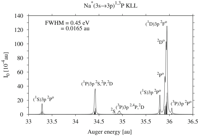
Fig. 3.4 The 3s \rightarrow 3p laser excited KLL Auger spectrum of sodium after ionization of the 1s shell. The Auger decay propagates from the resonantly excited unresolved ^1P_1 and ^3P_{0,1,2} fine structure states
