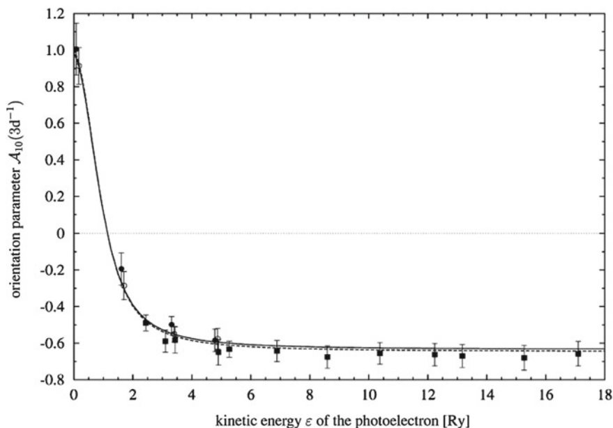
Fig. 3.18 Orientation parameter A_{10} of the photoionized krypton 3d inner shell hole state as a function of the kinetic energy \varepsilon of the photoelectron; numerical results: (—) 3d_{3/2} and (---) 3d_{5/2} HFR calculation (Kleiman and Lohmann 2003); experimental data: (●) 3d_{3/2} and (○) 3d_{5/2} (Schmidtke et al. 2001), (■) 3d mean value (Snell et al. 2002); after Kleiman and Lohmann (2003)
