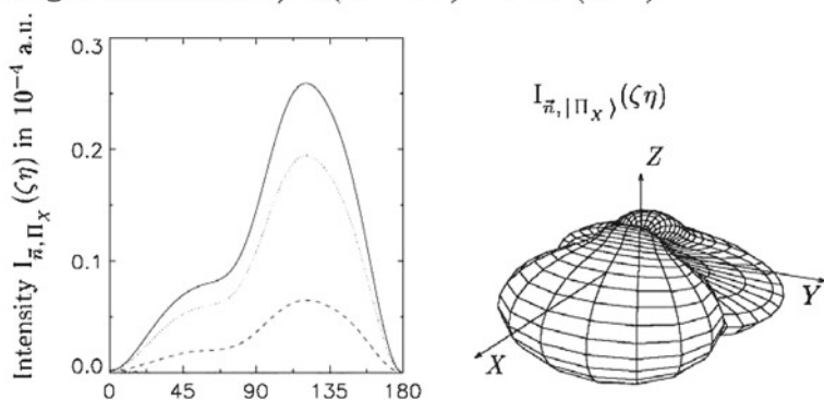
Fig. 3.34 Angular distribution of the emitted Auger electrons from axis-fixed CO molecules; the molecules are initially excited in a pure |\Pi_X\rangle state. ( Left column ): I_{\vec{n},|\Pi_X\rangle} as a function of \zeta for various fixed values of \eta . ( Right column ): I_{\vec{n},|\Pi_X\rangle}(\zeta, \eta) as a spherical plot. (—): \eta = 0^\circ , (·····): \eta = 30^\circ , (---): \eta = 60^\circ , (- · -): \eta = 90^\circ . Labels b and c refer to Table 3.17; after Bonhoff et al. (1999)
