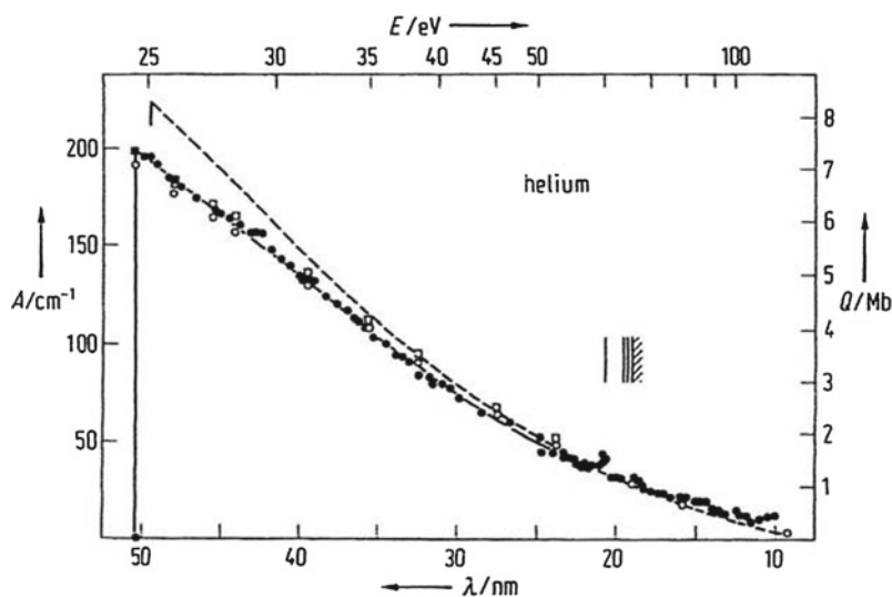
Fig. 2.14 Photoionization cross section Q and absorption coefficient A of helium as a function of the energy of the incident photons of energy E or wavelength \lambda . (○) experimental data of Samson (1964) and (●) Lowry et al. (1965) in comparison to various dipole approximations; (□) Stewart and Webb (1963); (---) Cooper (1962). The short vertical lines at 20 nm indicate the positions of unresolved resonances (see Fig. 2.3)
