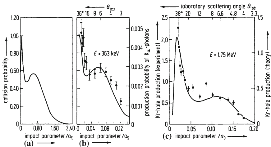
Fig. 2.72 Impact parameter dependence of a the Lyman- \alpha excitation of the (\text{H}^+ + \text{H}) collision system according to theoretical predictions by Bates and Williams (1965), b the production of a K-electron hole in a 363\text{ keV} (\text{Ne}^+ + \text{Ne}) collision (experimental data and theoretical curve after Sackmann et al. 1974), and c a L-electron hole production from a 1.75\text{ MeV} (\text{Kr}^+ + \text{Kr}) collision (after Shanker et al. 1984)
