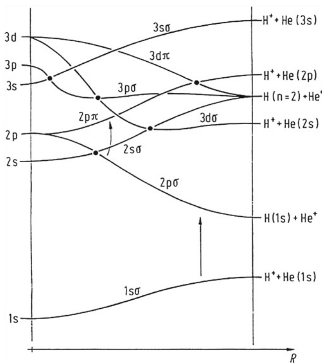
Fig. 2.81 Correlation diagram (schematic) for the collision process \text{H}^+ + \text{He} \rightarrow \text{H} + \text{He}^+ ( R = internuclear distance). Note that the nucleus at R = 0 corresponds to a lithium nucleus, which is surrounded by two electrons (following Hippler et al. 1987)
