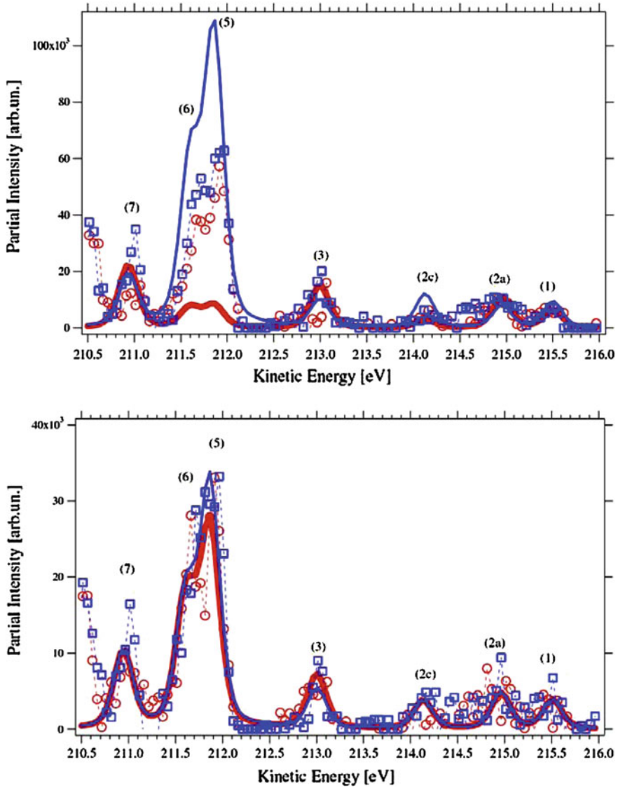
Fig. 3.12 (top) TSP and (bottom) DSP of the \text{Ar}^*2p_{1/2}^{-1}3d_{3/2}J=1 Auger decay. Peak numbers as assigned in Tables 3.9 and 3.10. Experimental data: ( \square ) spin parallel; ( \circ ) spin anti-parallel to the direction of photon propagation. Numerical data: (blue) spin parallel, (red) spin anti-parallel. (dashed lines) to guide the eye, only (after Turri et al. 2007)
