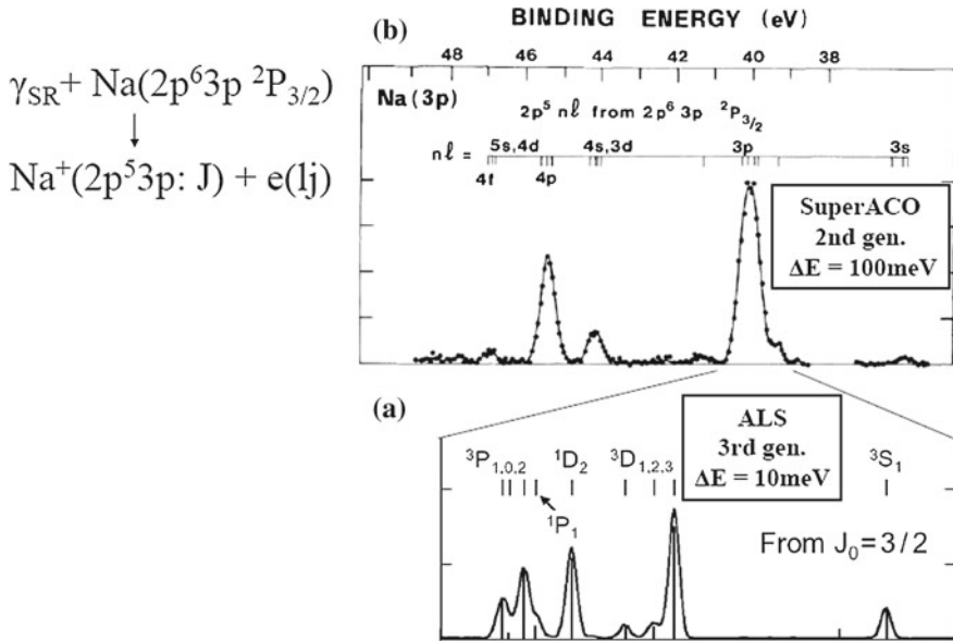
Fig. 4.23 Region of Na + (2p 5 3p) photoelectron spectra produced by photoionization from laser-excited Na*(2p 6 3p) 2 P 3/2 state measured at (a) the Advanced Light Source synchrotron radiation facility at the Lawrence Berkeley National Laboratory by Cubaynes et al. (2004) and (b) at the SuperACO synchrotron radiation facility in Orsay by Cubaynes et al. (1989). Adapted from Cubaynes et al. (2004) and Cubaynes et al. (1989)
