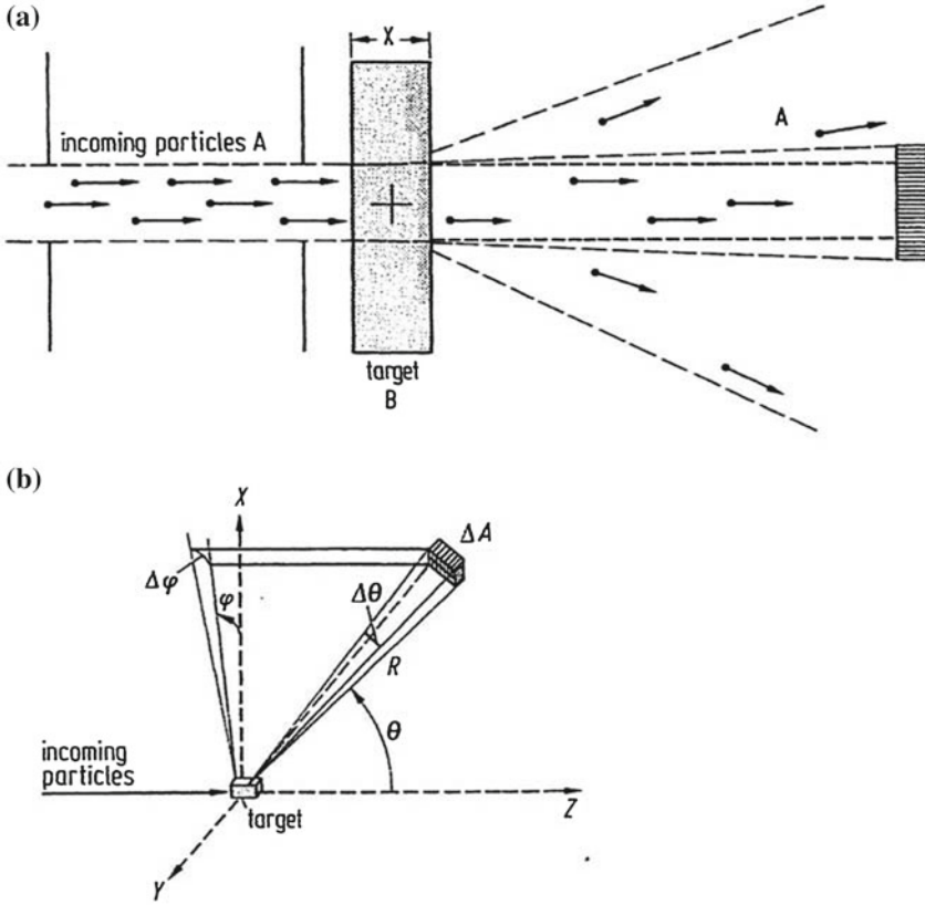
Fig. 2.2 a Scattering of particles A by the target particles B; b experimental geometry for measuring the differential cross section with the detector area \Delta A = (R \Delta\theta)(R \sin\theta \Delta\phi)
