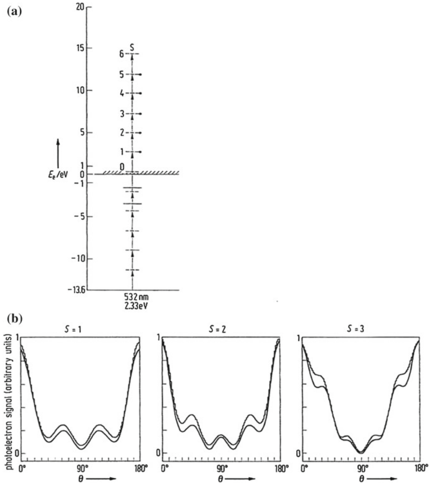
Fig. 2.12 a Multiphoton ionization of atomic hydrogen induced by laser radiation of wavelength \lambda = 532 nm; E_e photoelectron energy; the horizontal full lines represent hydrogen states, the dashed lines “virtual” in-between states. b Angular dependence of photoelectrons from the ATI peaks with the values S = 1, 2 , and 3 (see part a ) for the number of photons with energies h\nu , 2h\nu , and 3h\nu which are absorbed above the ionization threshold. The full curve corresponds to an experiment with a laser intensity of I = 1.3 \times 10^{13} \text{ W cm}^{-2} , the step-like curve is for a laser intensity of I = 1.6 \times 10^{13} \text{ W cm}^{-2} (after Wolff et al. 1988)
