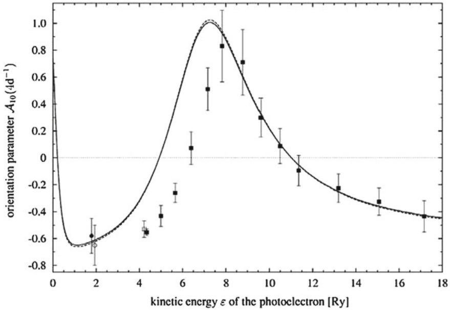
Fig. 3.20 Orientation parameter \mathcal{A}_{10} of xenon after photoionization of the inner 4d shell as a function of the kinetic energy \varepsilon of the photoelectron; numerical results: (—) 4d 3/2 and (---) 4d 5/2 HFR calculation (Kleiman and Lohmann 2003); experimental data: (●) 4d 3/2 and (○) 4d 5/2 (Snell et al. 1999a, b), (■) 4d mean value (Snell et al. 2002), (□) 4d 5/2 Schmidtke et al. (2000b); after Kleiman and Lohmann (2003)
