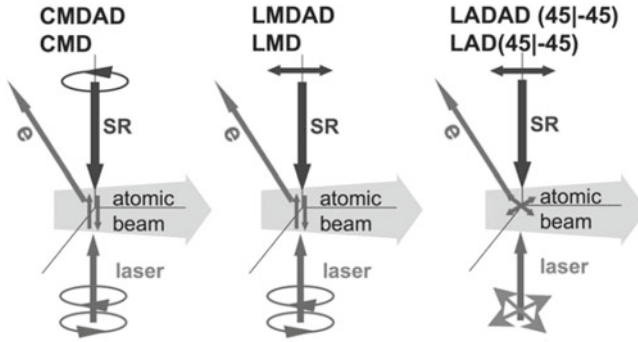
Fig. 4.24 Different kinds of magnetic dichroism in photoemission as studied in processes with collinear laser and synchrotron beams (SR). Circular or linear polarization of the SR is indicated in each panel, as well as two orthogonal polarizations of the laser light with the two corresponding directions of target polarization in the atomic beam. ( Left ) circular magnetic dichroism in the angular distribution of photoelectrons (CMDAD), which after integrating over the photoemission angle gives circular magnetic dichroism (CMD). ( Center ): linear magnetic dichroism in the angular distribution of photoelectrons (LMDAD) and linear magnetic dichroism (LMD). ( Right ) linear alignment dichroism in the angular distribution of photoelectrons (LADAD) and linear alignment dichroism (LAD); the two numbers in parenthesis indicate the angles of the linear laser polarization with respect to the linear SR polarization. After Grum-Grzhimailo and Meyer (2009)
