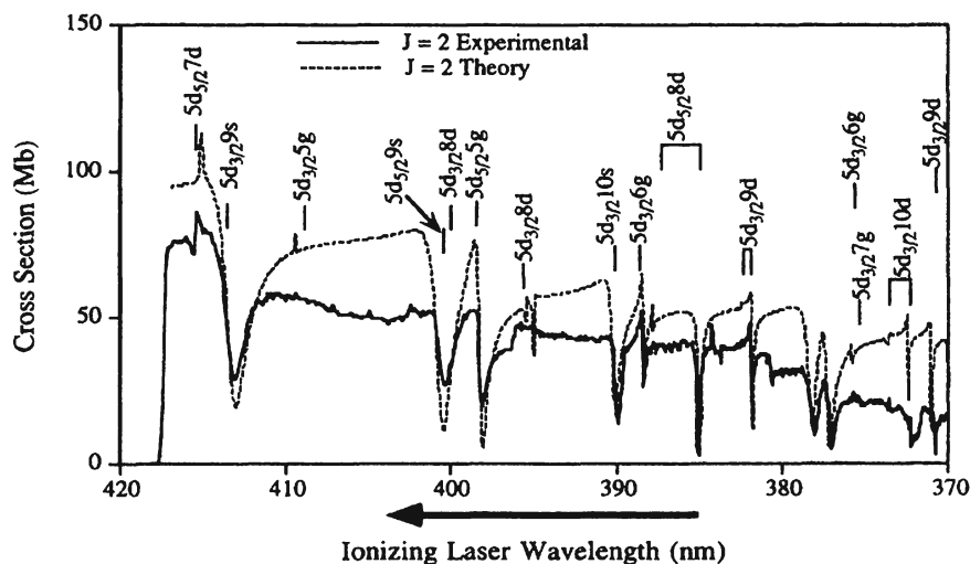
Fig. 4.33 Isotropic cross section, \sigma_2 , for photoionization of \text{Ba}^*(6s6p\ ^1P_1) to J = 2 states versus the ionizing laser beam wavelength. (—): measured spectrum; (---): theoretical spectrum of Greene and Aymar (1991) convoluted with the experimentally determined laser beam profile to account for the bandwidth. The positions and designations of some autoionizing resonances taken from Camus et al. (1983) are indicated. After He et al. (1995)
