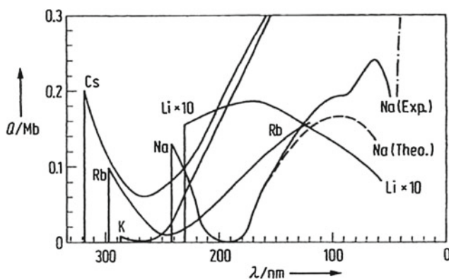
Fig. 2.16 Experimental photoionization cross sections Q of alkali atoms as a function of the wavelength \lambda (after Samson 1982); the dashed line represents calculations based on the many-body perturbation theory by Chang (1972)
