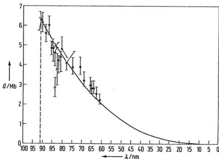
Fig. 2.13 Cross section Q of the photoionization of atomic hydrogen as a function of the wavelength \lambda . (—) theory based upon dipole approximation; (○) experimental data point with the value Q(\lambda = 85.06 \text{ nm}) = (5.15 \pm 0.18) \text{ Mb} ( \text{Mb} = \text{megabarn} = 10^{-18} \text{ cm}^2 ) after Beynon and Cairns (1965); (×) two experimental data points after Beynon (1966); (●) experimental data after Palenius et al. (1976)
