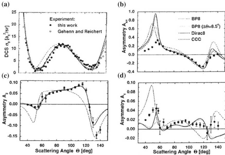
Fig. 2.62 a Differential cross section \sigma_0 for scattering of electrons by cesium atoms (normalized to theory at \theta = 90^\circ , impact energy of 3 eV); (●) Baum et al. (1986); (○) Gehenn and Reichert (1977); b the asymmetries A_{nn} , c A_2 , and d A_1 are compared to theoretical predictions: Breit-Pauli R-matrix approaches BP8 (including after convolution with the experimental angular resolution of \Delta\theta = 8.5^\circ ), a relativistic Dirac 8-state R-matrix model (Dirac 8) and a non-relativistic convergent close-coupling calculation (CCC). Many more such data for projectile energies from 5 to 25 eV by Baum et al. (2002) have been published
