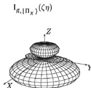
Fig. 3.35 Angular distribution of the emitted Auger electrons from axis-fixed CO molecules (continued). Labels d and f refer to Table 3.17; after Bonhoff et al. (1999). See Fig. 3.34 for explanations
