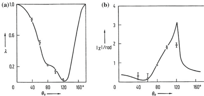
Fig. 2.38 \lambda - and |\chi| -data of the He(2 1 P)-excitation by electron impact in dependence of the electron scattering angle \theta_e at an electron of 24 eV; experimental data of Crowe et al. (1983); the full theoretical curve represents a 5-state R -matrix calculation of these authors
