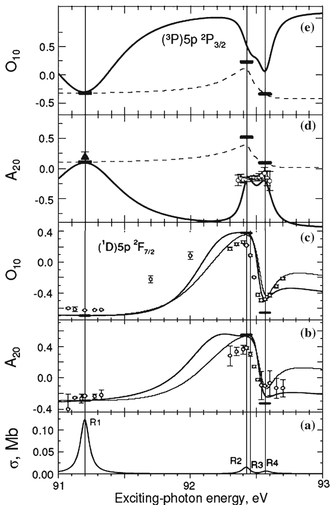
Fig. 4.46 Dependence of the alignment and orientation parameters on the excitation energy in the region of the Kr J = 1 Auger states: 4d_{5/2}^{-1}5p_{3/2} (R1), 4d_{5/2}^{-1}6p_{3/2} (R4), and perceptible mixtures of the 4d_{5/2}^{-1}5p_{1/2,3/2} states (R2, R3). (○): experimental data by Lagutin et al. (2003) and Schartner et al. (2005). Horizontal bars with lengths equal to the natural widths (the resonance R3 is negligible) indicate parameters computed within the two-step model for an isolated resonance. a calculated cross section; b and c thin lines, calculations neglecting interference between the resonances and between the resonant and direct amplitudes; thick lines, calculations accounting for the interference terms. d and e calculations with (—), and without (---) direct photoionization amplitude, respectively. Adapted from Schartner et al. (2005)
