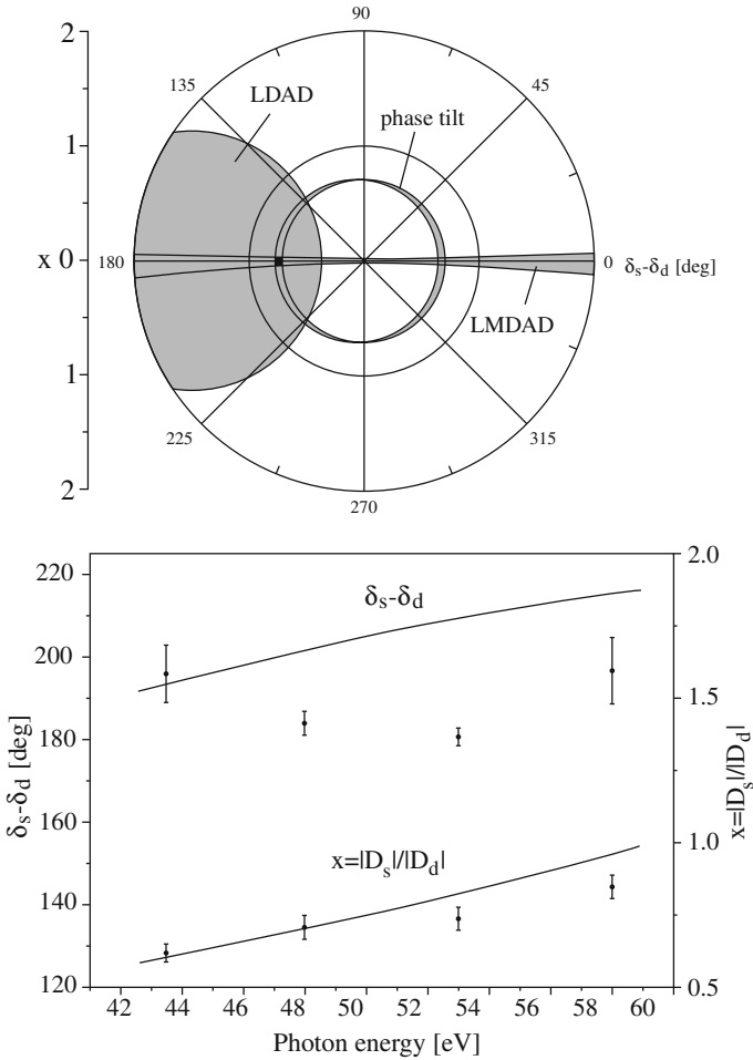
Fig. 4.25 Absolute ratio x = |D_s|/|D_d| of the dipole amplitudes and phase difference ( \delta_s - \delta_d ) for the outgoing electron waves \varepsilon_s, \varepsilon_d in the 5p photoionization of Eu. (Top) polar plot of the different sets of values derived from measurements of LADAD, LMDAD, and phase tilt at h\nu = 53 eV. The area where all three sets intersect is the black square. The cross is the theoretical result obtained using the Cowan code. (Bottom) energy dependence of the extracted parameters together with theoretical results obtained using the Cowan code. The data were obtained with a cylindrical mirror analyzer, which partly integrates the photoelectron flux over the azimuthal angle. Adapted from Godehusen et al. (1998)
