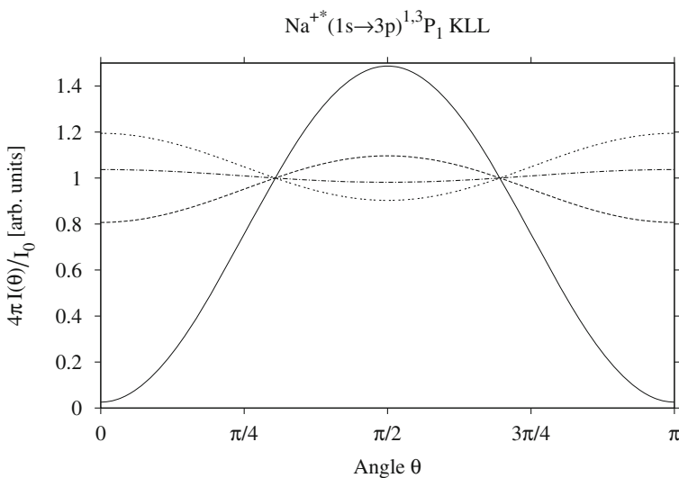
Fig. 3.7 The angular distribution of the emitted Auger electrons for selected Auger transitions of the excited \text{Na}^{+*}(1s^{-1} \rightarrow 3p)^{1,3}P_1 KLL Auger decay. Utilizing the photoionization/excitation process as per (3.37) and (3.38) an alignment of \mathcal{A}_{20} = 1/\sqrt{2} has been assumed. The angular distribution data for the anisotropy coefficient have been taken from Table 3.8. The Auger transitions are depicted as follows; (—): ^1P \rightarrow ^2S ; (---): ^3P \rightarrow ^2P ; (- · - · -): ^3P \rightarrow ^2D ; (· · · · ·): ^3P \rightarrow ^2P^\circ
