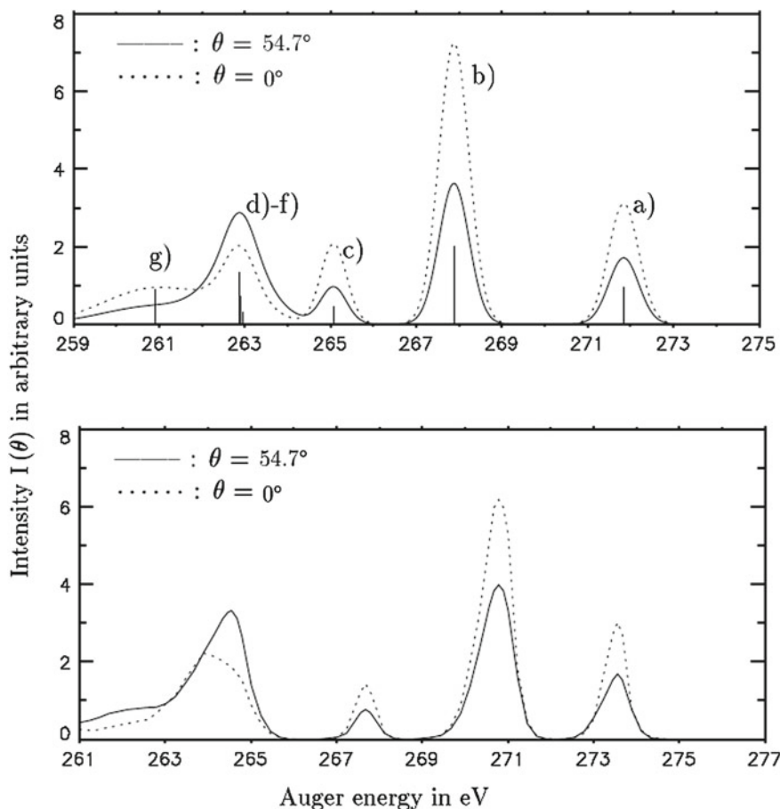
Fig. 3.33 Auger spectrum for the transitions of the (2\sigma^{-1}2\pi^1)^1\Pi vacancy of CO created by absorption of linearly polarized photons. (Top) calculated spectrum (Bonhoff et al. 1999), the labels refer to Table 3.17. (Bottom) experimental spectrum by Hemmers et al. (1993)
