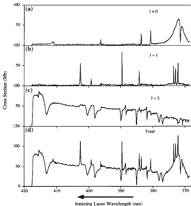
Fig. 4.32 a–c Cross sections for photoionization of \text{Ba}^*(6s6p\ ^1P_1) to specific final J states. d total isotropic photoionization cross section of \text{Ba}^*(6s6p\ ^1P_1) . After He et al. (1995)
