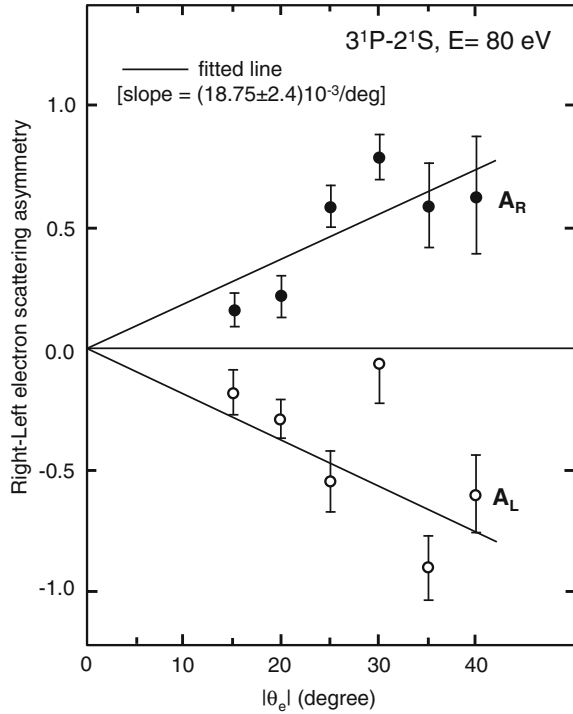
Fig. 2.52 Right-left electron scattering asymmetry as a function of the scattering angle for detecting right (●) or left (○) hand circularly coincident polarized photons of the helium transition 3^1P_1 \rightarrow 2^1S_0 at 80 eV. The full lines are fitted to the experimental data (Silim 1985)
