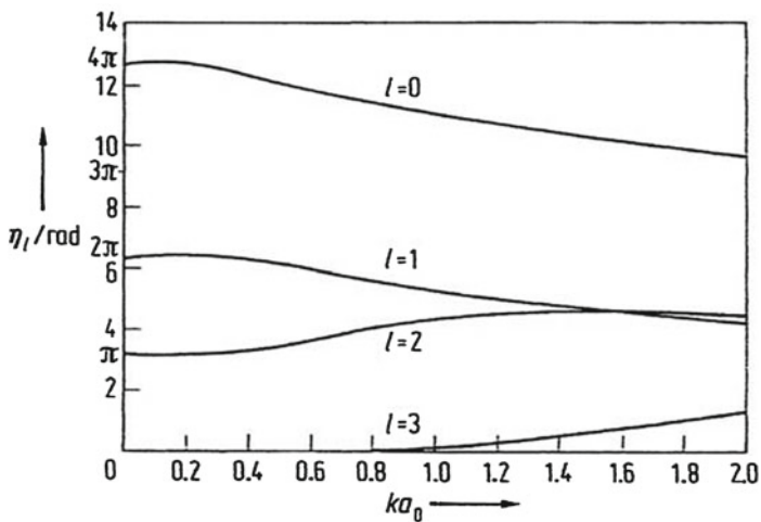
Fig. 2.18 Calibrated scattering phases \eta_\ell for \ell = 0, 1, 2 , and 3 of elastic scattering on krypton. \eta_0 tends to 4\pi at zero energy. The unit of the abscissa (ka_0)^2 = 1 corresponds to an energy of 13.6 eV of the incident electrons (Holtmark 1930)
