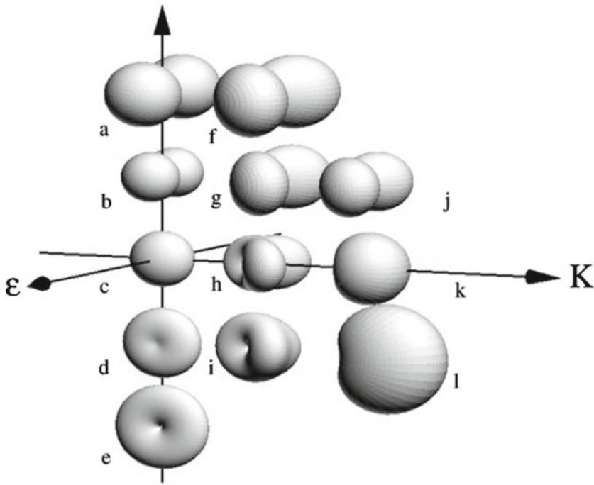
Fig. 4.48 Angular distribution patterns for different values of \beta , \gamma , and \delta ; see (4.109). K is the direction of the incoming photon beam, while \varepsilon denotes the axis of its linear polarization. The patterns show the photoelectron emission probability as a function of the emission angle. (a): \beta = 2 and \gamma = \delta = 0 ; (b): \beta = 1 and \gamma = \delta = 0 ; (c): \beta = \gamma = \delta = 0 ; (d): \beta = -0.5 and \gamma = \delta = 0 ; (e): \beta = -1 and \gamma = \delta = 0 ; (f): \beta = 2 , \gamma = 3 , and \delta = 0 ; (g): \beta = 1 , \gamma = 3.52 , and \delta = 0 ; (h): \beta = 0 , \gamma = \sqrt{27/4} , and \delta = 0 ; (i): \beta = -0.5 , \gamma = 1.81 , and \delta = 0 ; (j): \beta = 1 , \gamma = 1.75 , and \delta = 0.5 ; (k): \beta = 0 , \gamma = 0.5 , and \delta = 1 ; (l): \beta = -0.5 , \gamma = 0 , and \delta = \sqrt{27/4} . After Hemmers et al. (2004)
