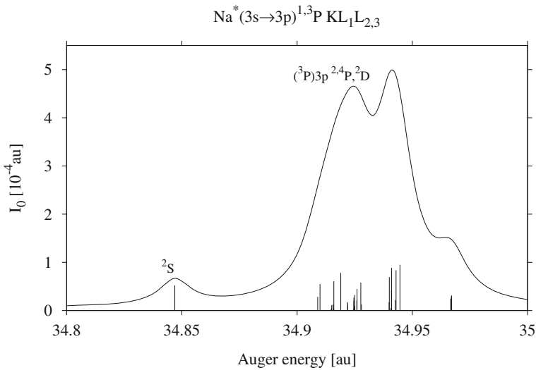
Fig. 3.6 The multiple splitting of the low intensity 2s, 2p^5(^3\text{P})^2,4\text{L}_J Auger lines, stemming from the laser excited 3s \rightarrow 3p Na \text{KL}_1\text{L}_{2,3}(^3\text{P})3p Auger transitions
