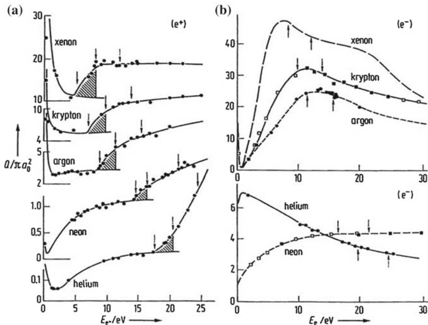
Fig. 2.20 a Total cross sections Q of low energy positron scattering on rare gas atoms as a function of the positron energy E_{e+} ; the three arrows indicate the onset of the formation of positronium, the first inelastic excitation and the ionization of the atoms. The hatched areas represent an estimation for the cross section of the positronium formation, the subtraction of which results in the total elastic cross section (lower part of the hatched area); b total cross sections for the scattering of electrons on rare gas atoms as a function of the electron energy E_e ; the two arrows on each curve indicate the onset of the first inelastic excitation and the ionization of the atoms (after Kauppila and Stein 1982)
