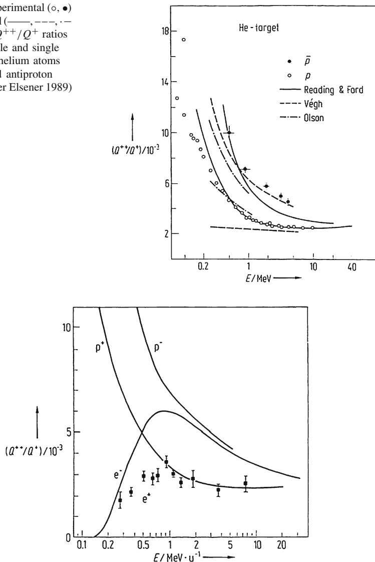
Fig. 2.87 Q^{++}/Q^+ data for helium atoms as target with protons and anti-protons as projectiles. The full curves represent experimental data for electrons ( e^- ), protons ( p^+ ), and anti-protons ( p^- ) while the data ( \blacksquare ) are the positron ratios R_{e^+} = Q^{++}/Q^+ according to measurements of Charlton et al. (1988) ( 1u = \frac{1}{12}m(^{12}\text{C}) )
