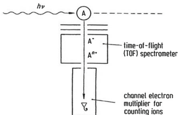
Fig. 2.4 Ion charge analysis by means of a time-of-flight (TOF) spectrometer and ion detection by a channel electron multiplier
