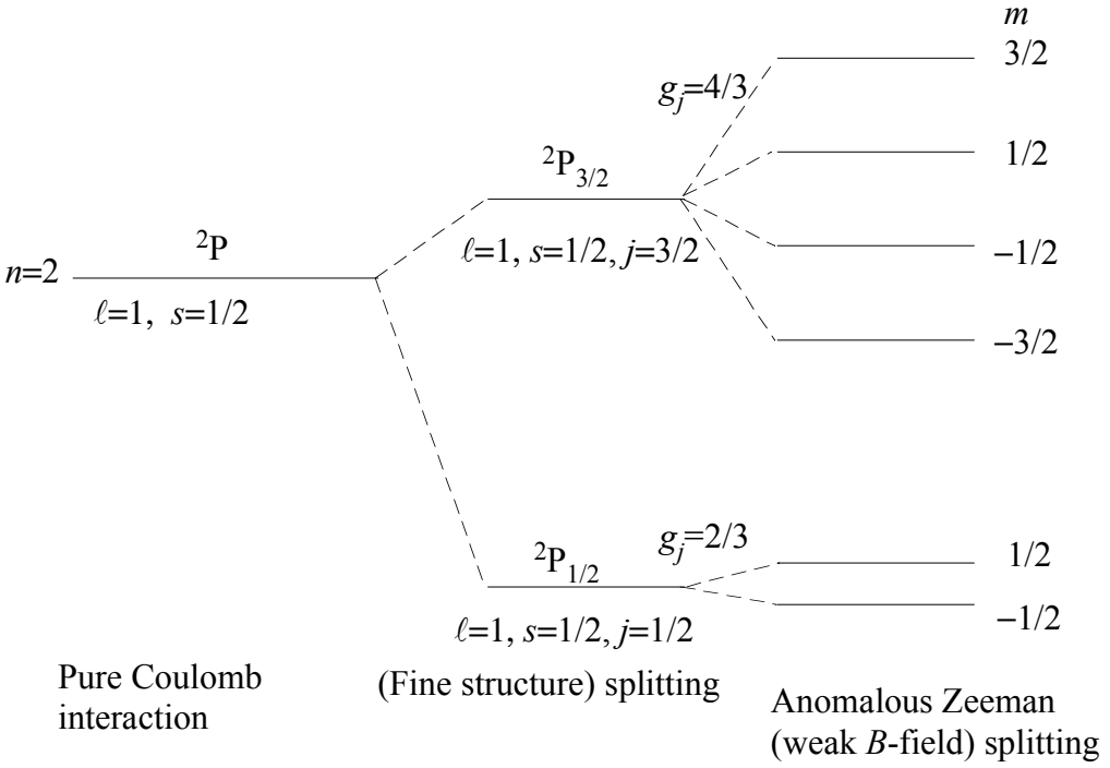
FIGURE 8.3 Weak B -field (anomalous) Zeeman splitting for {}^2P ( n = 2, \ell = 1 ) level in hydrogen.
