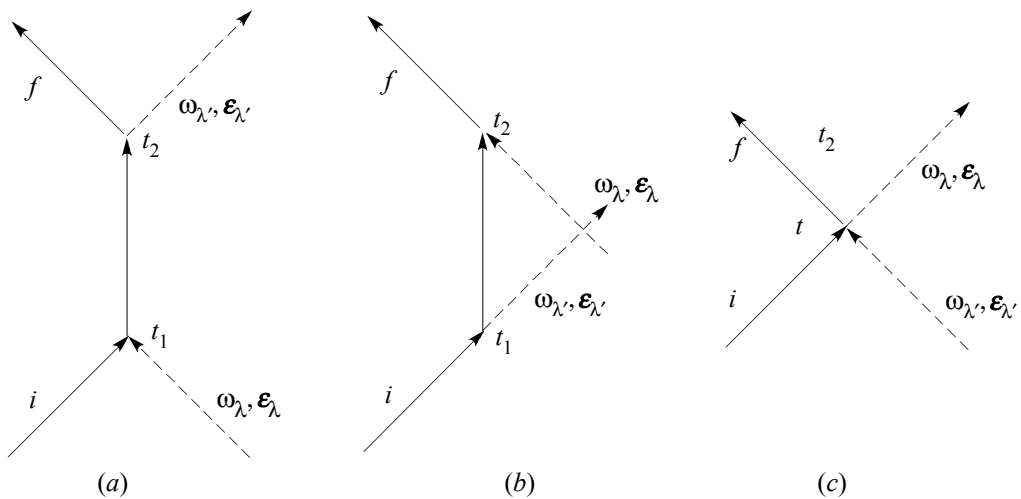
FIGURE 13.2 Figures (a) and (b) represent annihilation and creation (or creation and annihilation) of a photon in succession. Figure (c) indicates this as a one step process.
