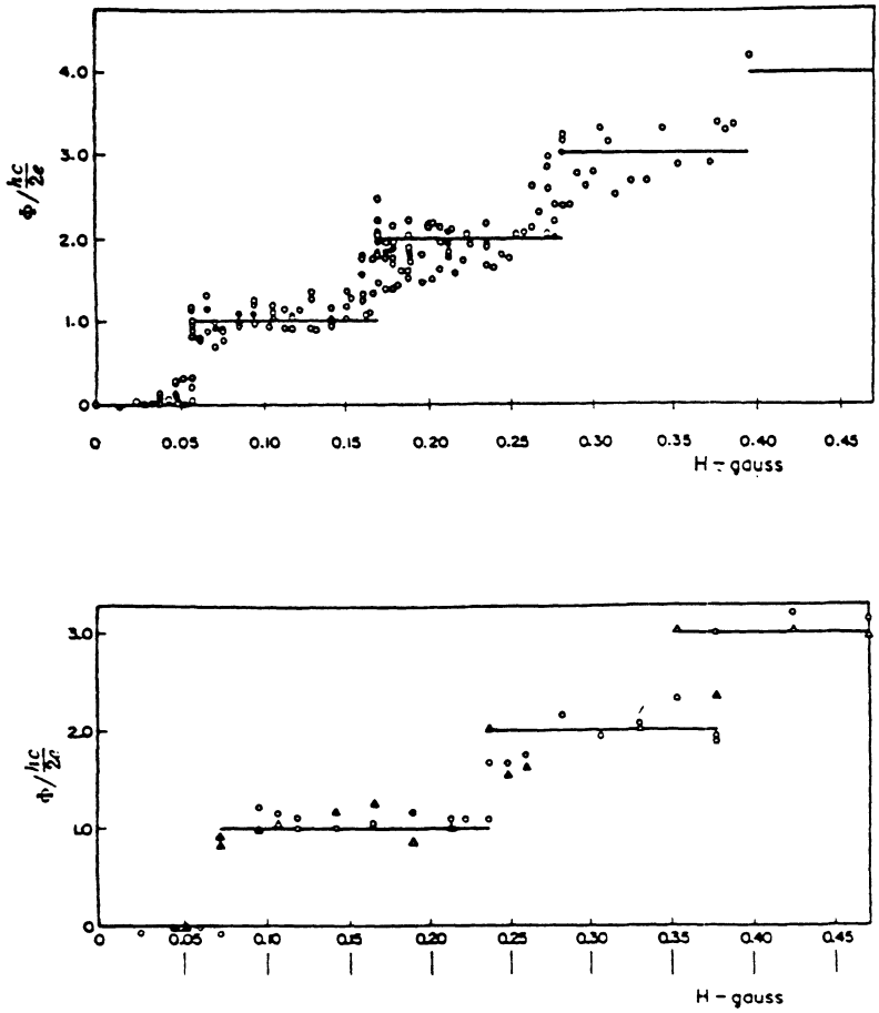
Figure1: Flux quantization in two small tubular superconducting samples according to Deaver and Fairbank (ref.11). The ordinate shows the trapped flux in MKS units h/2e as a function of the external field in which the cylindrical rings have been cooled below the transition temperature. Note absence of residual flux!
