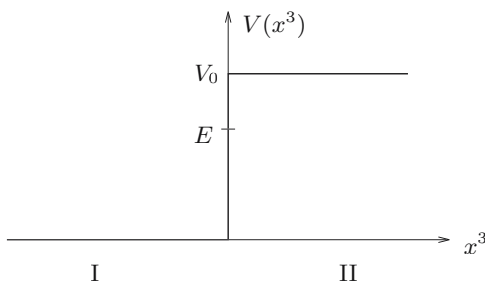
Fig. 10.1. A potential step of height V_0
