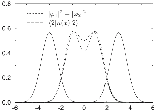
Fig. 3.2. Densities for two-boson states. The full line is the case a = 3 . Since there is no overlap here, |\varphi_1|^2 + |\varphi_2|^2 and \langle n(\mathbf{x}) \rangle are indistinguishable from one another. The dashed lines are for a = 1 : in this case \langle 2 | n(\mathbf{x}) | 2 \rangle is increased at small separations in comparison to \varphi_1^2 + \varphi_2^2
