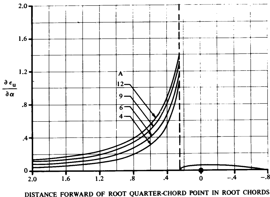
Fig. 16.11 Upwash estimation (subsonic only). (Ref. 37)
