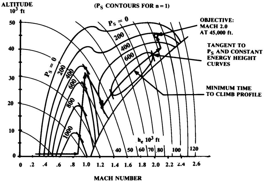
Fig. 17.14 Minimum time-to-climb, low thrust fighter (circa 1960).
