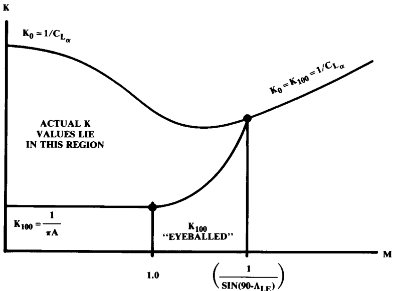
Fig. 12.34 0% and 100% K vs Mach number.
