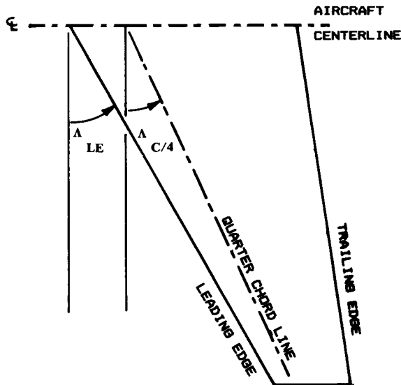
Fig. 4.16 Wing sweep Λ.
