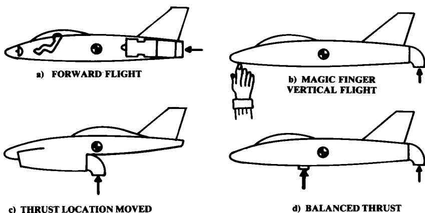
Fig. 20.1 The balance problem.
