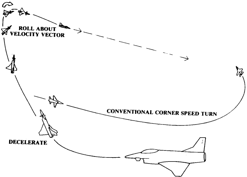
Fig. 17.28 X-31 Supermaneuver.
