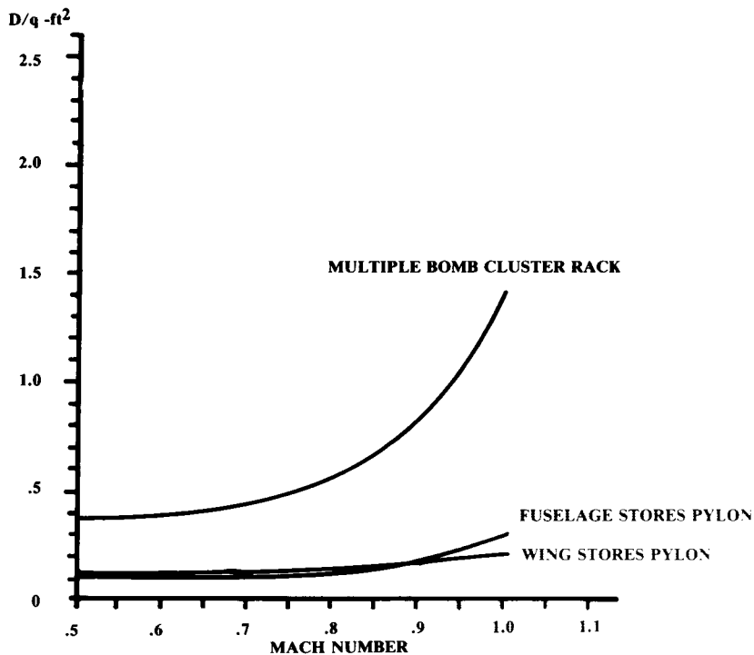
Fig. 12.23 Pylon and bomb rack drag.
