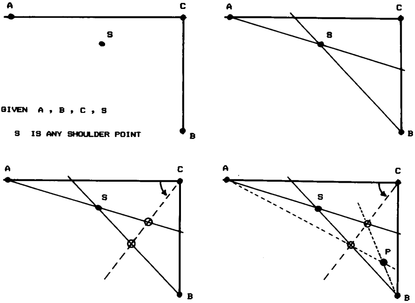
Fig. 7.11 Conic layout.
