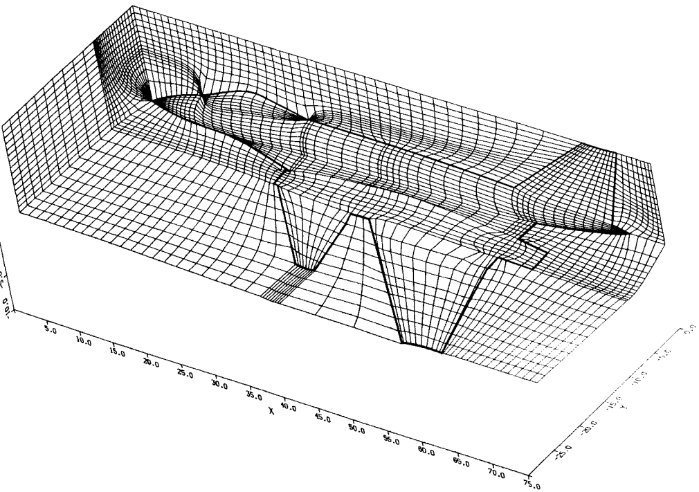
Fig. 12.40 Flowfield gridding. (Ref. 82)
