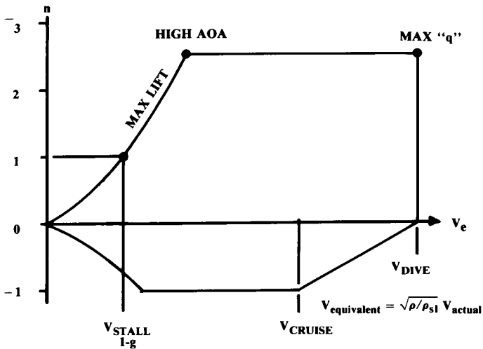
Fig. 14.3 V-n diagram (maneuver).
