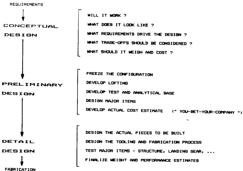
Fig. 2.2 Three phases of aircraft design.
