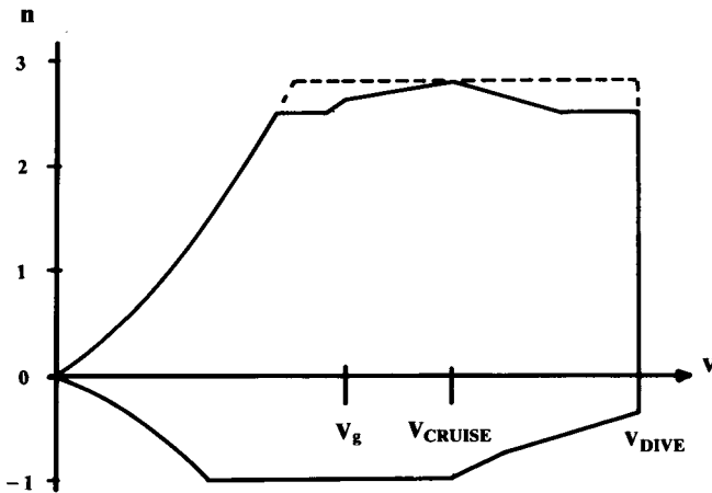
Fig. 14.8 Combined V-n diagram.
