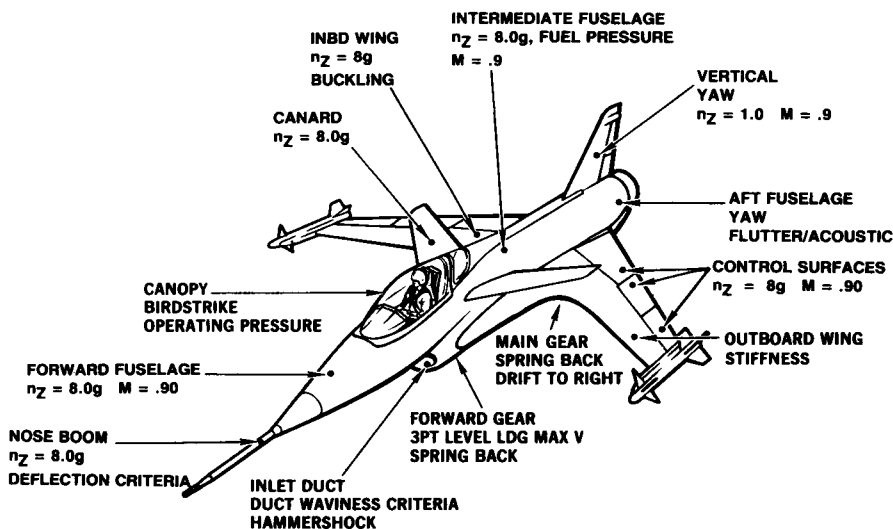
Fig. 14.1 Typical fighter limit loads.
