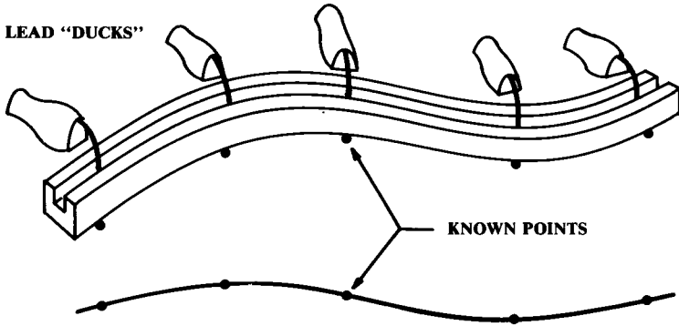
Fig. 7.9 Spline lofting.
