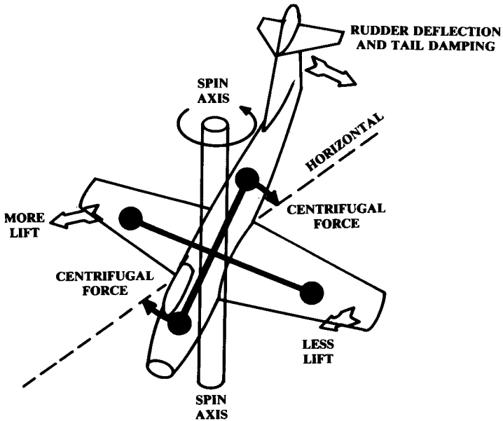
Fig. 16.29 Forces in spin.
