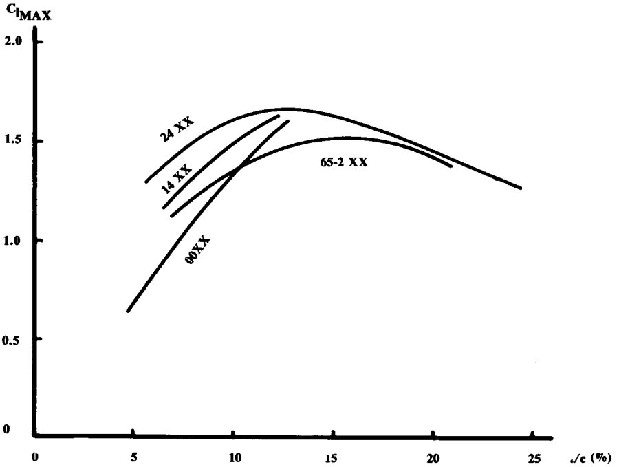
Fig. 4.13 Effect of t/c on maximum lift.
