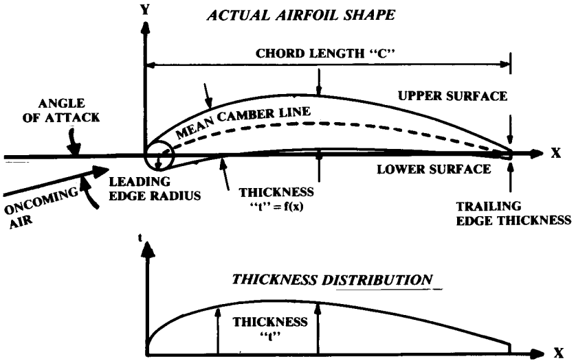
Fig. 4.1 Airfoil geometry.
