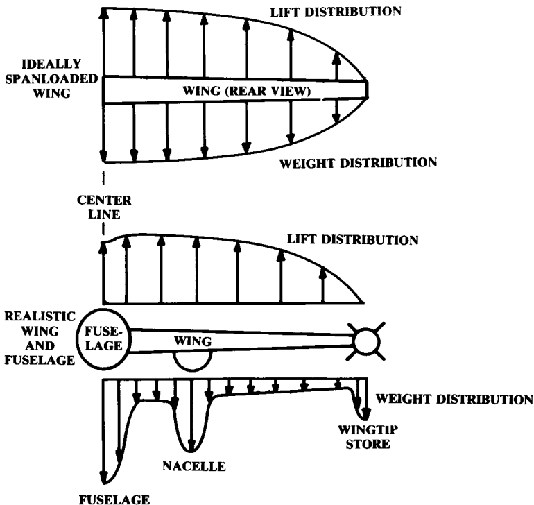
Fig. 8.4 Spanloading for weight reduction.
