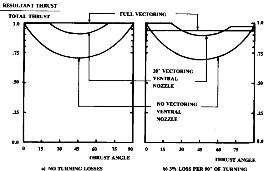
Fig. 20.9 Resultant thrust.
