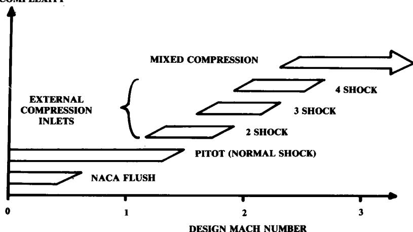
Fig. 10.10 Inlet applicability.
