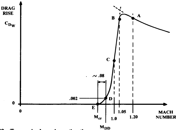
Fig. 12.29 Transonic drag rise estimation.
