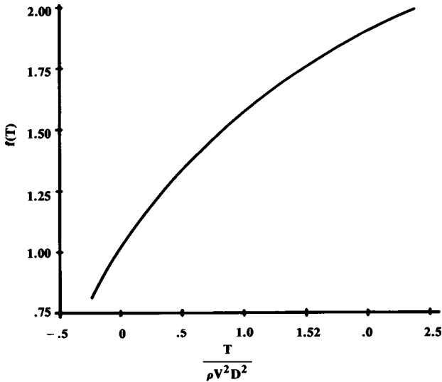
Fig. 16.16 Propeller normal force factor. (after Ref. 68)
