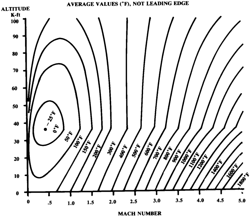
Fig. 14.22 Skin temperature estimate.
