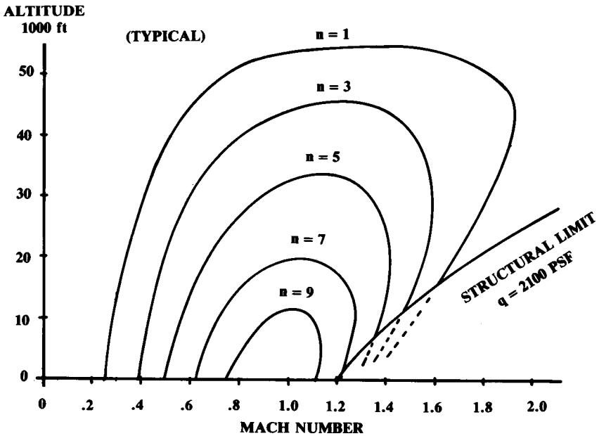
Fig. 17.10 P_s = 0 contours.
