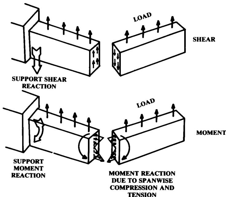
Fig. 14.37 Shear and moment in beams.
