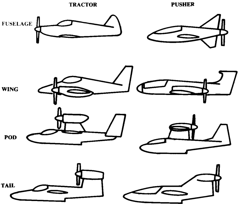
Fig. 10.21 Propeller location matrix.
