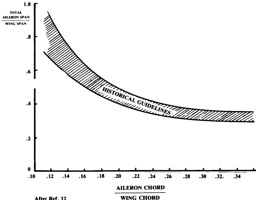
Fig. 6.3 Aileron guidelines.
