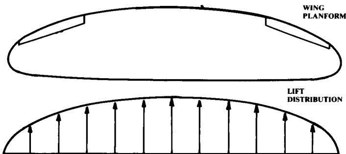
Fig. 4.21 Elliptical wing.
