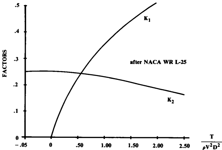
Fig. 16.17 Propeller downwash factors. (after Ref. 68)
