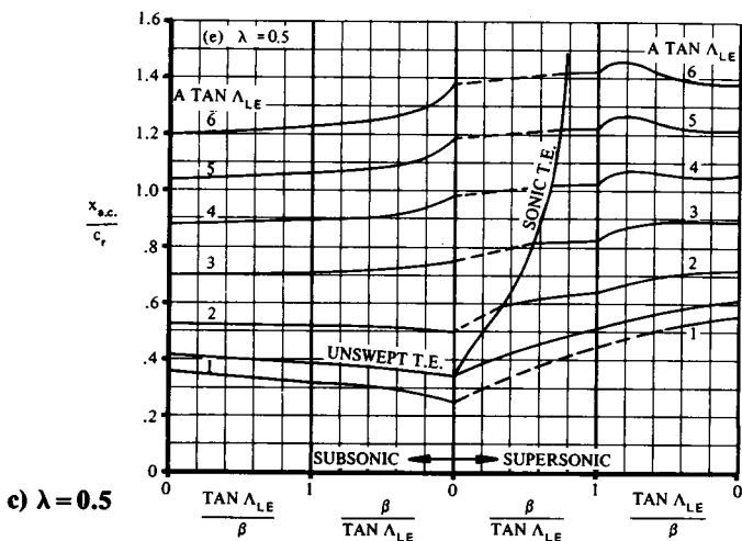
Fig. 16.5 Wing aerodynamic center. (Ref. 37)
