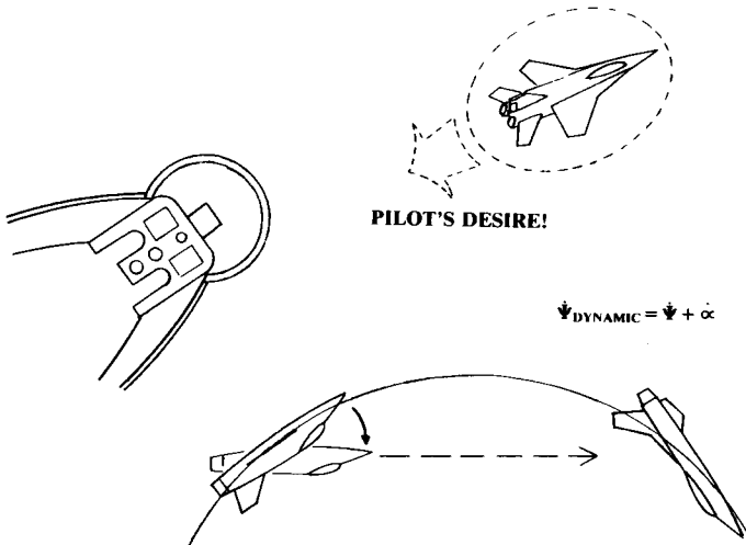
Fig. 17.25 Dynamic turn.
