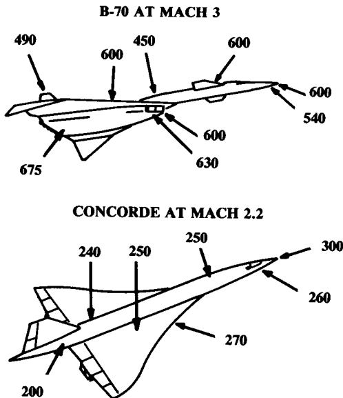
Fig. 14.21 Supersonic skin temperatures ( ^{\circ} F).
