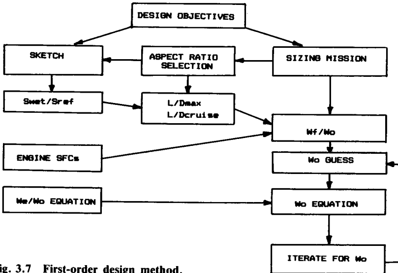
Fig. 3.7 First-order design method.
