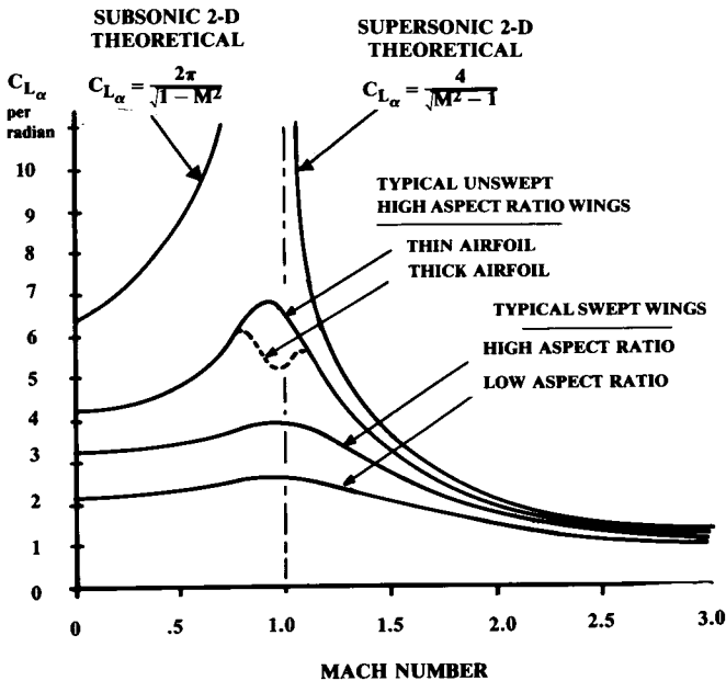
Fig. 12.5 Lift curve slope vs Mach number.
