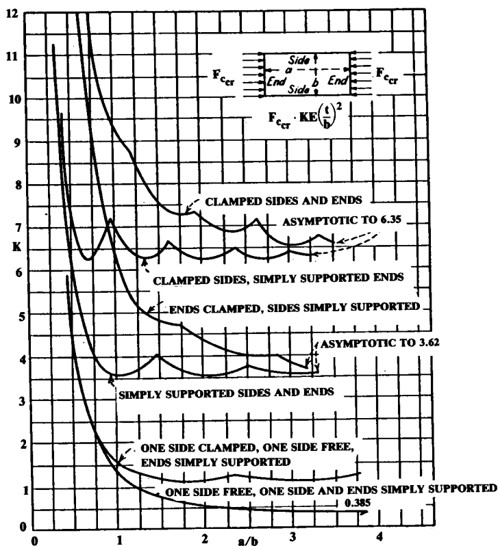
Fig. 14.33 Panel buckling coefficient. (NACA TN3781)
