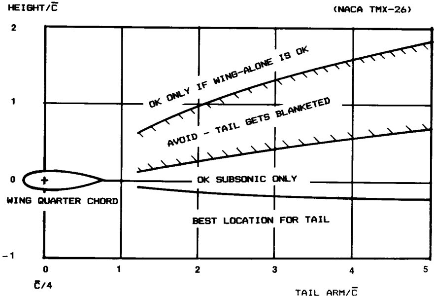
Fig. 4.29 Aft tail positioning.
