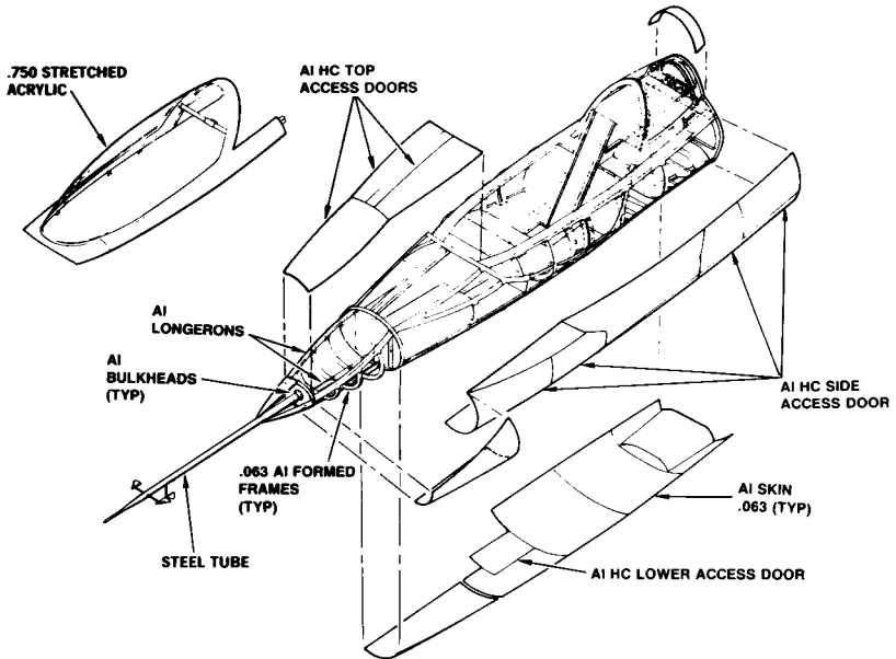
Fig. 14.23 Materials – forebody.
