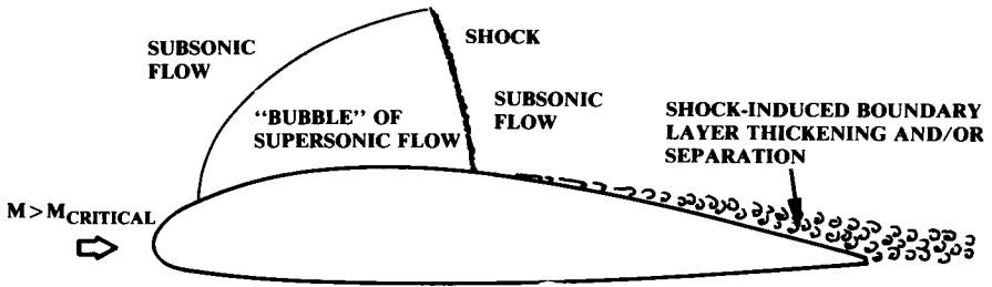
Fig. 4.8 Transonic effects.
