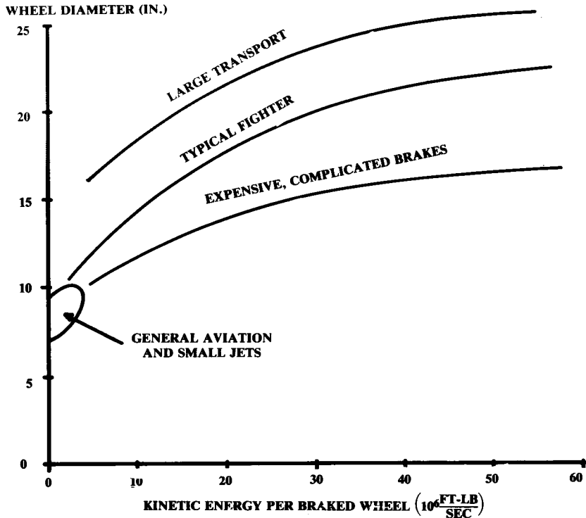
Fig. 11.7 Wheel diameter for braking.
