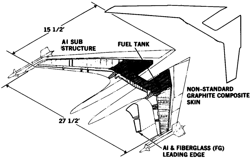
Fig. 14.25 Wing materials.
