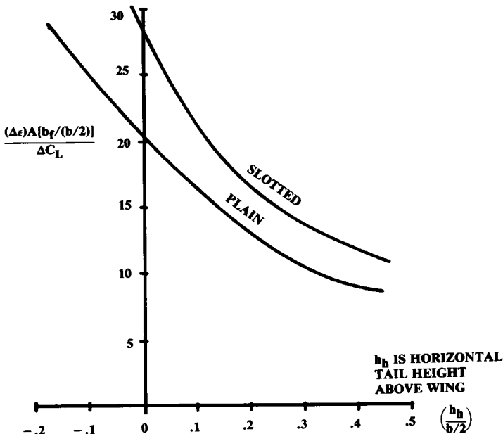
Fig. 16.13 Downwash increment due to flaps.
