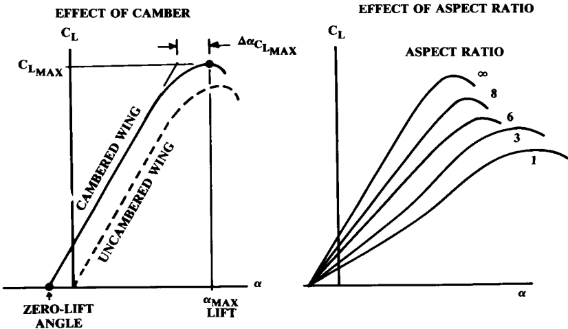
Fig. 12.4 Wing lift curve.
