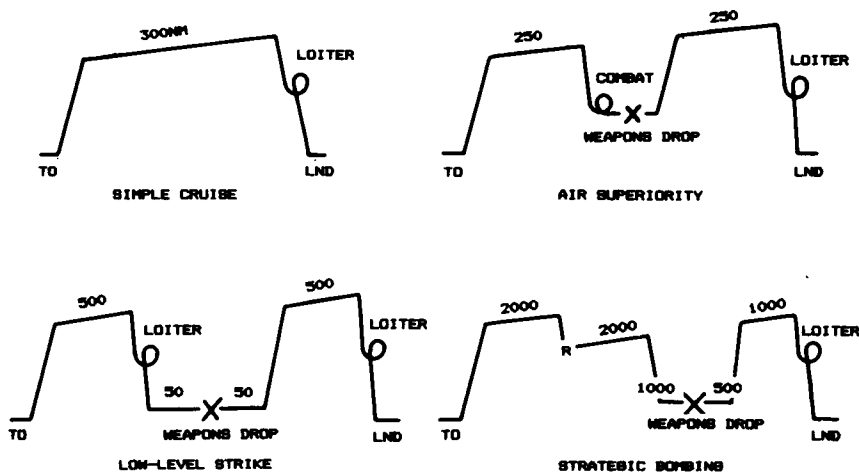
Fig. 3.2 Typical mission profiles for sizing.
