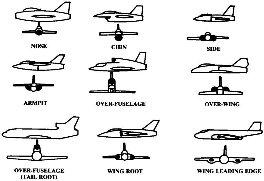
Fig. 10.11 Inlet locations—buried engines.
