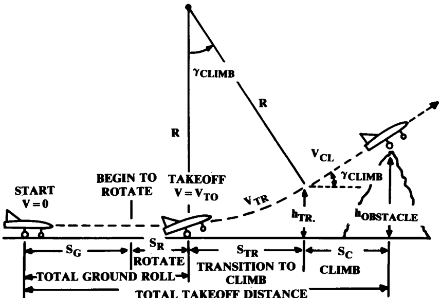
Fig. 17.17 Takeoff analysis.
