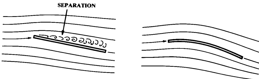
Fig. 4.4 Effect of camber on separation.
