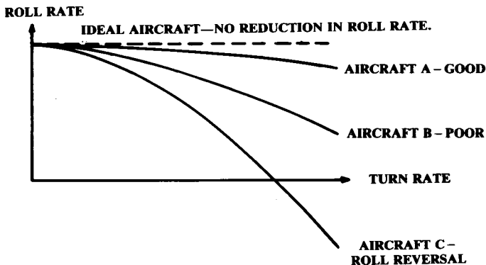
Fig. 17.20 Loaded roll comparison.
