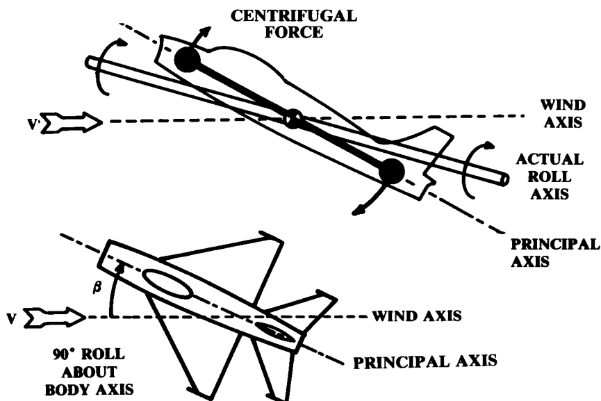
Fig. 16.26 Inertia coupling.
