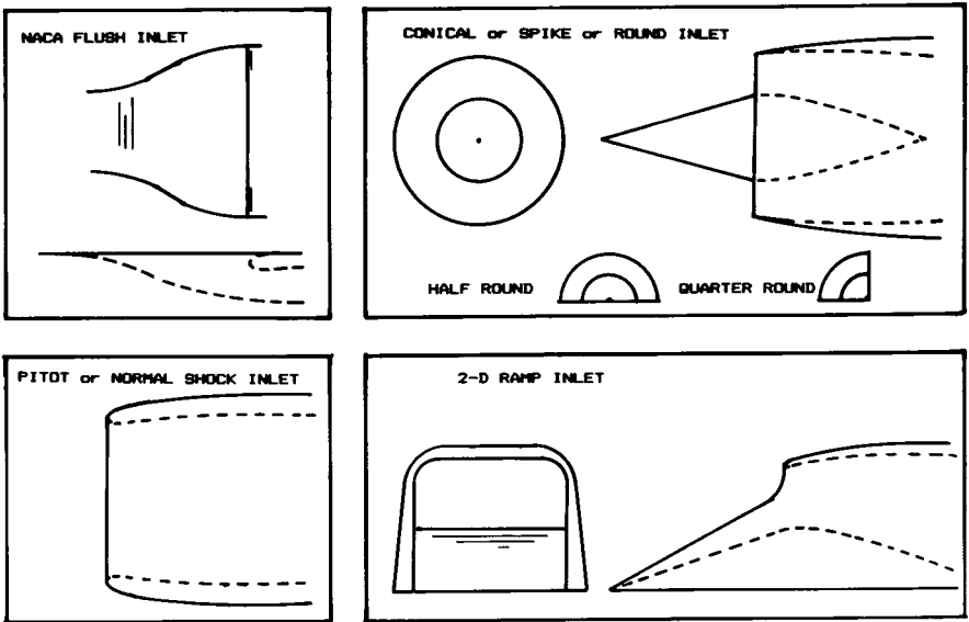
Fig. 10.4 Inlet types.
