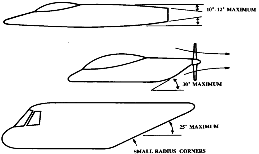
Fig. 8.1 Longitudinal contour guidelines.
