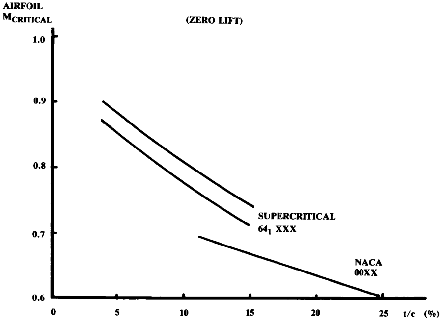
Fig. 4.12 Effect of t/c on critical mach number.
