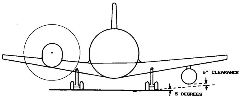
Fig. 4.26 Low wing.
