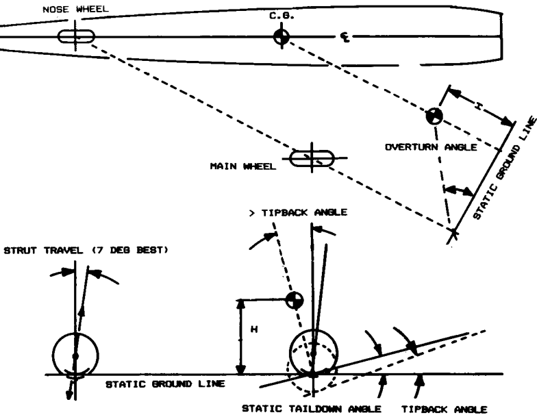
Fig. 11.4 Tricycle landing gear geometry.
