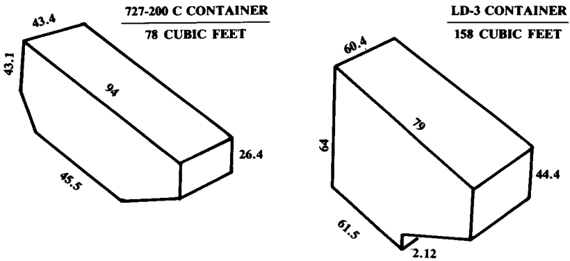
Fig. 9.4 Cargo containers.
