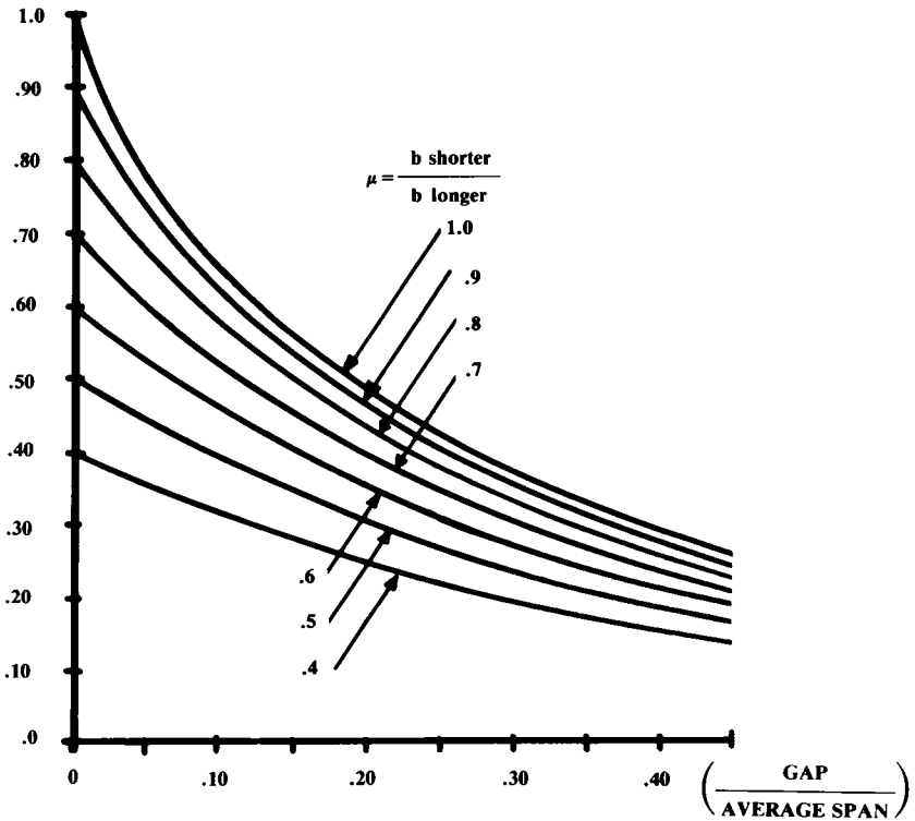
Fig. 12.32 Prandtl's biplane interference factor. (Ref. 12)
