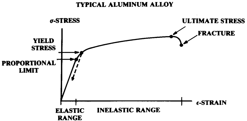
Fig. 14.17 Stress-strain diagram.
