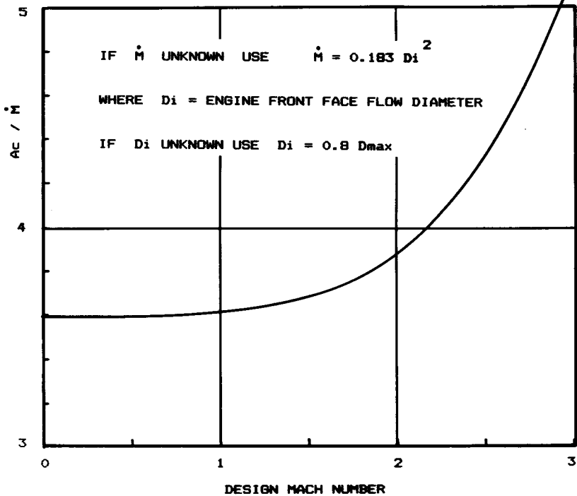
Fig. 10.13 Preliminary capture area sizing.
