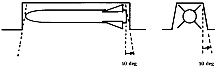
Fig. 9.7 Weapon release clearance.
