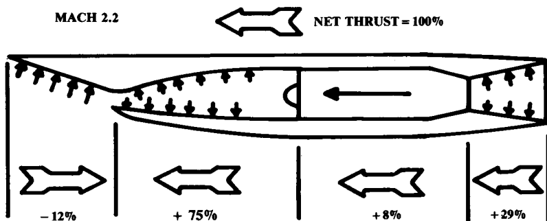
Fig. 13.1 Turbojet thrust contributors.
