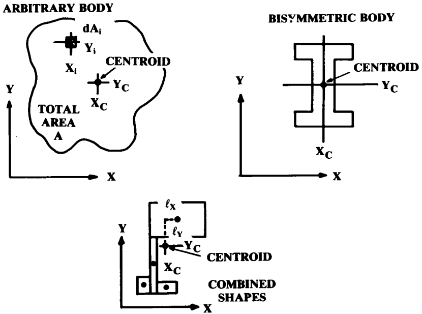
Fig. 14.30 Section property definitions.
