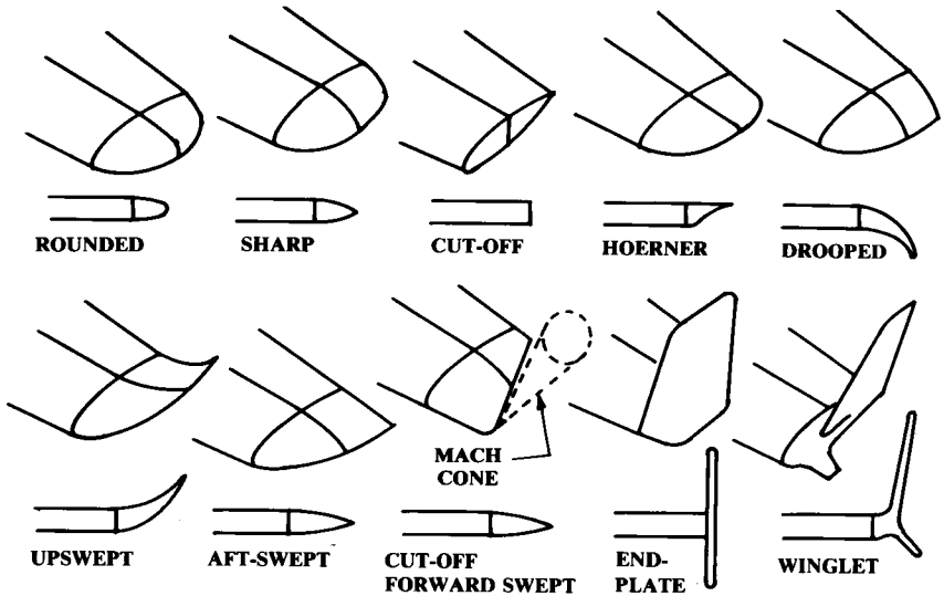
Fig. 4.27 Wing tips.
