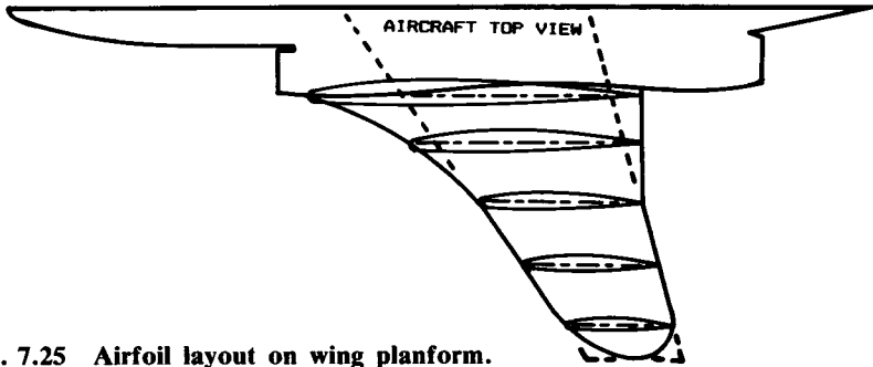
Fig. 7.25 Airfoil layout on wing platform.
