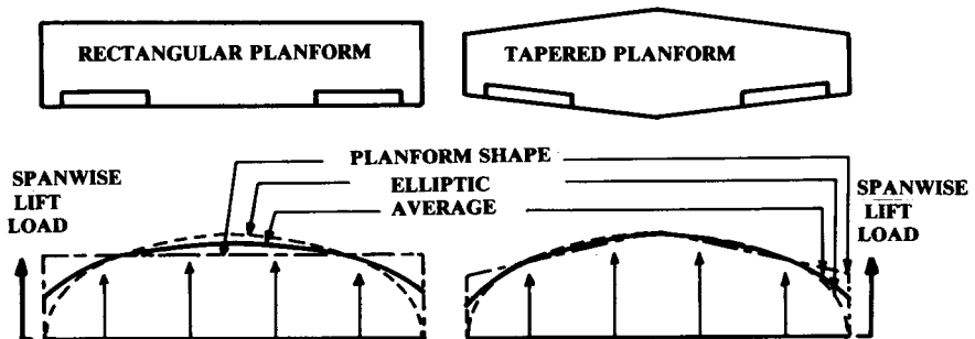
Fig. 14.10 Schrenk’s approximation.
