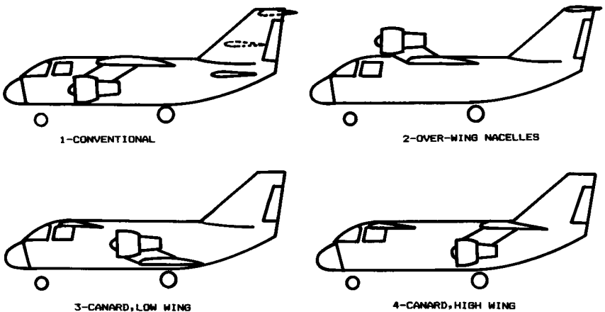
Fig. 3.9 ASW concept sketches.
