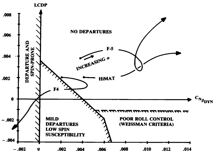
Fig. 16.28 Departure susceptibility.
