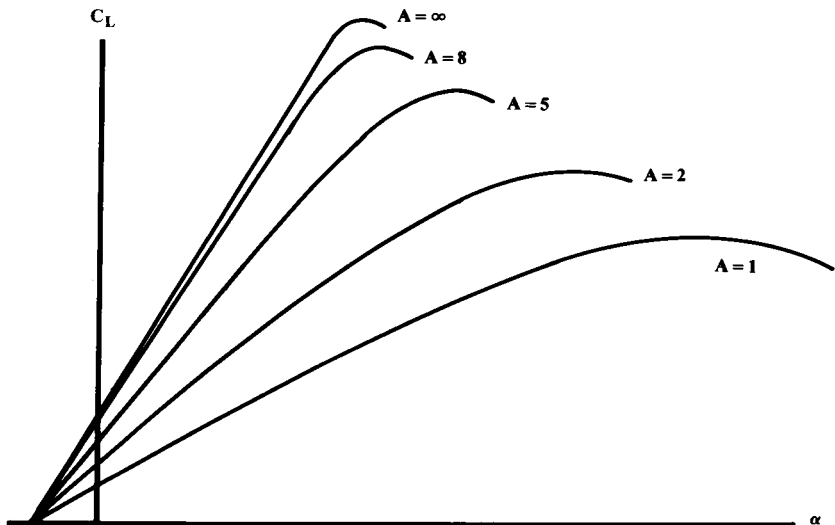
Fig. 4.18 Effect of aspect ratio on lift.
