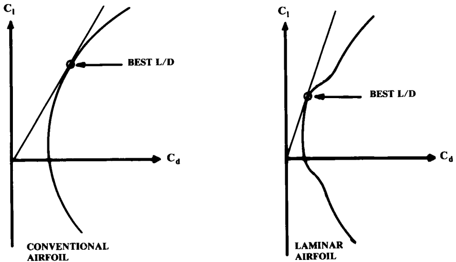
Fig. 4.9 Design lift coefficient.
