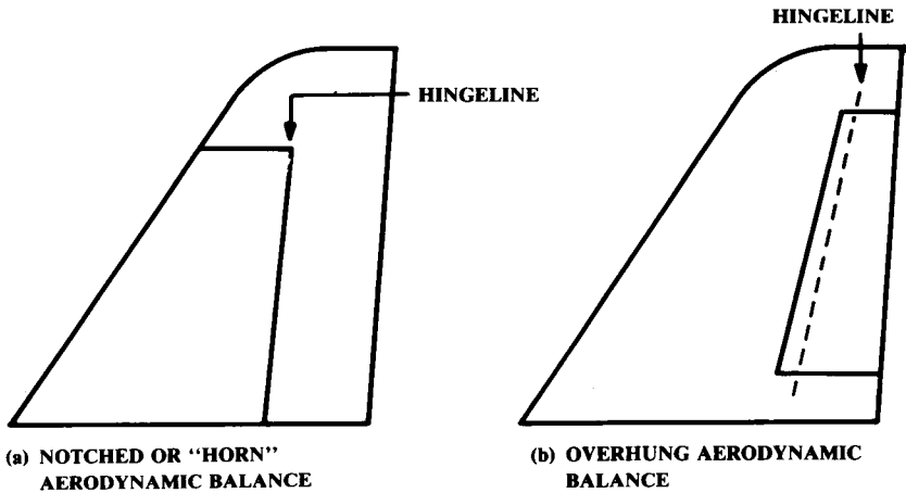
Fig. 6.5 Aerodynamic balance.
