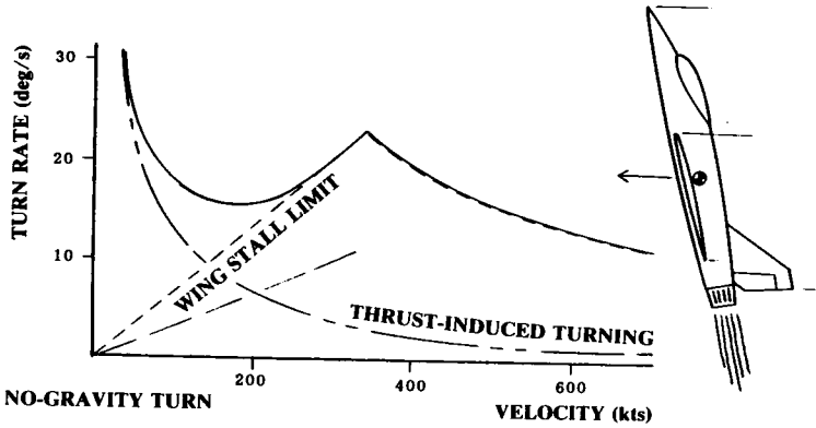
Fig. 17.24 Fuselage pointing.
