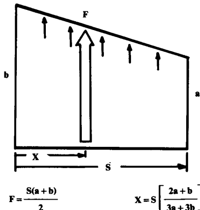
Fig. 14.39 Trapezoidal approximation for distributed loads.
