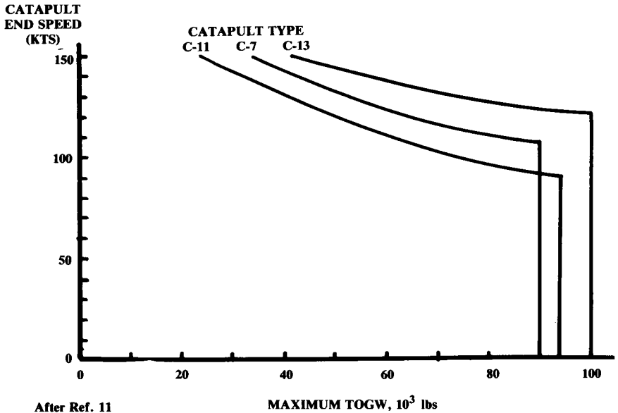
Fig. 5.5 Catapult end speeds.
