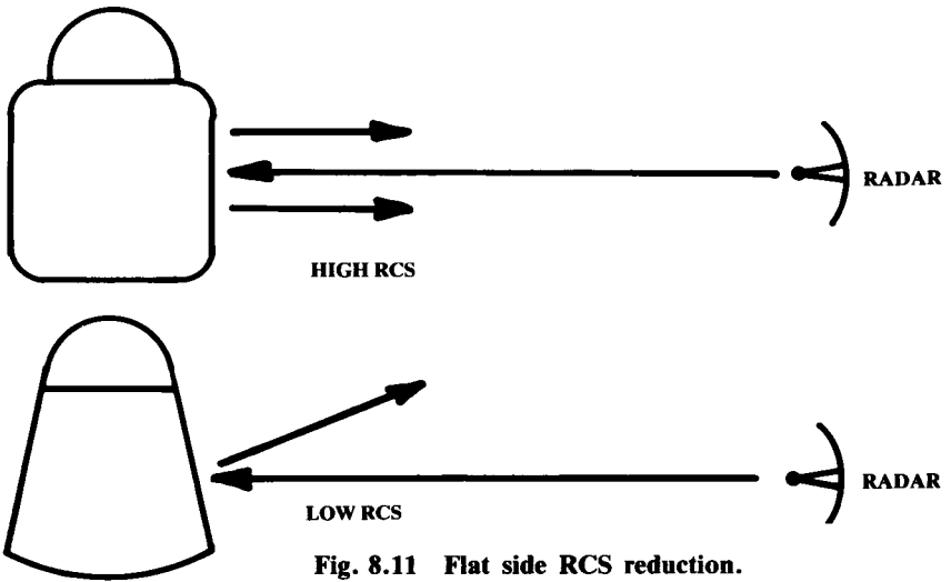
Fig. 8.11 Flat side RCS reduction.
