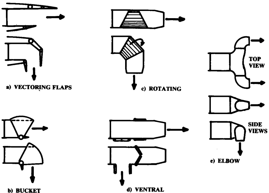
Fig. 20.8 Vectoring nozzles.
