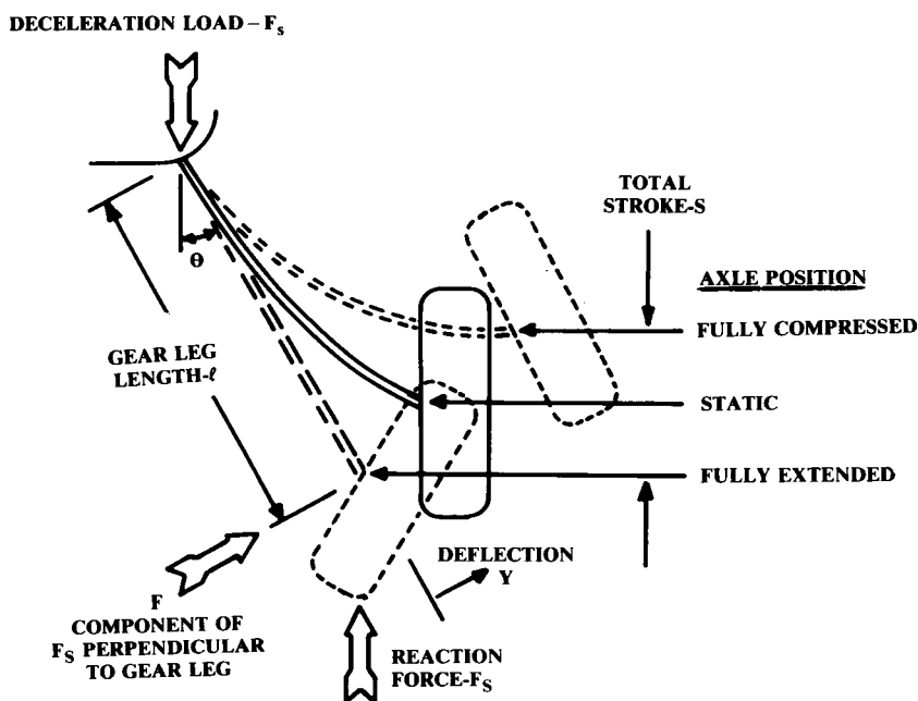
Fig. 11.10 Solid spring gear deflection.
