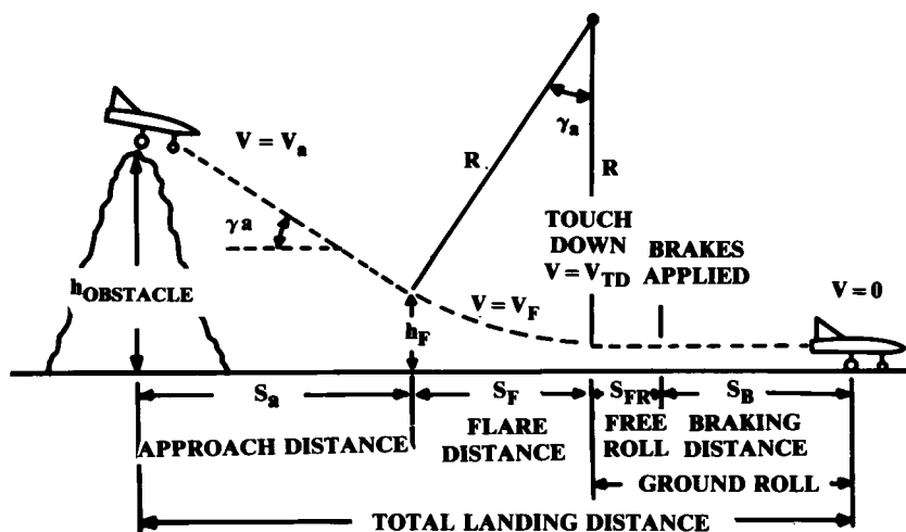
Fig. 17.18 Landing analysis.
