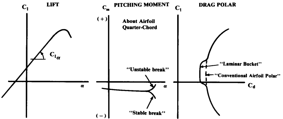
Fig. 4.5 Airfoil lift, drag, and pitching moment.
