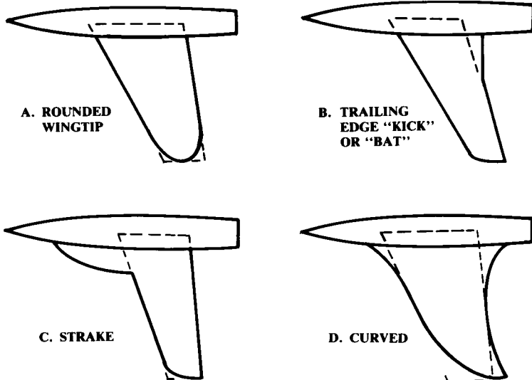
Fig. 7.24 Nontrapezoidal wings.
