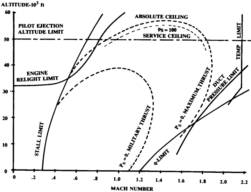
Fig. 17.16 Operating envelope.
