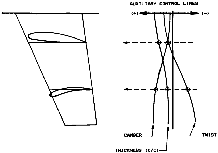
Fig. 7.27 Wing airfoil layout—nonlinear variations.
