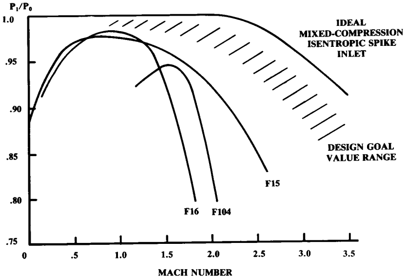
Fig. 13.4 Actual inlet pressure recoveries.
