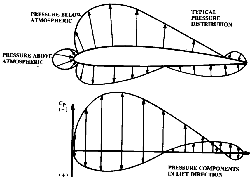
Fig. 4.2 Typical airfoil pressure distribution.
