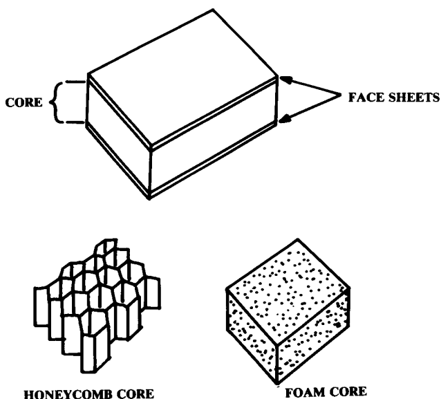
Fig. 14.29 Sandwich construction.
