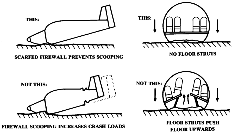
Fig. 8.15 Crashworthiness design.
