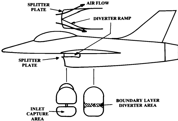
Fig. 10.19 Boundary layer diverter.
