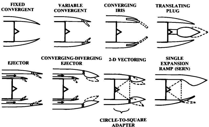
Fig. 10.20 Types of nozzles.
