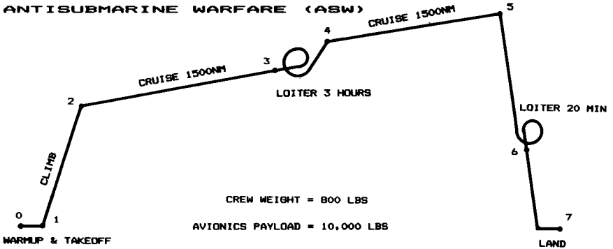
Fig. 3.8 Sample mission profile.
