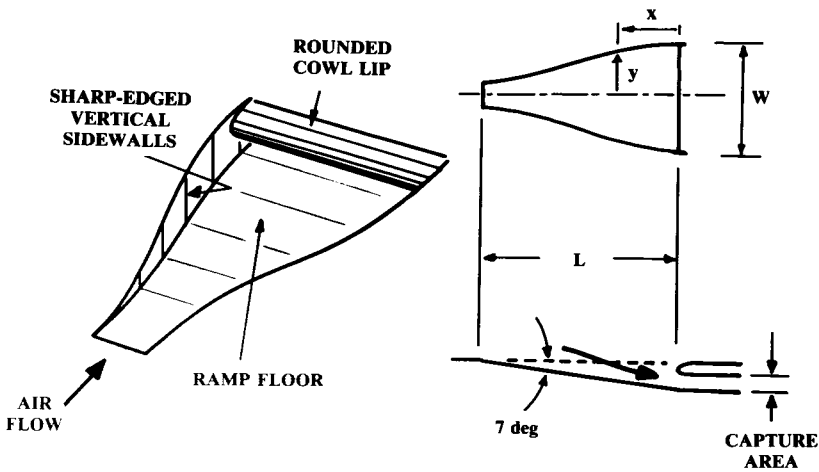
Fig. 10.5 Flush inlet geometry.
