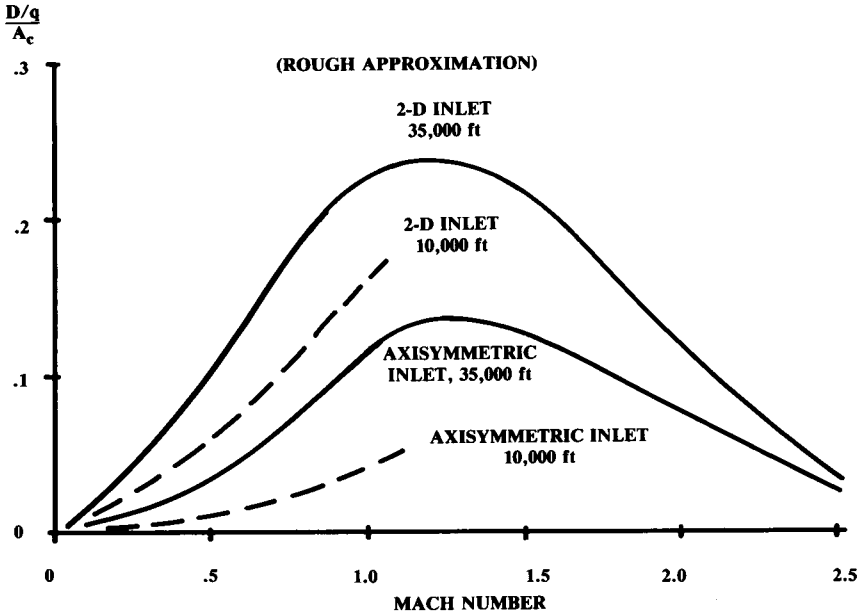
Fig. 13.6 Inlet drag trends.
