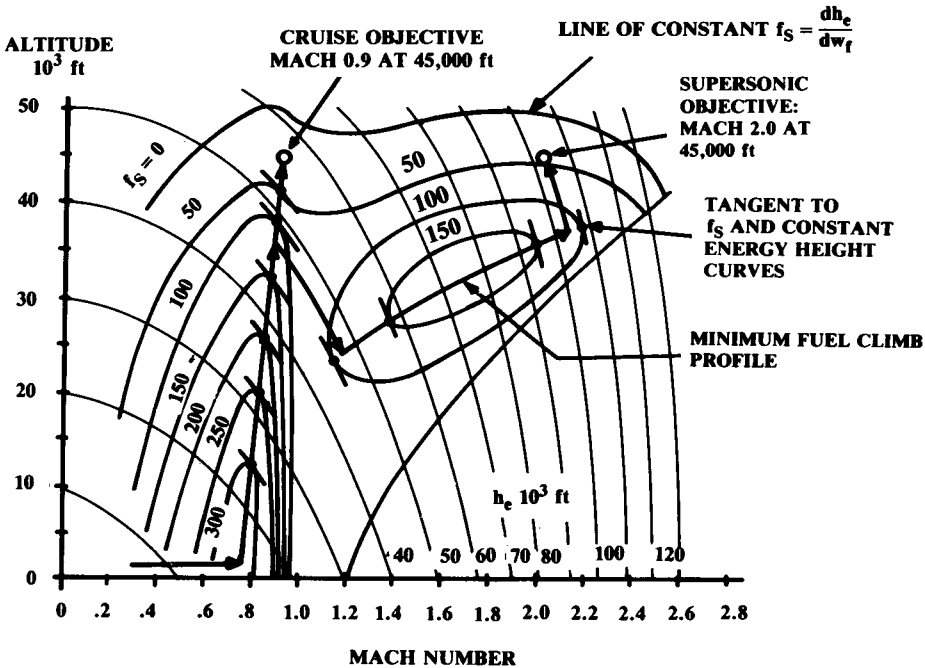
Fig. 17.15 Minimum fuel to climb.
