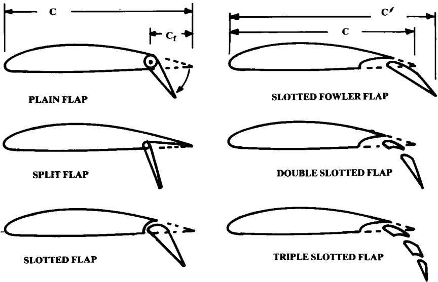
Fig. 12.16 Flap types.
