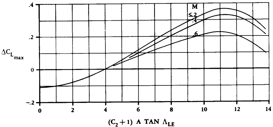
Fig. 12.13 Maximum-lift increment for low-aspect-ratio wings. (Ref. 37)
