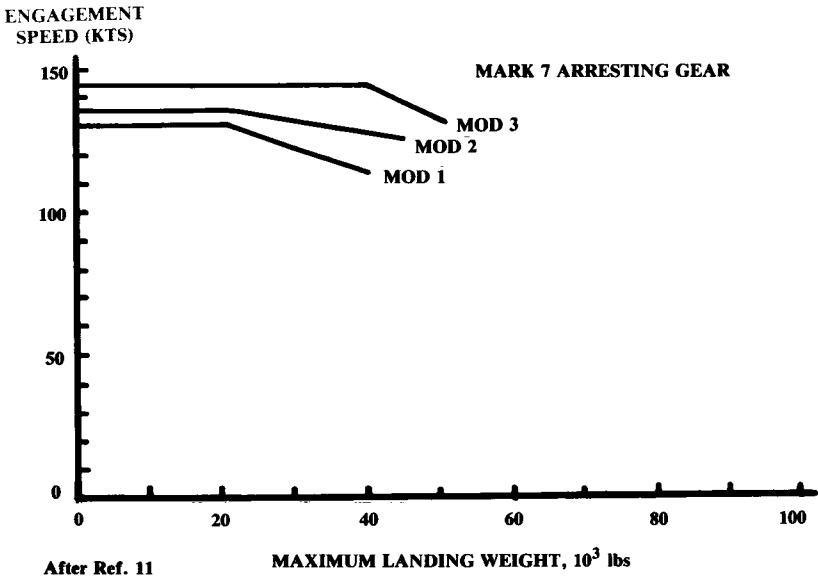
Fig. 5.6 Arresting gear weight limits.
