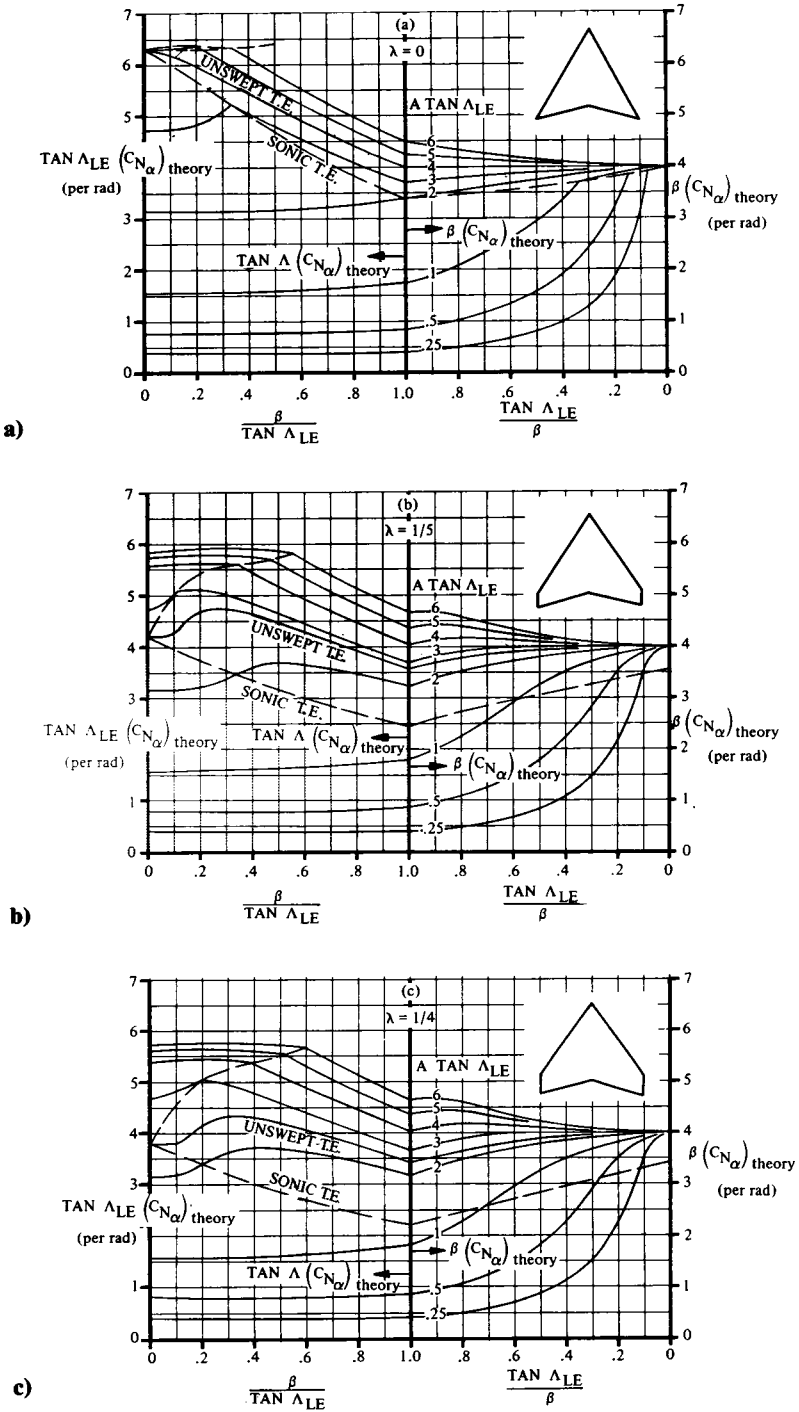
Fig. 12.6 Wing supersonic normal-force-curve slope. (Ref. 37)
