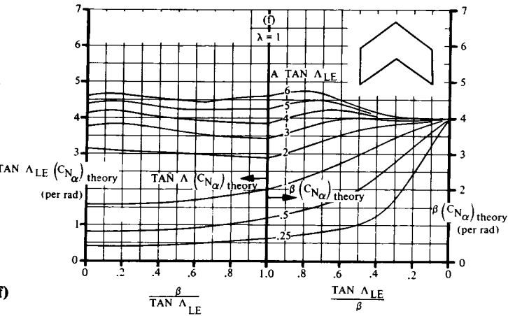
Fig. 12.6 (cont'd.) Wing supersonic normal-force-curve slope. (Ref. 37)
