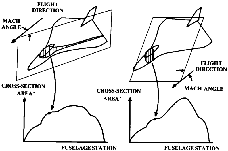
Fig. 12.25 Mach-plane cut volume distribution (two roll angles).
