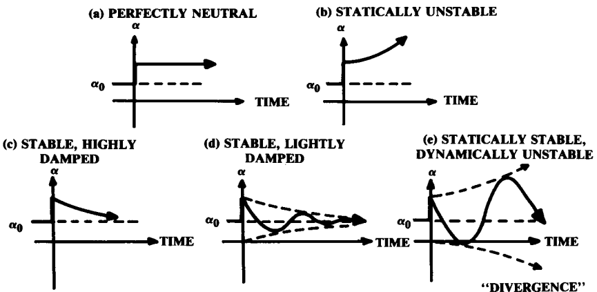
Fig. 16.1 Static and dynamic stability.
