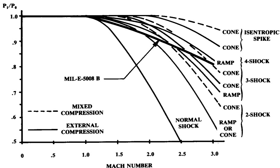
Fig. 13.3 Reference and available inlet pressure recovery.
