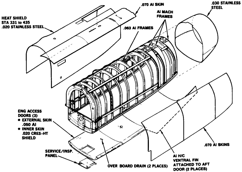
Fig. 14.24 Material selection—aft fuselage.
