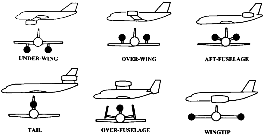
Fig. 10.12 Inlet locations—podded engines.
