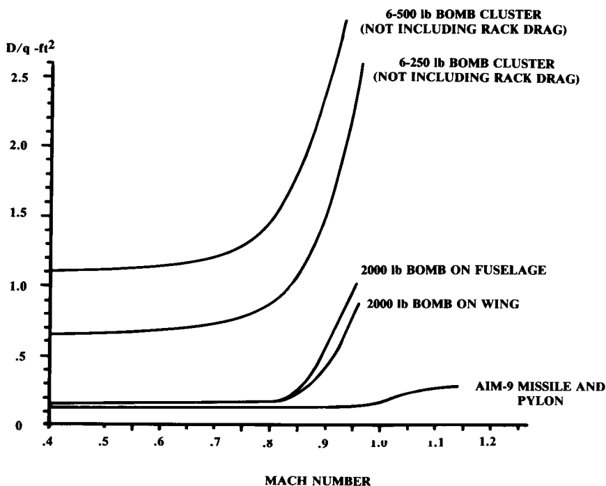
Fig. 12.22 Bomb and missile drag.
