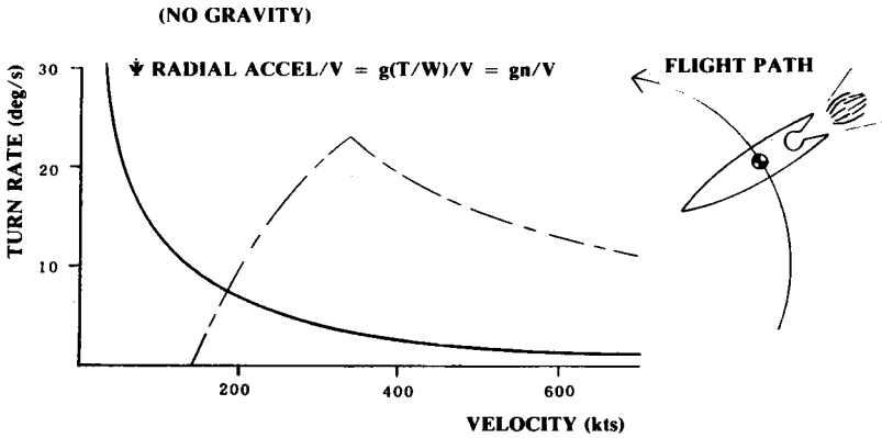
Fig. 17.21 Thrust-induced turning.
