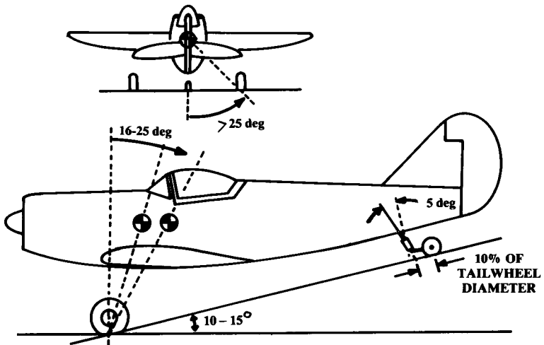
Fig. 11.3 Taildragger landing gear.
