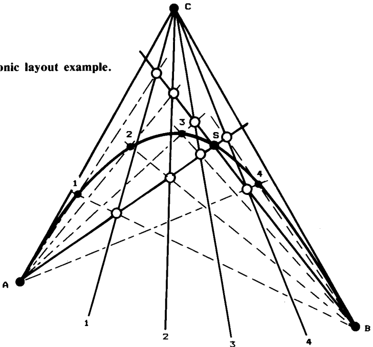
Fig. 7.11 Conic layout.
