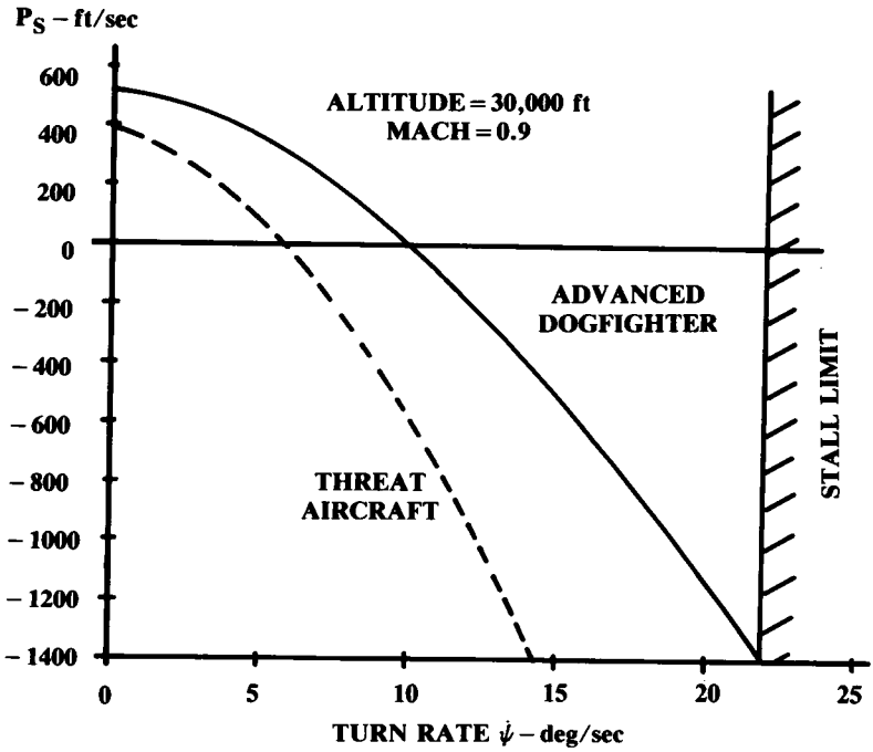
Fig. 17.9 Turn rate vs P_s .
