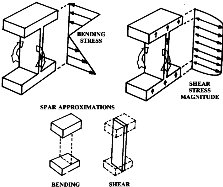
Fig. 14.41 Typical aircraft spar in bending and shear.
