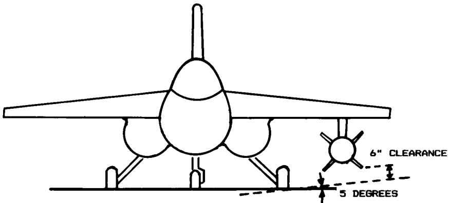
Fig. 4.25 Mid wing.
