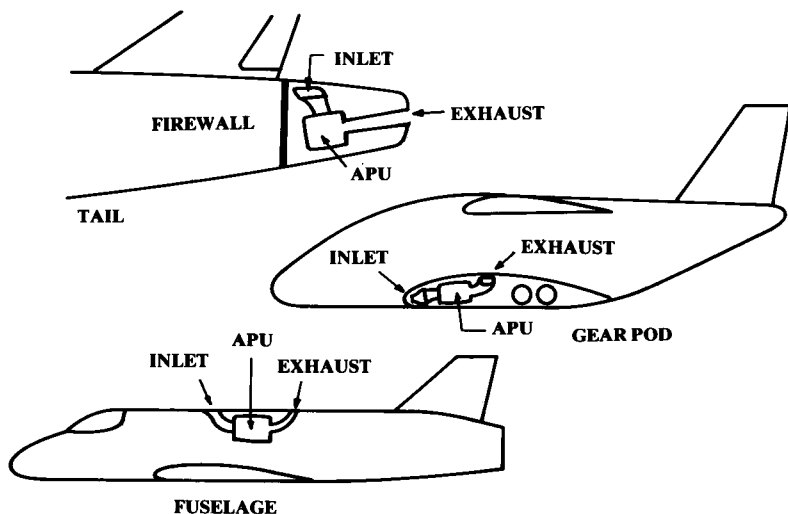
Fig. 11.17 APU installation.
