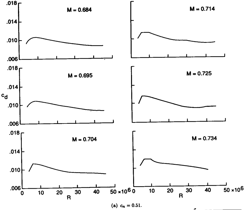
Figure 10. Profile-drag coefficient versus Reynolds number at various normal-force coefficients.
