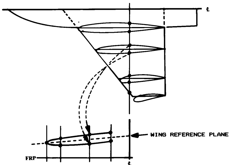
Fig. 7.31 Wing/tail cross section layout.
