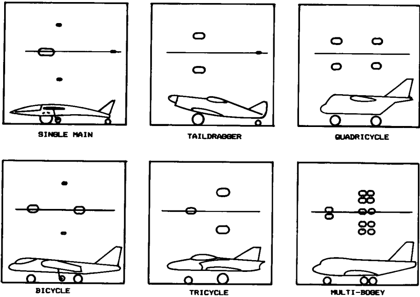
Fig. 11.1 Landing gear arrangements.
