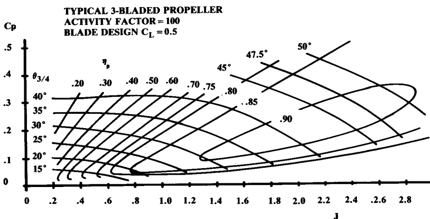
Fig. 13.9 Forward flight thrust and efficiency. (after Ref. 50)
