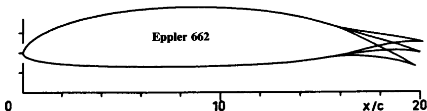
Eppler 662 - Flapped sailplane airfoil. (Ref. = NACA C.P. 2085)
