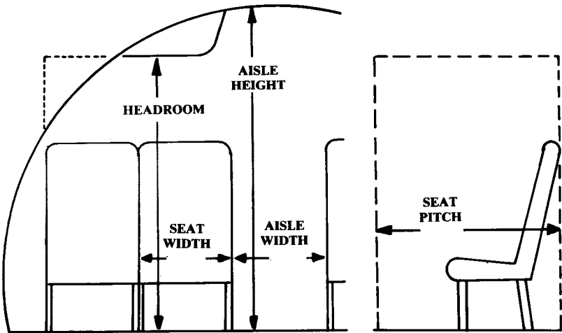
Fig. 9.3 Commercial passenger allowances.
