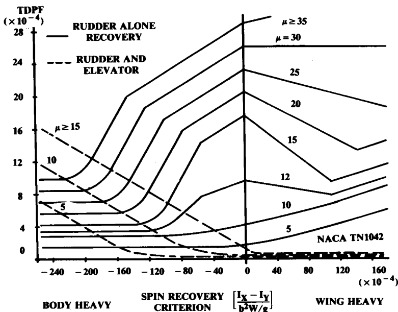
Fig. 16.31 Spin recovery criteria.
