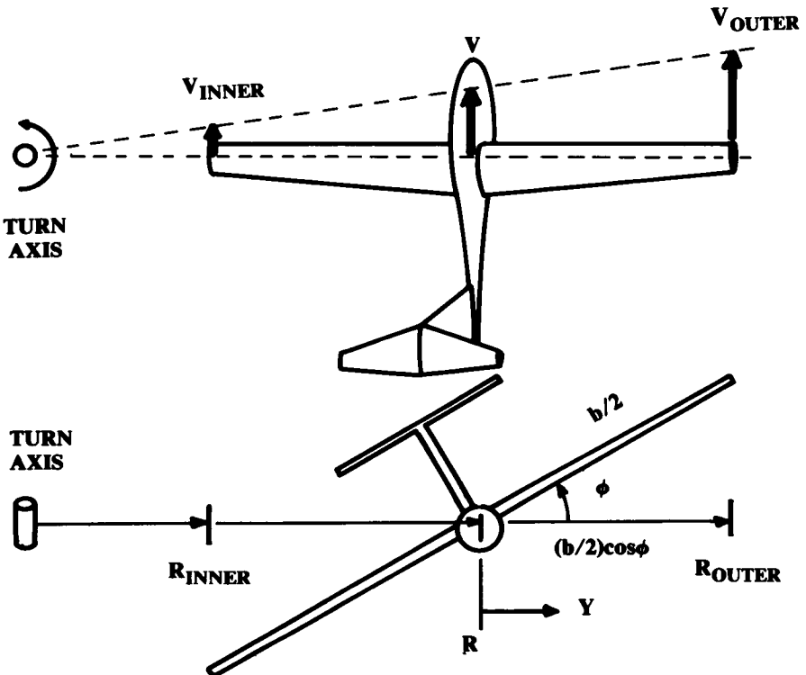
Fig. 17.7 Turn radius effect on wingtip velocity.
