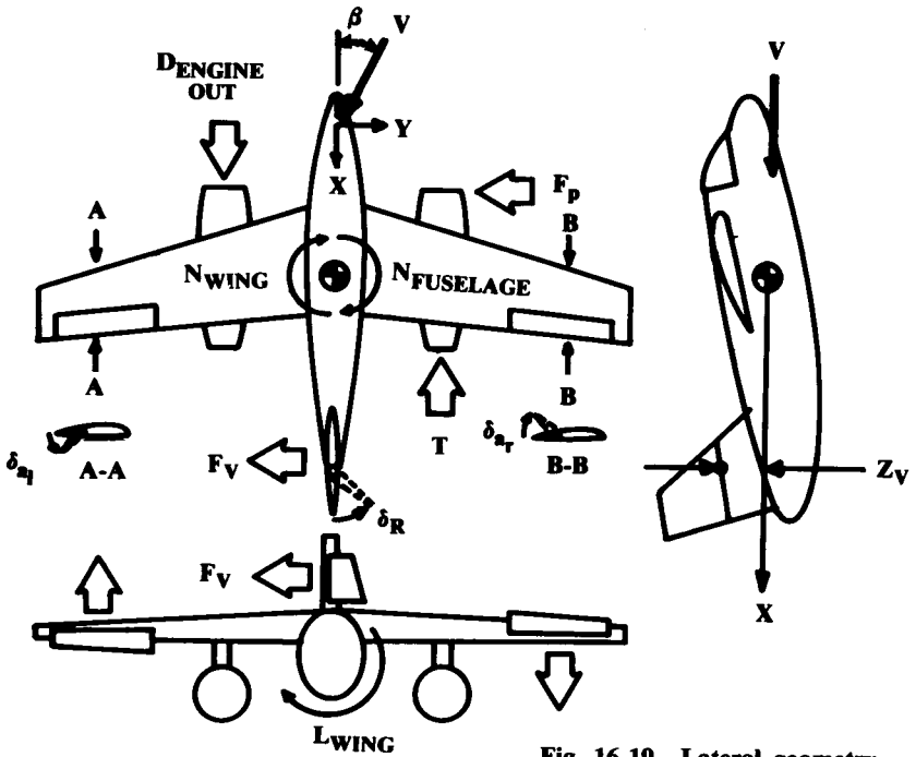
Fig. 16.19 Lateral geometry.
