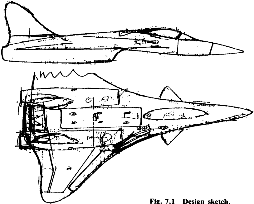
Fig. 7.1 Design sketch.
