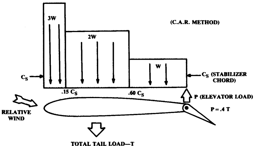
Fig. 14.14 Loads on fixed stabilizer with elevator deflection.
