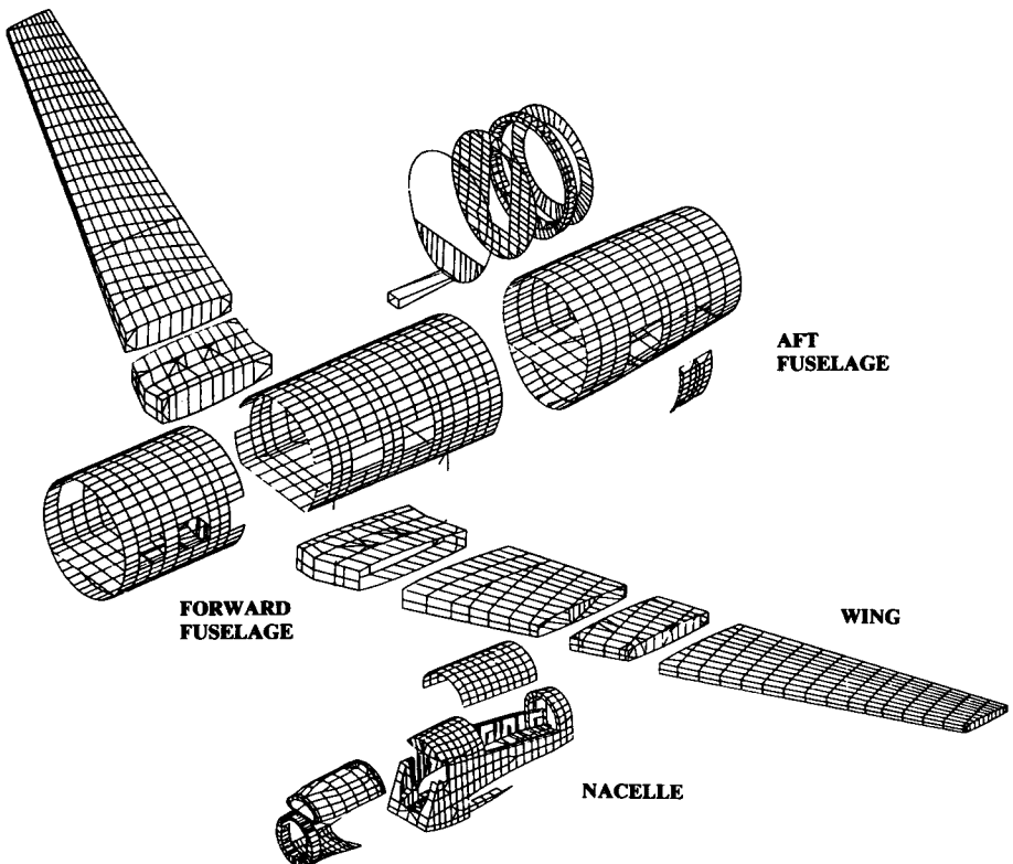
Fig. 14.46 Typical finite element model. (Courtesy Lockheed)
