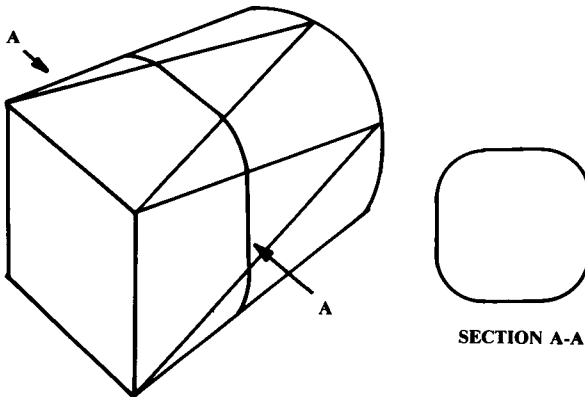
Fig. 7.20 Circle-to-square adapter.
