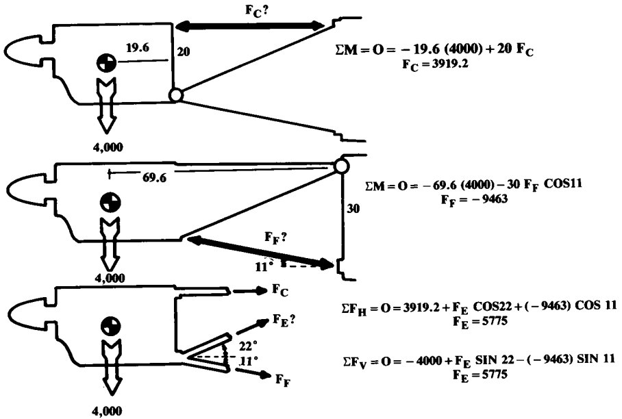
Fig. 14.36 Method of moments/method of shears.
