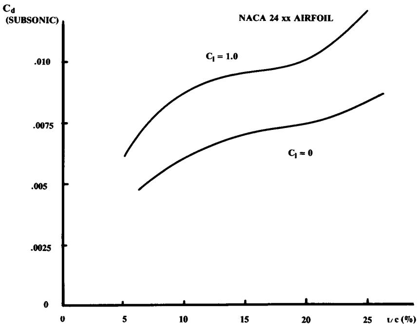
Fig. 4.11 Effects of t/c on drag.
