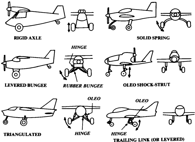
Fig. 11.8 Gear/shock arrangements.
