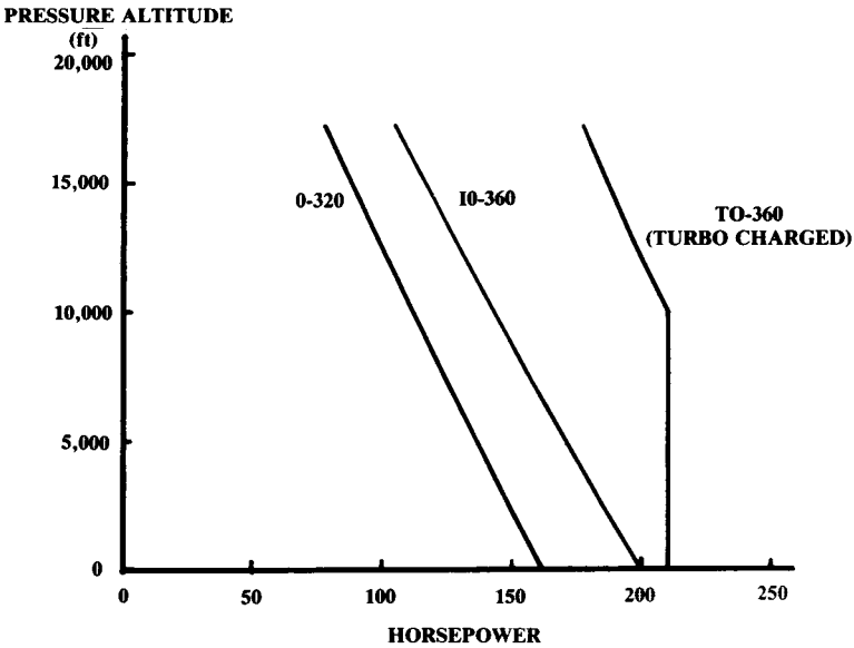
Fig. 5.2 Piston engine power variation with altitude.
