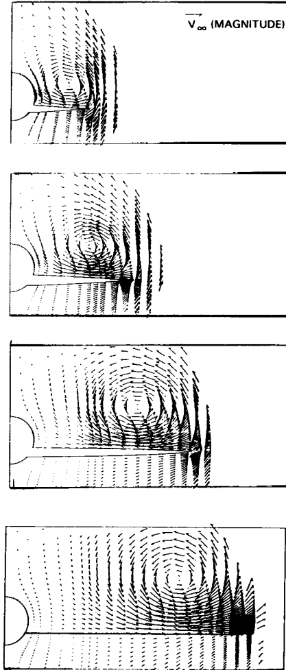
Fig. 12.39 Correlation of computed and measured cross-plate velocity fields; 75^\circ/62^\circ double-Delta wing body; M_\infty = 0.3 ; \alpha = 20^\circ . (Ref. 81)
