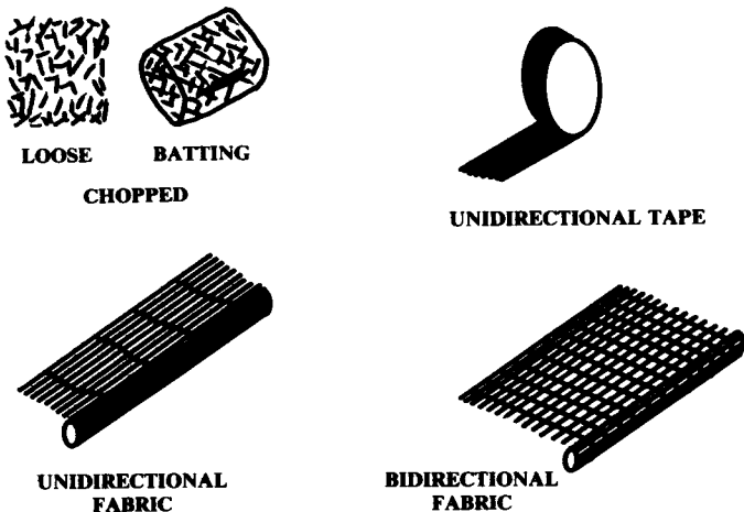
Fig. 14.28 Composite production forms.
