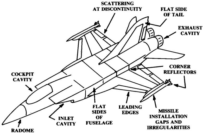
Fig. 8.10 Major RCS contributors.
