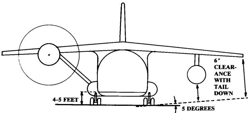
Fig. 4.24 High wing.
