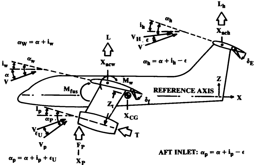
Fig. 16.3 Longitudinal moments.
