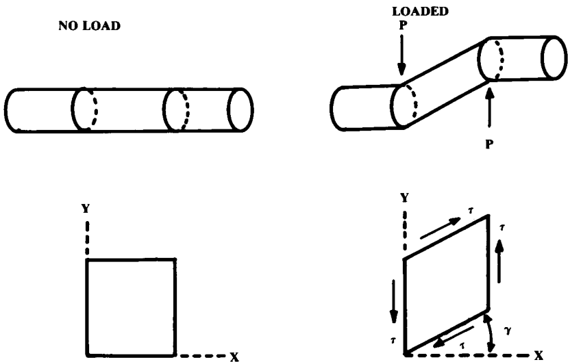
Fig. 14.20 Shear deformation.
