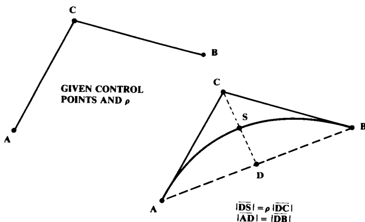
Fig. 7.16 Conic layout using \rho .
