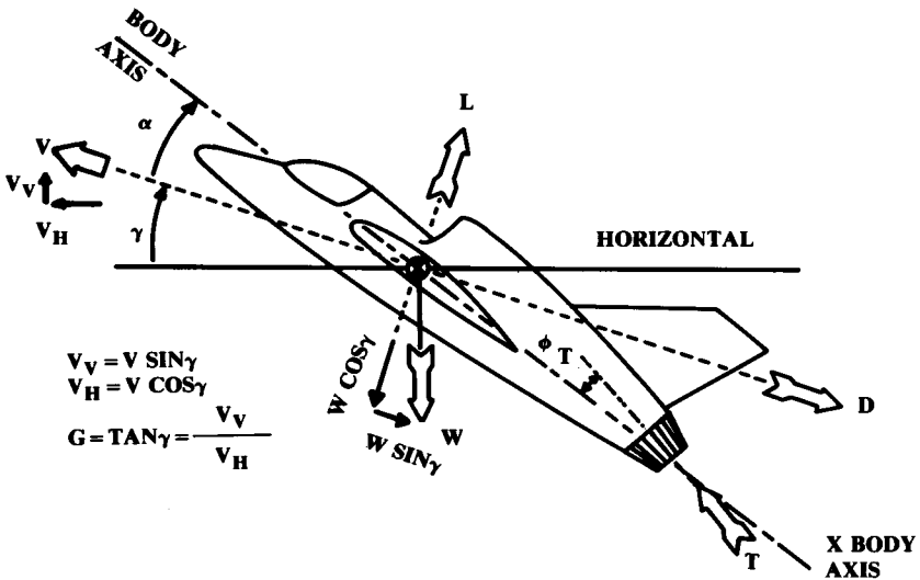
Fig. 17.1 Geometry for performance calculation.
