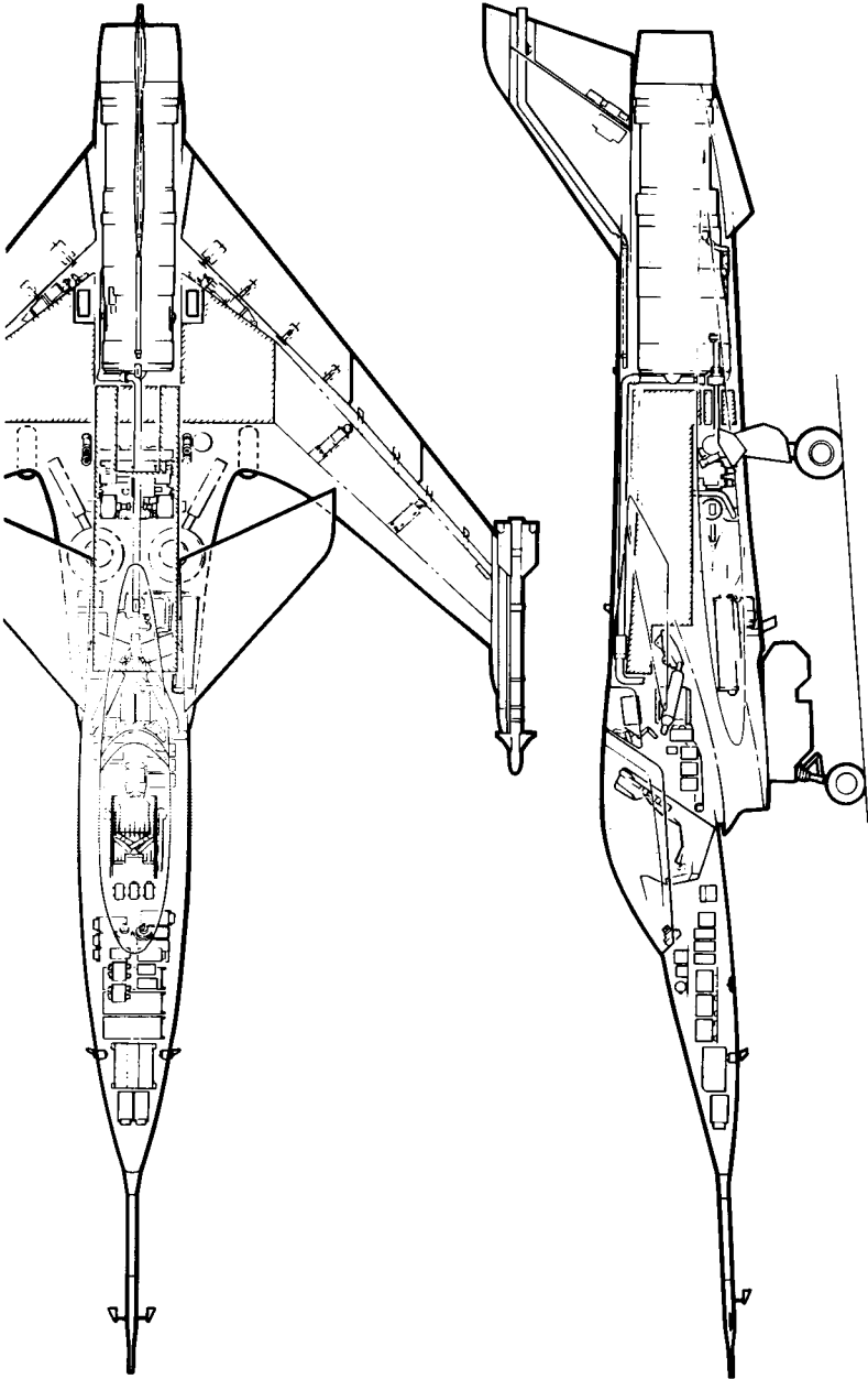
Fig. 7.6 FSX Inboard profile.
