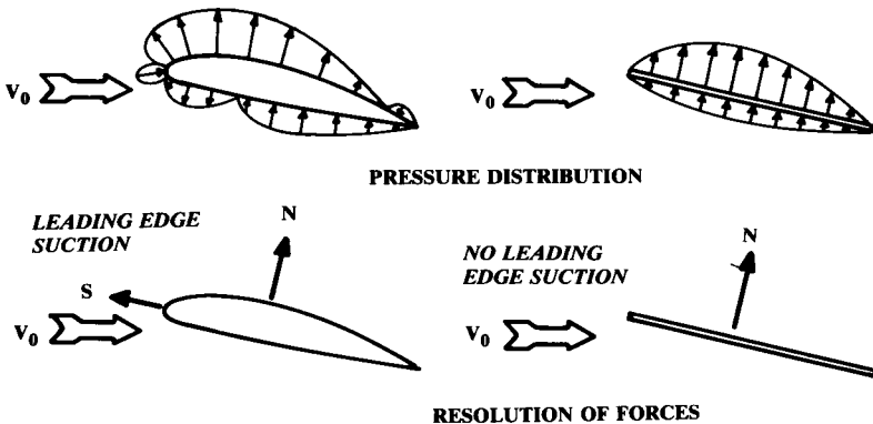
Fig. 12.33 Leading edge suction definition.
