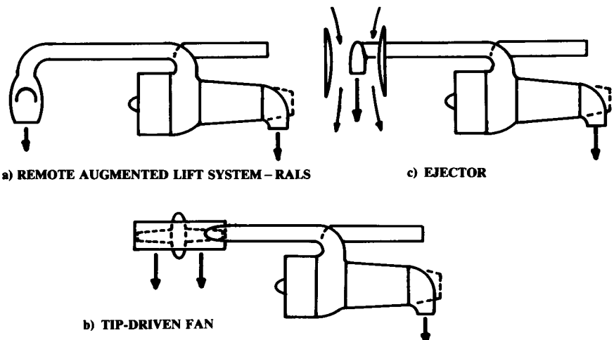
Fig. 20.7 Split flow engines (diverted fan air).
