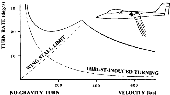
Fig. 17.22 Thrust vectoring at center of gravity.
