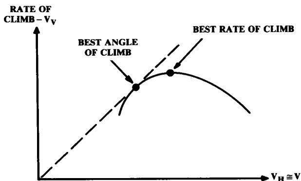
Fig. 17.3 Graphical method for best climb.
