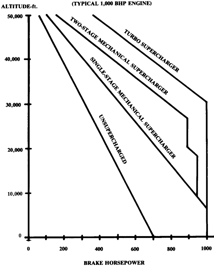
Fig. 13.7 Effects of supercharging.
