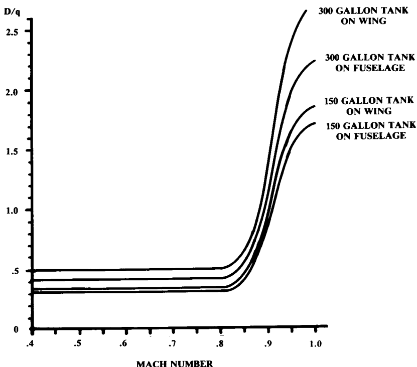
Fig. 12.21 External stores drag-fuel tanks.
