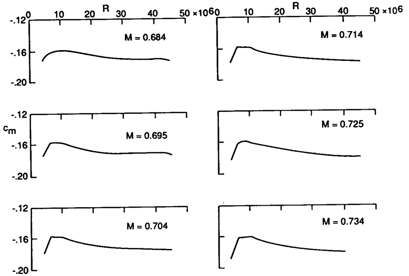
Figure 11. Quarter-chord pitching-moment coefficient versus Reynolds number at various normal-force coefficients
