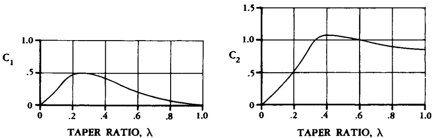
Fig. 12.11 Taper-ratio correction factors for low-aspect-ratio wings. (Ref. 37)
