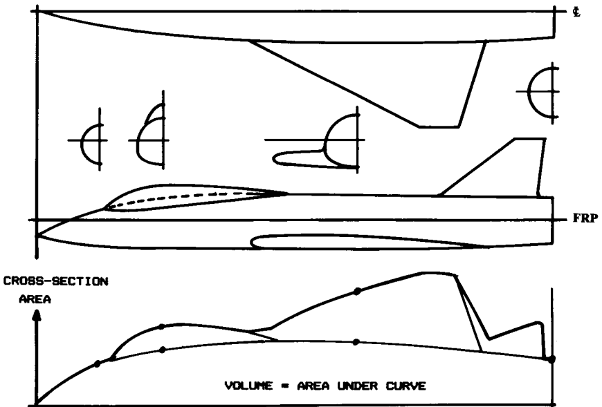
Fig. 7.36 Aircraft volume plot.
