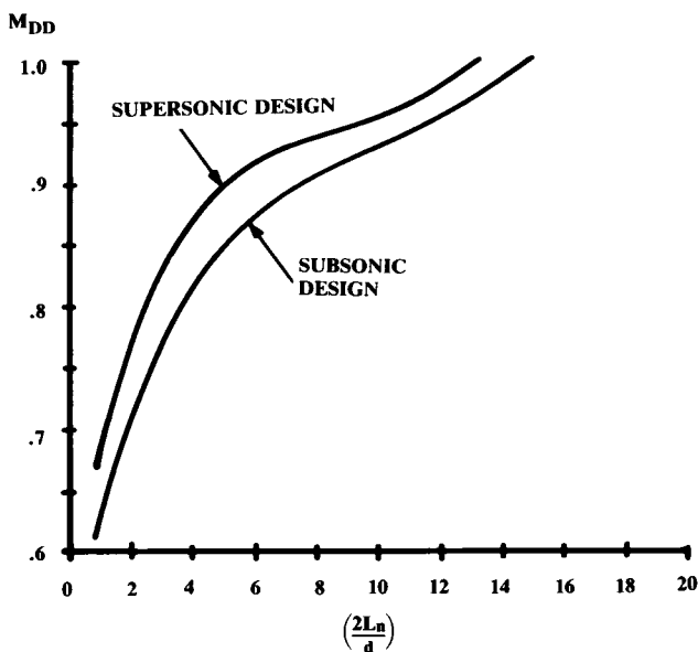
Fig. 12.28 Body drag-divergent Mach number.
