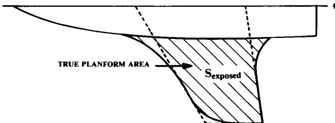
Fig. 7.33 Wing/tail wetted area estimate.
