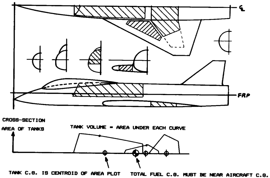
Fig. 10.23 Fuel tank volume plotting.
