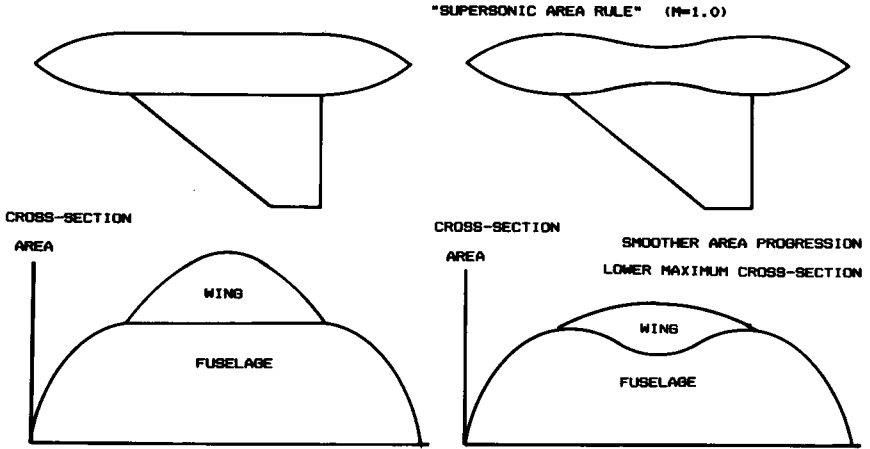
Fig. 8.3 Design for low wave drag.
