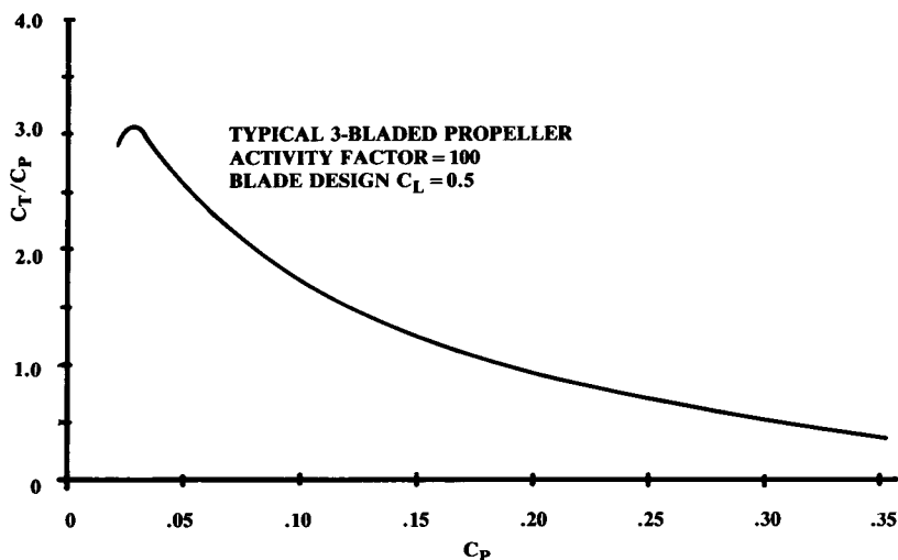
Fig. 13.8 Static propeller thrust. (after Ref. 50)
