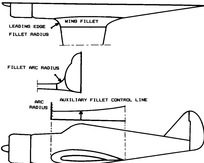
Fig. 7.32 Wing fillet layout.
