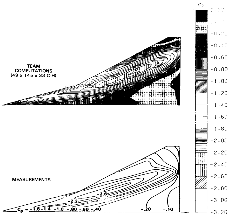
Fig. 12.38 Correlation of computed and measured surface pressure contours; 75^\circ/62^\circ double-Delta wing body; M_\infty = 0.3 ; \alpha = 20^\circ . (Ref. 81)
