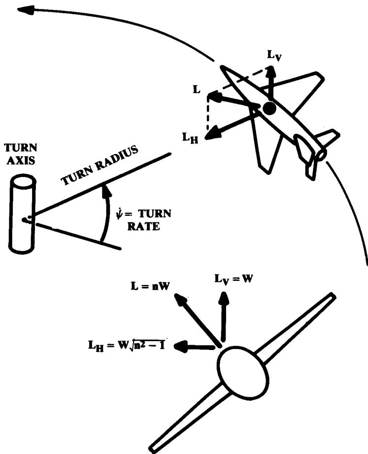
Fig. 17.4 Level turn geometry.
