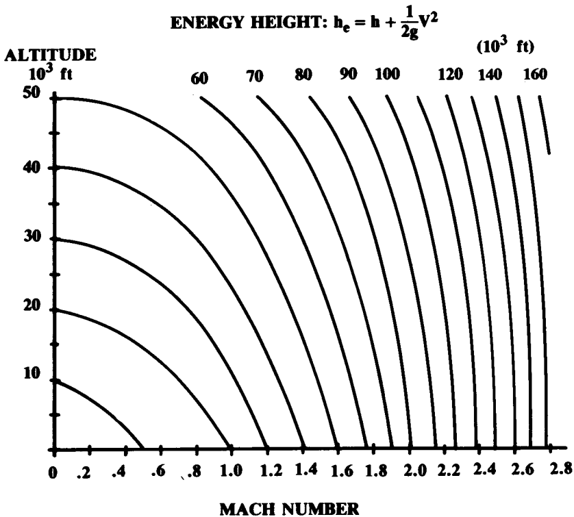
Fig. 17.12 Lines of constant energy height.
