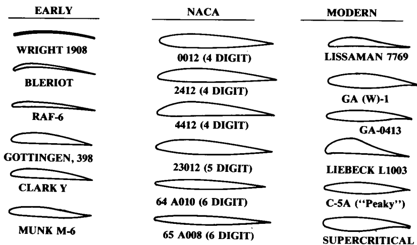
Fig. 4.6 Typical airfoils.
