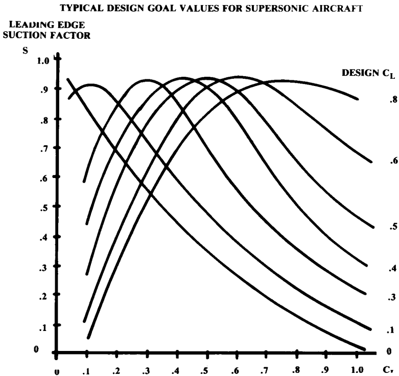
Fig. 12.35 Leading edge suction vs C_L .
