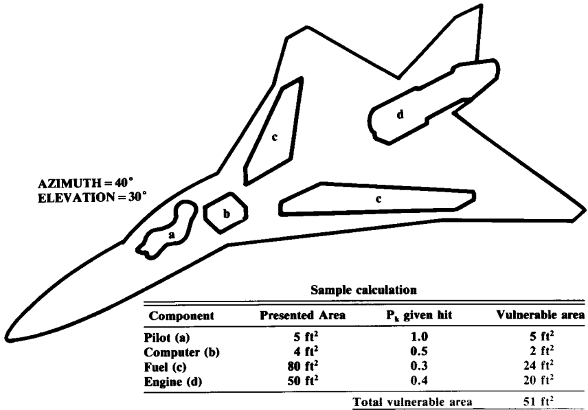
Fig. 8.14 Vulnerable area calculation.
