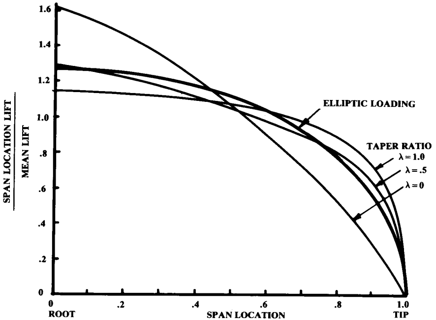
Fig. 4.22 Effect of taper on lift distribution.
