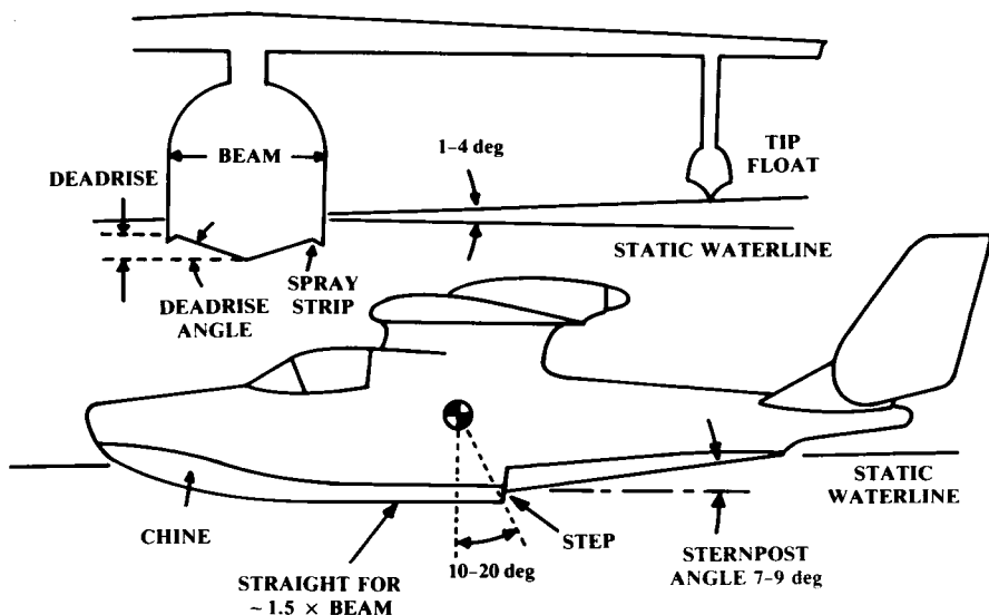
Fig. 11.15 Seaplane geometry.
