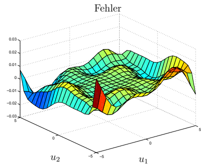
Abb. 3.62: \mathcal{NL}(u) - \widehat{\mathcal{NL}}(u)
