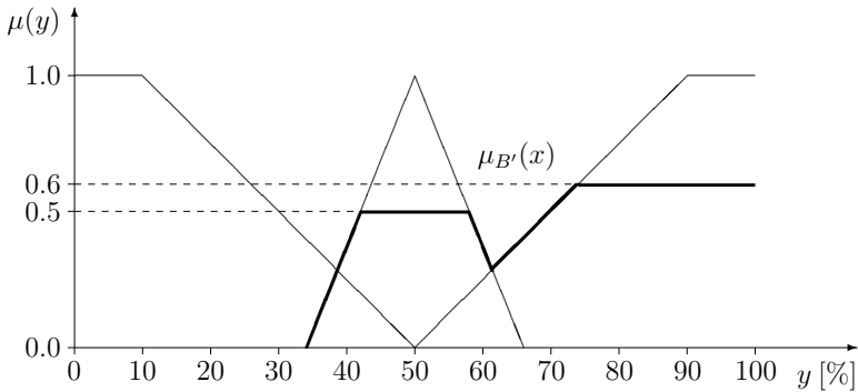
Abb. 18.39: Clipping
