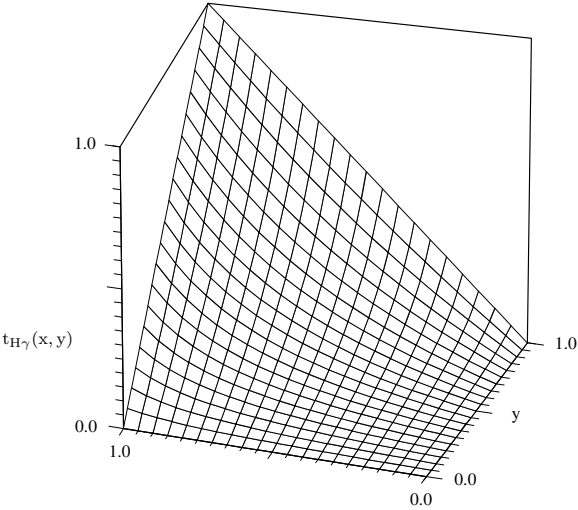
Abb. 18.28: Hamacher-Durchschnittsoperator, \gamma = 5,0
