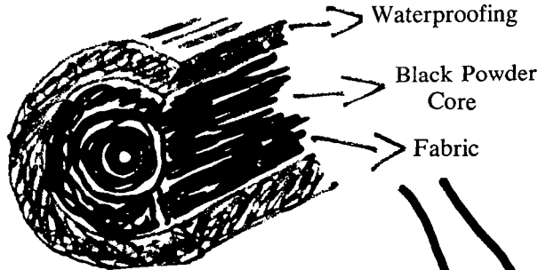
Figure 73. Safety fuse.
