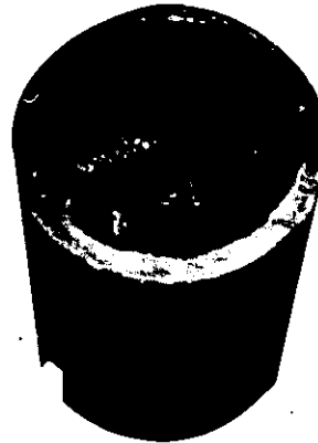
Place completed washer in breech piece (locked to barrel), with tin spacer separating washer and a round in the chamber. Weld washer fast to breech piece, maintaining headspace established by the empty round and tin spacer.
