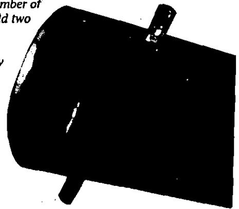
Completed M203 barrel with locking studs welded in place (left).
