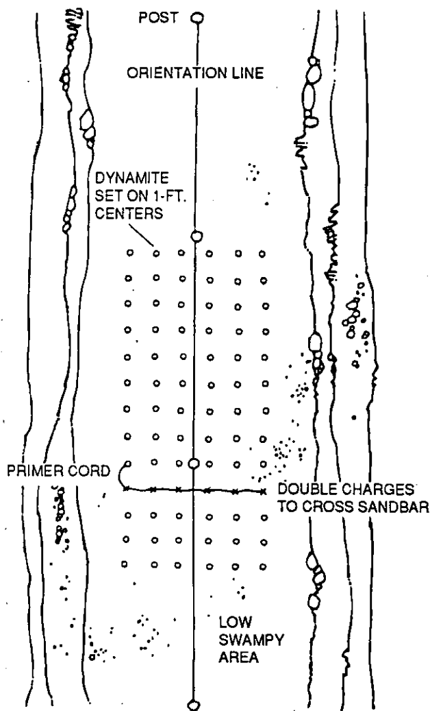
Top view of a ditching grid.
