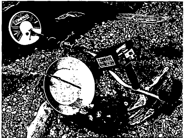
Sophisticated modern metal detectors like the Compass Scanner can be used under extremely difficult circumstances and can automatically retune themselves for varying ground conditions and earth composition. (Photo courtesy of Compass Electronics.)
