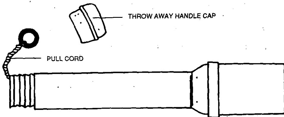
German World War II stick grenade.
