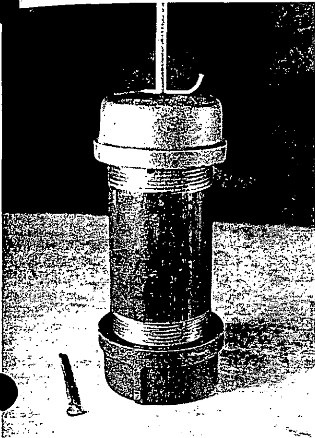
Firing-pin assembly cocked and retained with a small pin. Note the nail used as safety taken from hole in the grenade body, lying next to the grenade.
