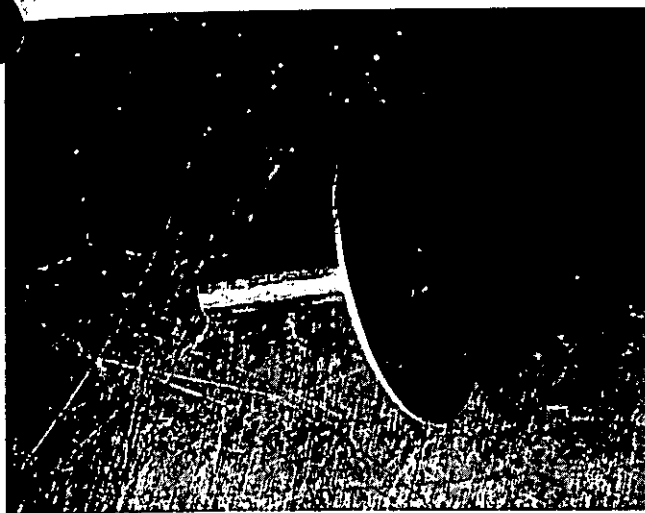
Prepare a pull-pin fuze by gluing or welding a 1/8-inch pipe nipple into the center of a 1/2-inch fender washer.
