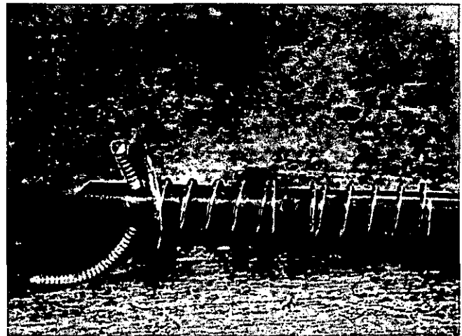
Sharpen the end of a 4-inch long, 1/4-inch bolt and drill a 1/16-inch hole through the bolt about 1/2 inch ahead of the sharpened tip through which a pin is inserted. This pin becomes the retainers for a flat washer against which a 3/8-inch compression spring bears, and a second 1/16-inch hole farther up the shaft acts as the striker retainer hole.
