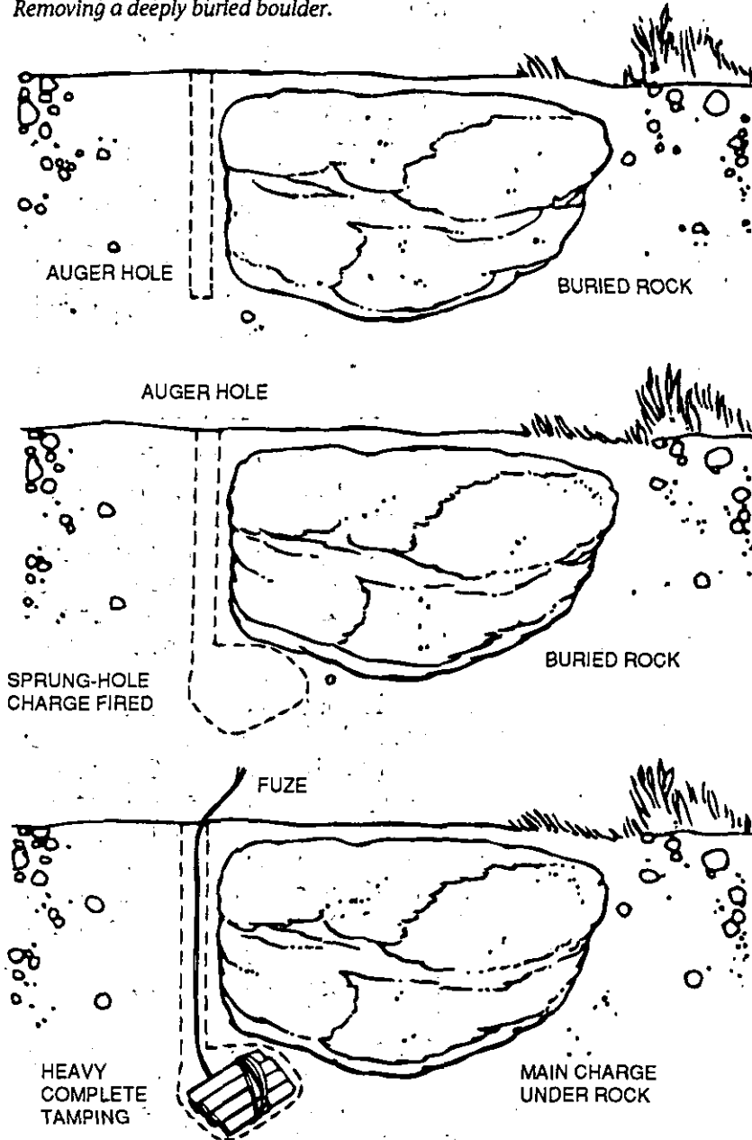
Removing a deeply buried boulder.
