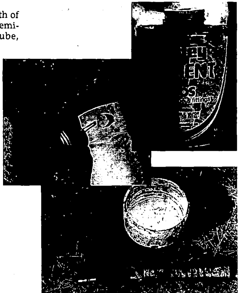
Top Left: Permanently glue the lower cap on the cache tube using ABS cement purchased from a plumbing supply house. Top Right: ABS cement used to attach caps to cache tubes. Bottom: Eight-inch slip-type cap for cache tube with grease gun used to attach cap.
