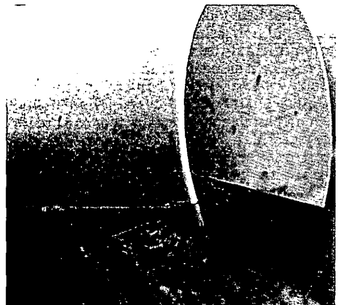
Using a common hand saw, cut straight down from the marks, producing three almost equal 9- x 10-inch slabs of PVC pipe.
