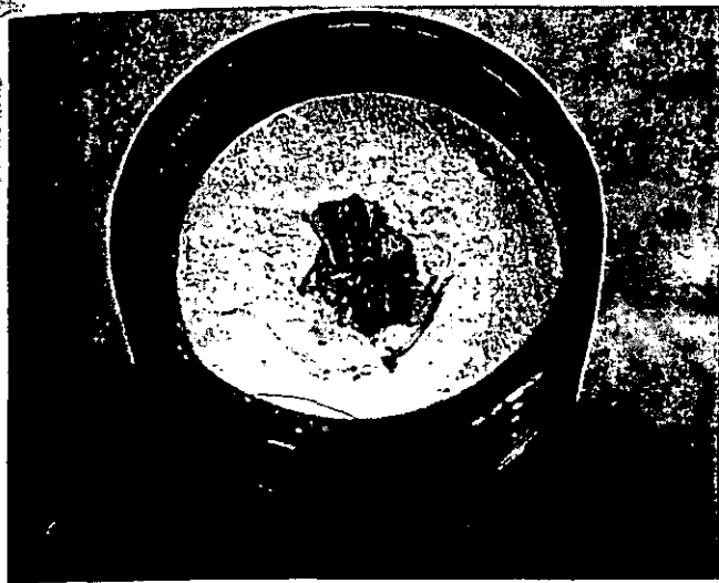
A standard 12-second piece of dynamite fuze glued to a 1/2-inch fender washer. A match head is placed in the center of the split fuze and the entire assembly anchored solidly 1 inch into the base of the projectile body. Explosives are packed in behind the washer as an added deterrent to the assembly's moving when the round is fired. Heat from the blank shell lights the match head and fuze.
