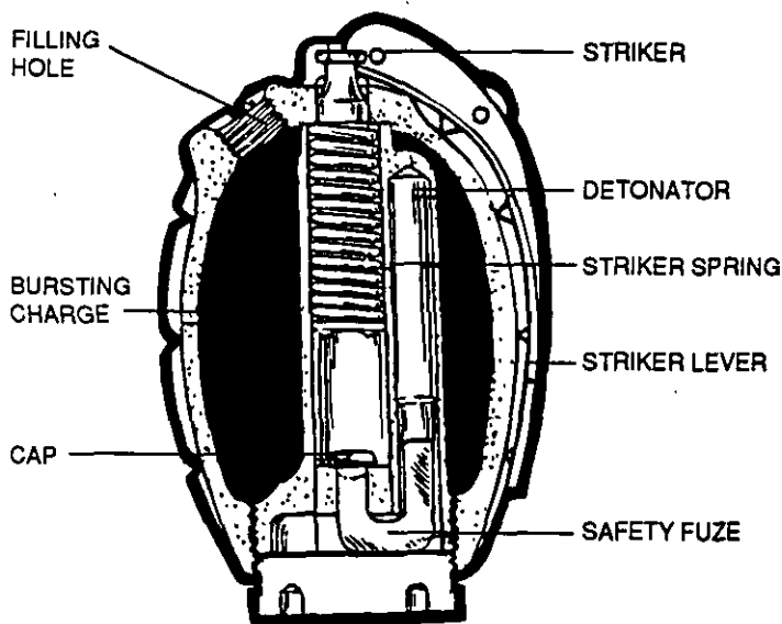
Developed in 1915, the Mills number 5 hand grenade, better known as the Mills bomb, was the first modern British grenade.
