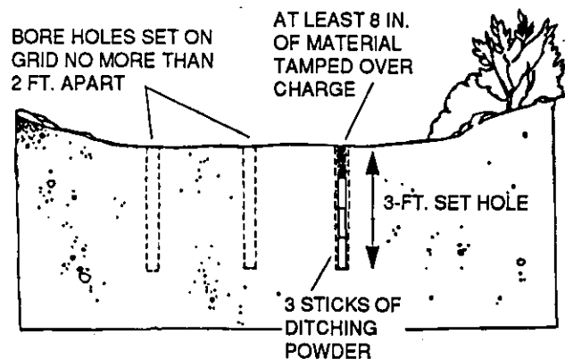
Side view of ditching set.
