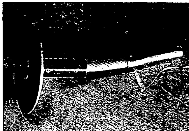
A fuze segment with cap attached pushed snugly up into a 1/8-inch pipe nipple with shot shell primer in place ready for insertion in the grenade body.
