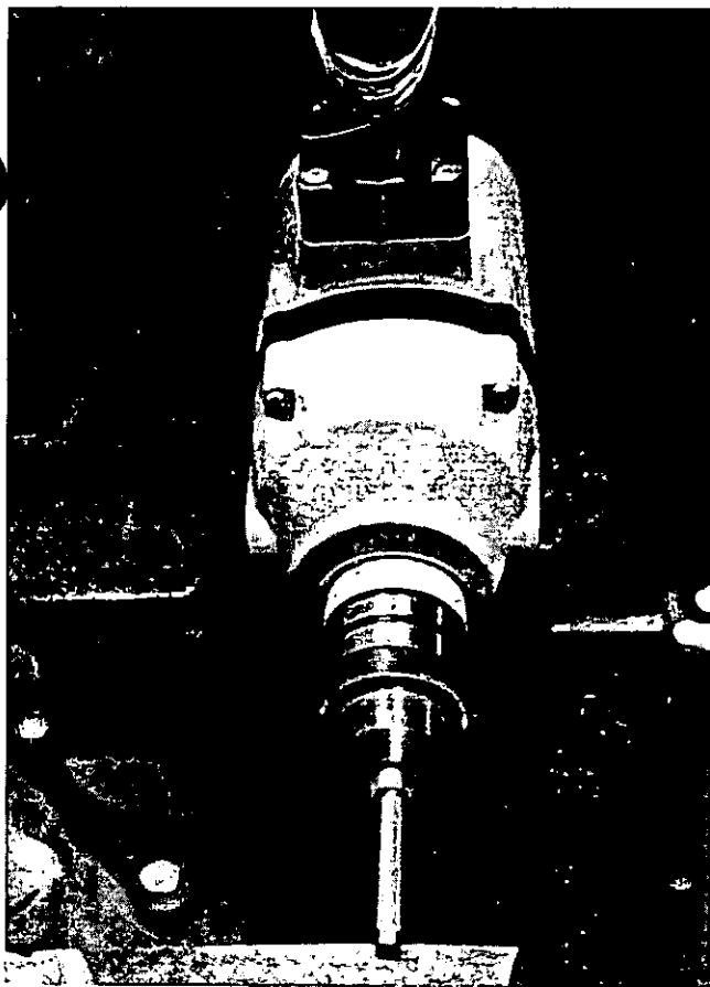
Wrap tape around bolt threads and chuck into fastened-down 1/2" drill. Work the end down to 1/16" for the firing pin.
