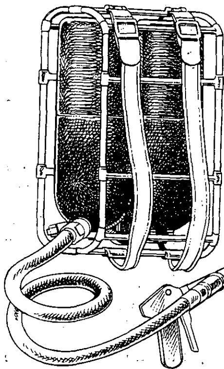
M9E1-7 portable flamethrower (U.S.).
