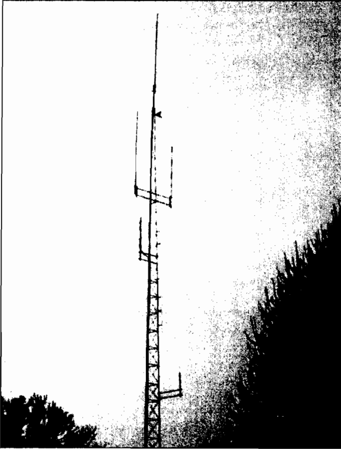
Typical public safety base antenna system Note that all antennas are vertically polarized
