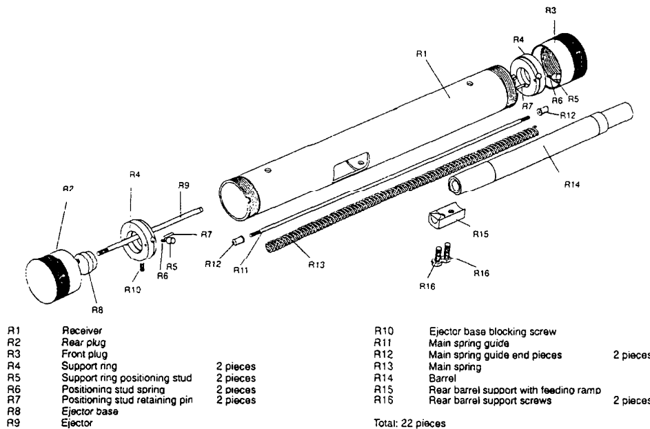
Receiver with barrel and main spring.
