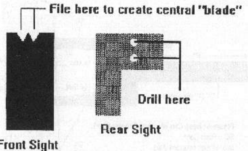
Figure 5: Front and Rear Sight Detail.
