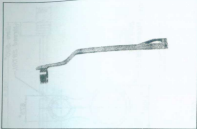
Combination carrying handle/operating handle guide, side view.
