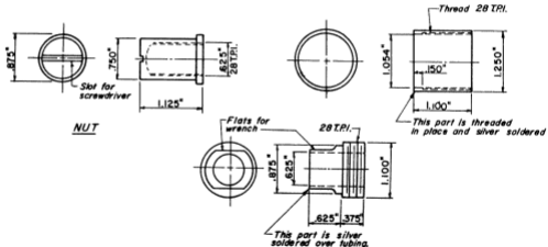
STOCK MOUNTING BRACKET AND NUT
