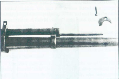
Forend can also be held in place using system shown here. Method shown on plan is stronger, simpler, neater.
