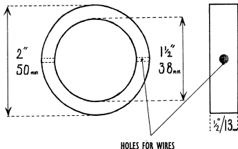
Igniter housing.
