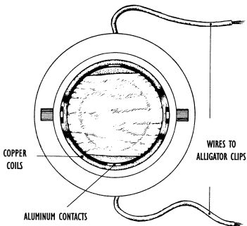
Top view of cartridge with completed igniter in place.
