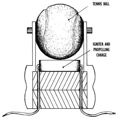
Cross-section of completed cartridge.
