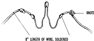
Estes igniter.
