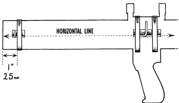
Position of open sights.
