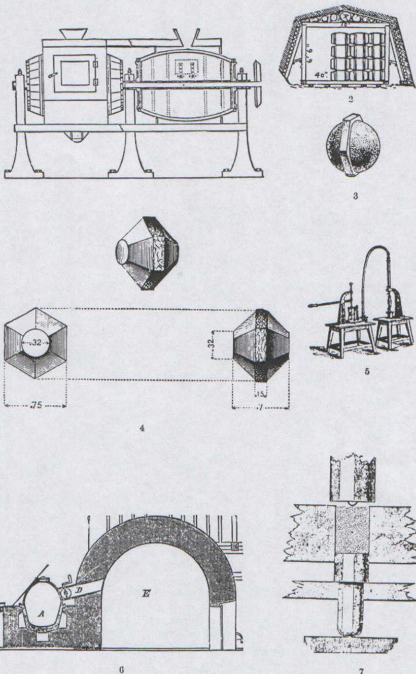
GUNPOWDER. —1, Glazing Apparatus. 2, Storage of Gunpowder in Magazine. 3, Spherohexagonal Powder. 4, Hexagonal Powder. 5, Densimeter. 6, Sulphur Refining Apparatus. 7, Special Powder Machine.
