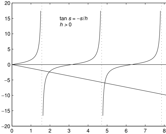
Figure 6.2 The graphical solution of (6.79).
