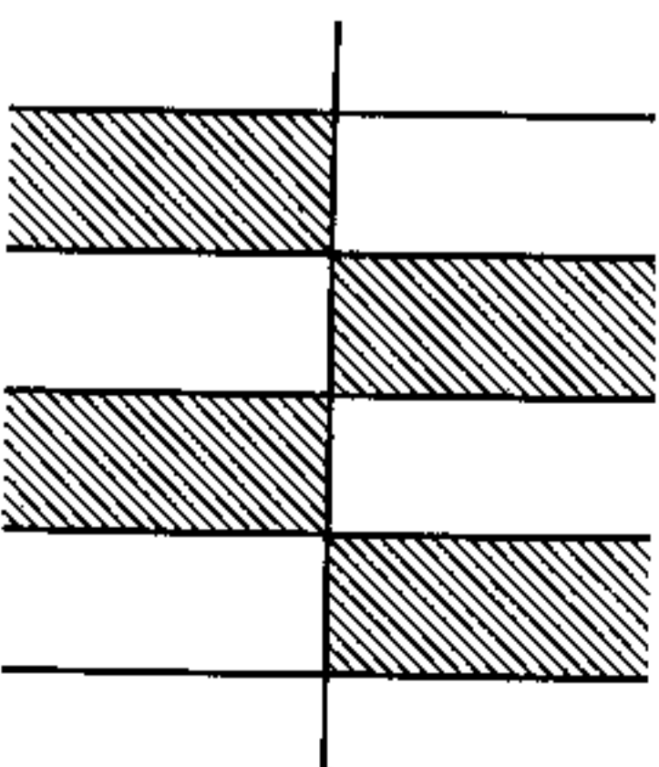
FIG. 3-11. Fundamental regions of \cos z .
