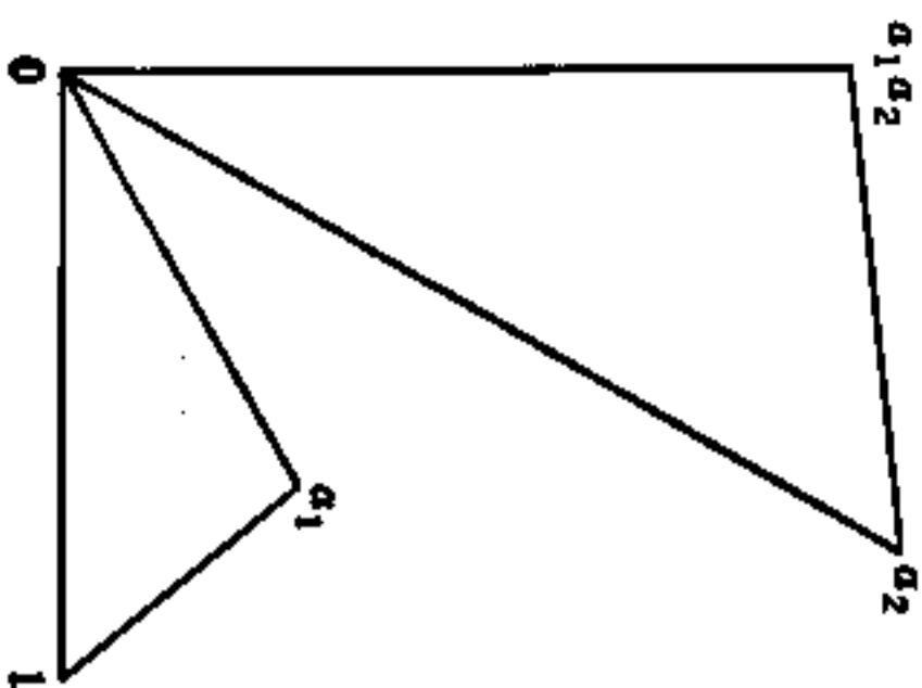
FIG. 1-2. Vector multiplication.
