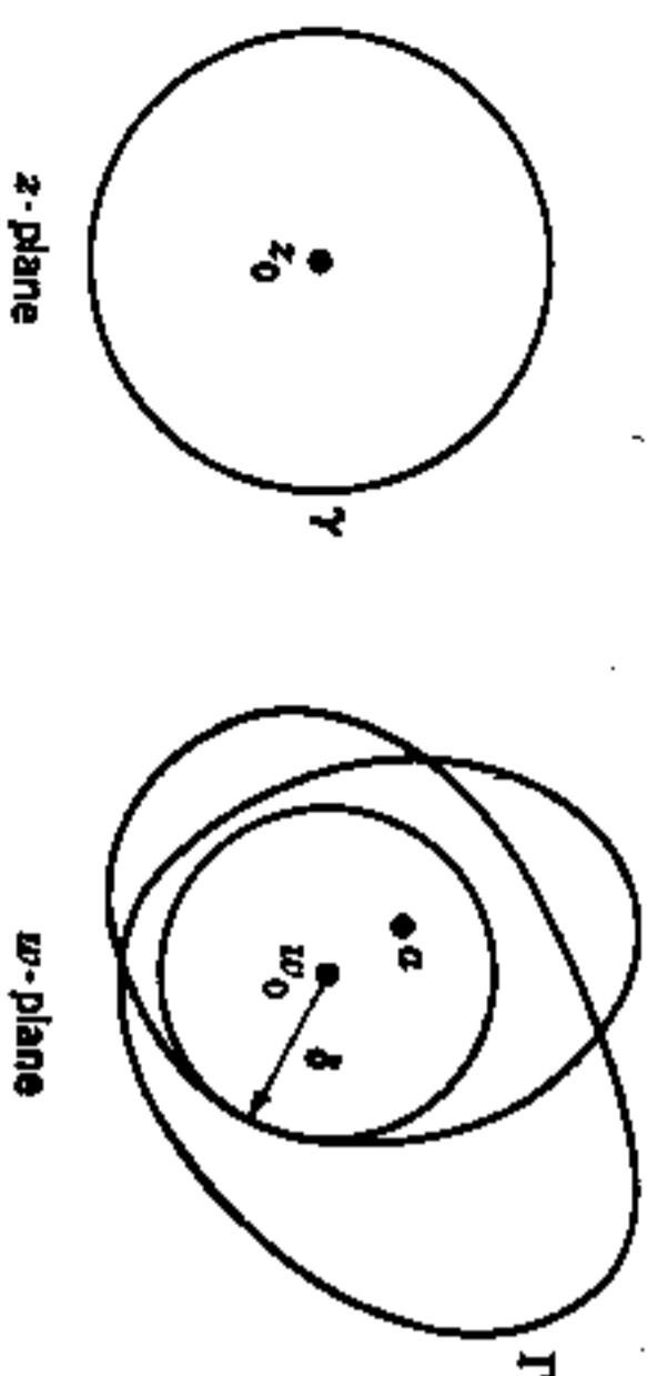
FIG. 4-7. Local correspondence.
