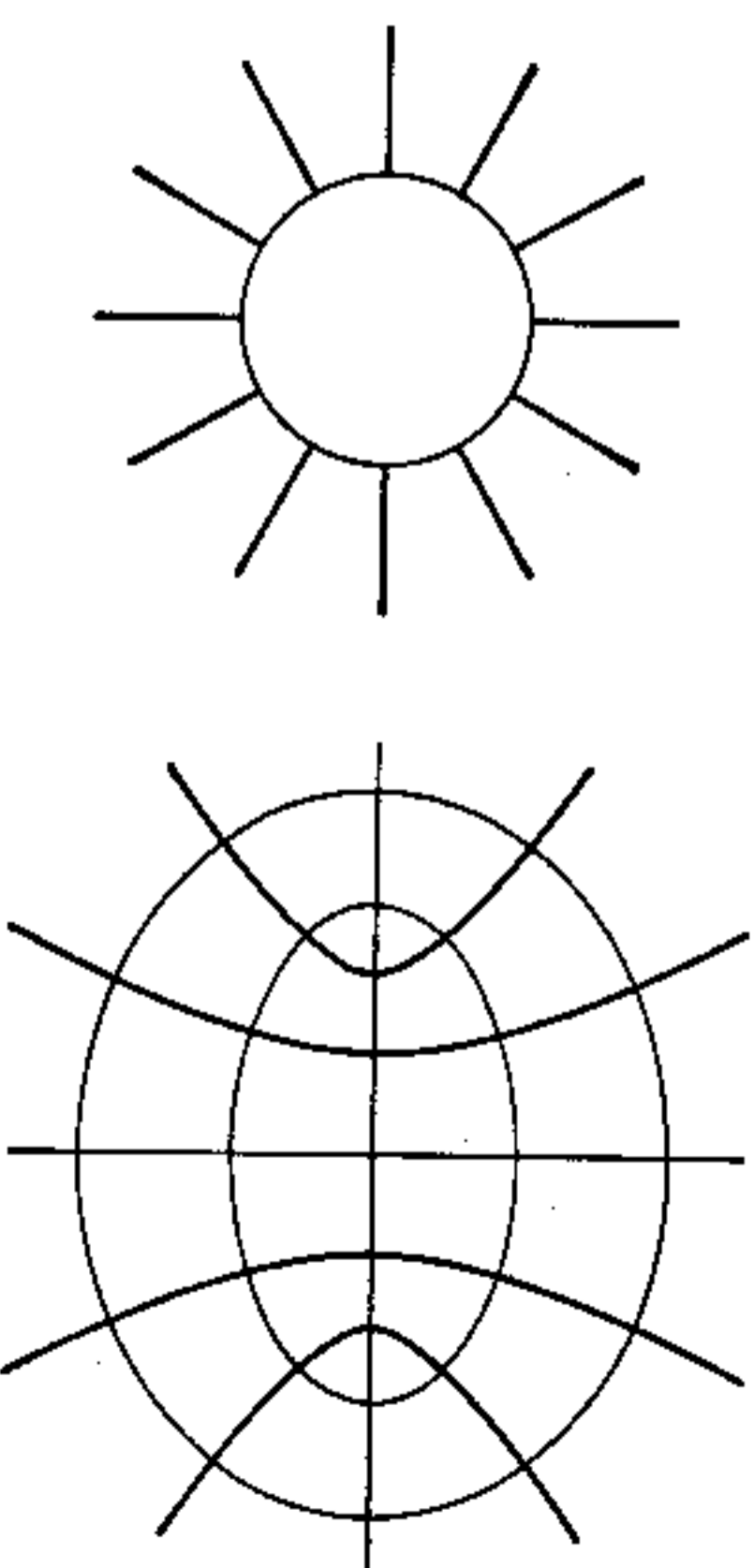
FIG. 3-9. Mapping by z = \frac{1}{2}(w + w^{-1}) .
