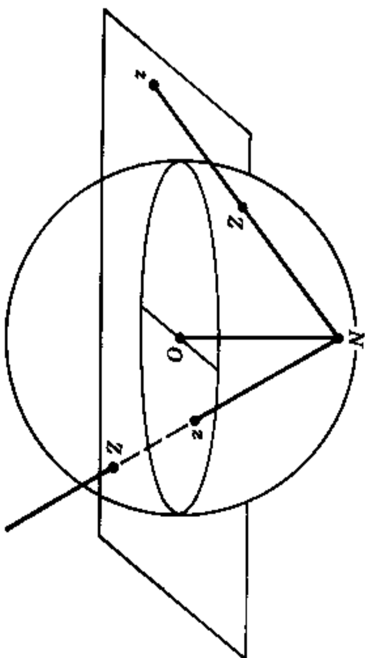
FIG. 1-3. Stereographic projection.
